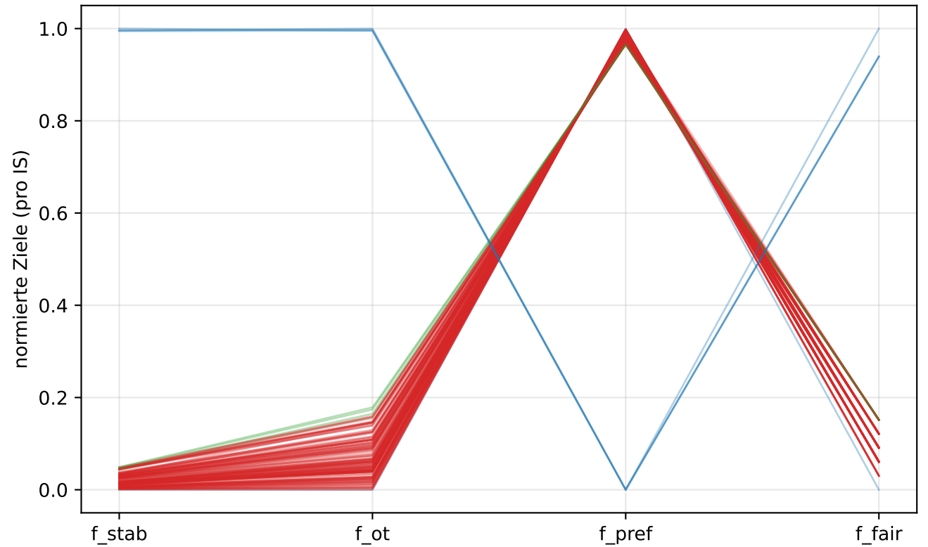
Parallel Coordinates (P*): praxisnah_v1/sc-large__av-tight__dp-weekday_high__sev-
