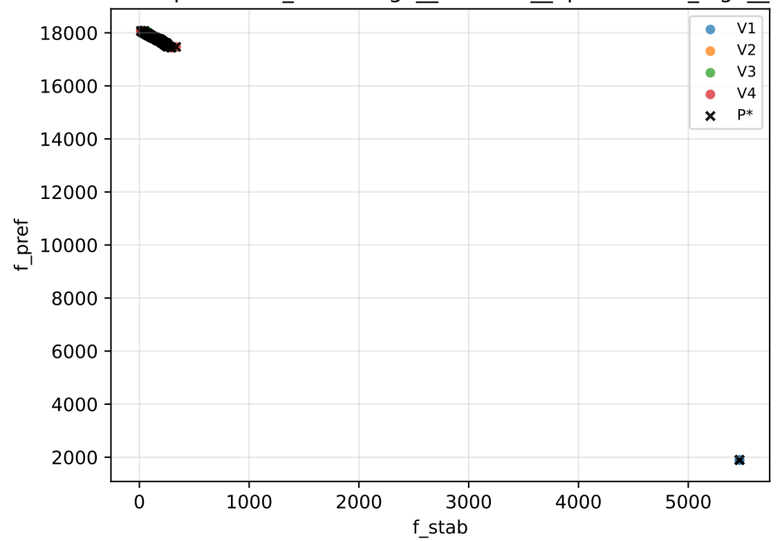
Pareto-Scatter: praxisnah_v1/sc-large__av-loose__dp-weekend_high_se
