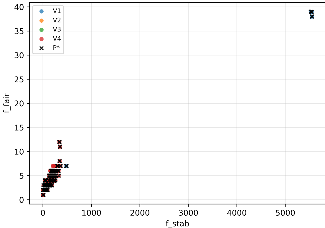
Pareto-Scatter: praxisnah_v1/sc-large__av-loose__dp-weekday_high__sev
