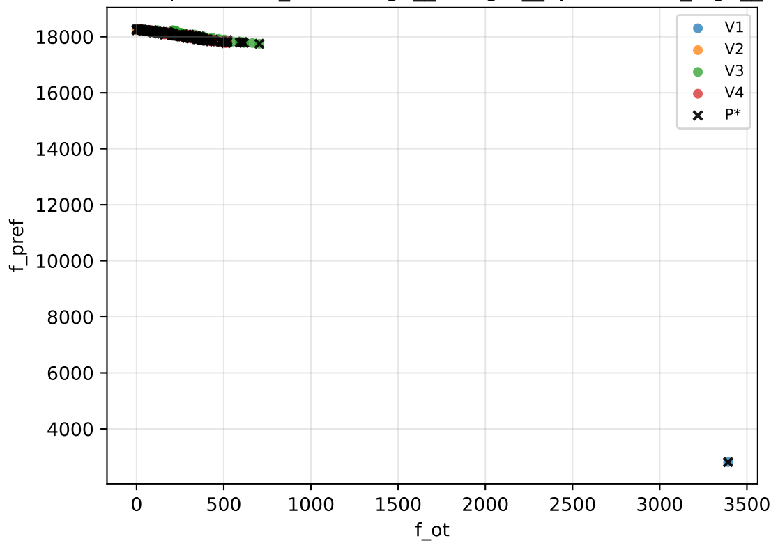
Pareto-Scatter: praxisnah_v1/sc-large__av-tight_dp-weekend_high_se
