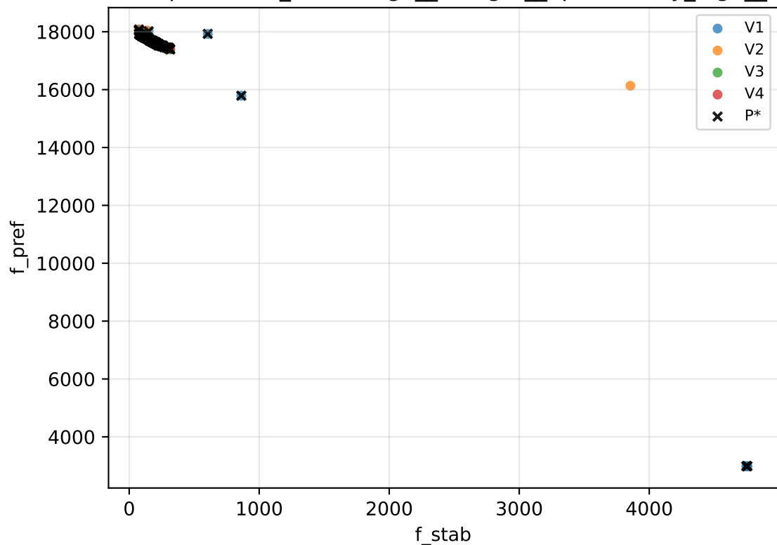
Pareto-Scatter: praxisnah_v1/sc-large__av-tight__dp-weekday_high__sev
