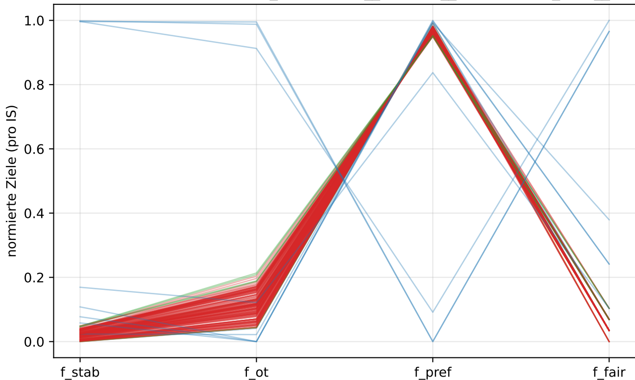
Parallel Coordinates (P*): praxisnah_v1/sc-large_av-tight_dp-weekend_high_sev-s
