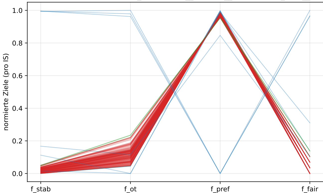
Parallel Coordinates (P*): praxisnah_v1/sc-large_av-tight_dp-weekday_high_sev-s
