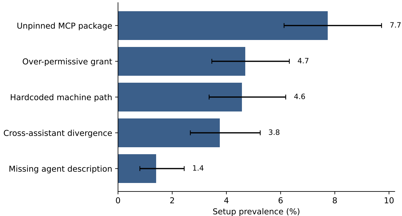
Gating-tier prevalence among setups (95% CI)
