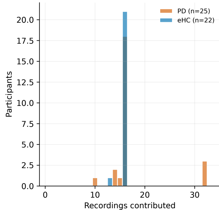
All tasks
