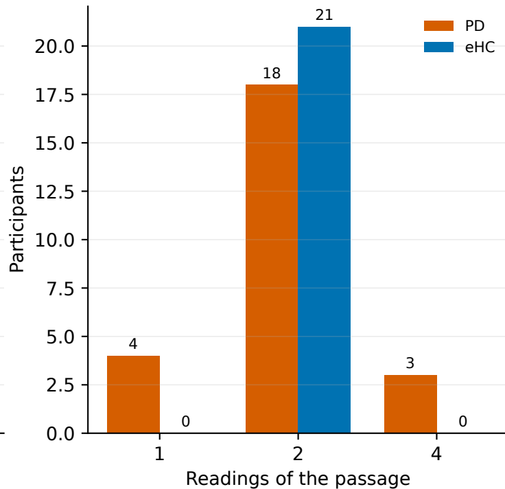
Read-passage task
