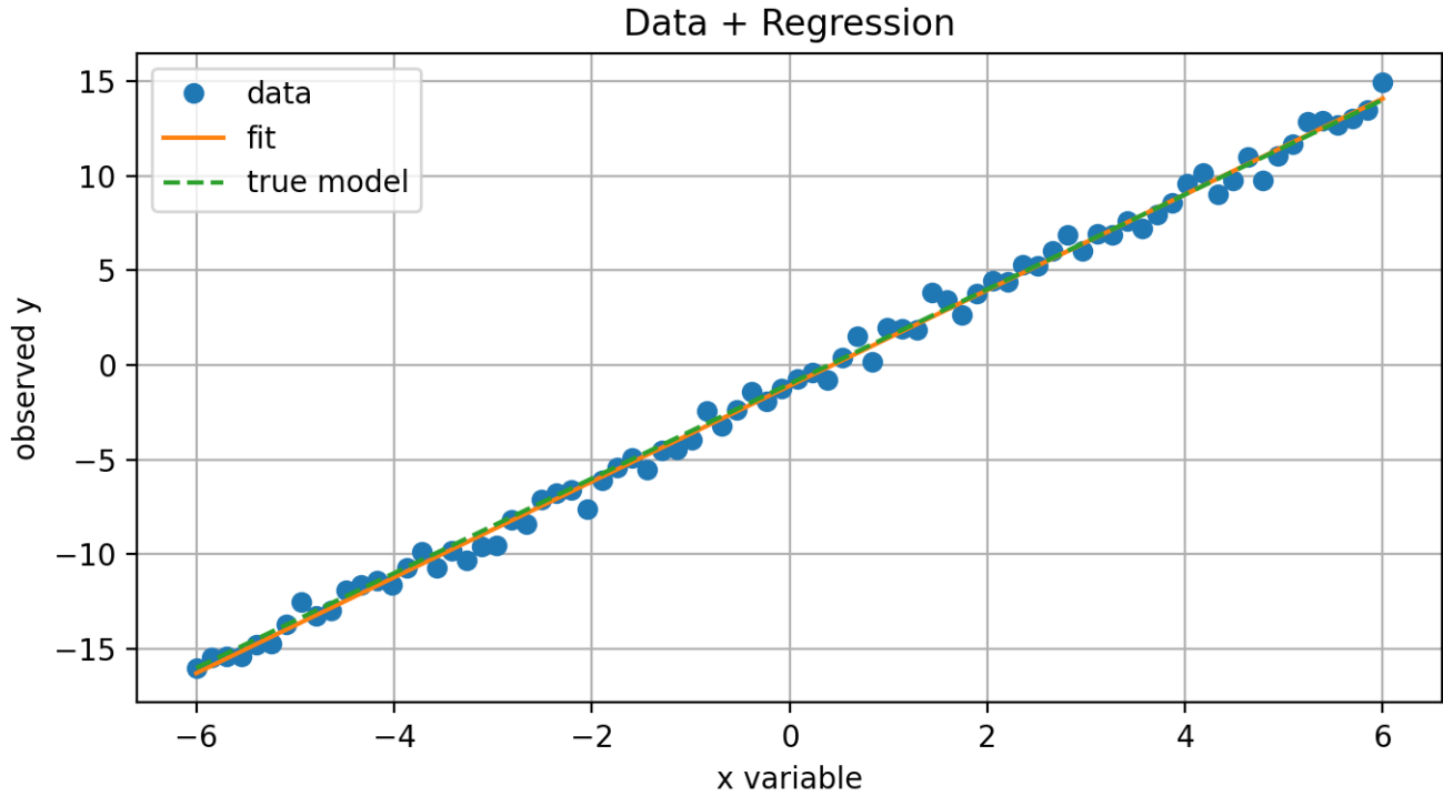
Figure 1: Graph showing linear regression of Demo dataset + true model of Linear regression demonstration
