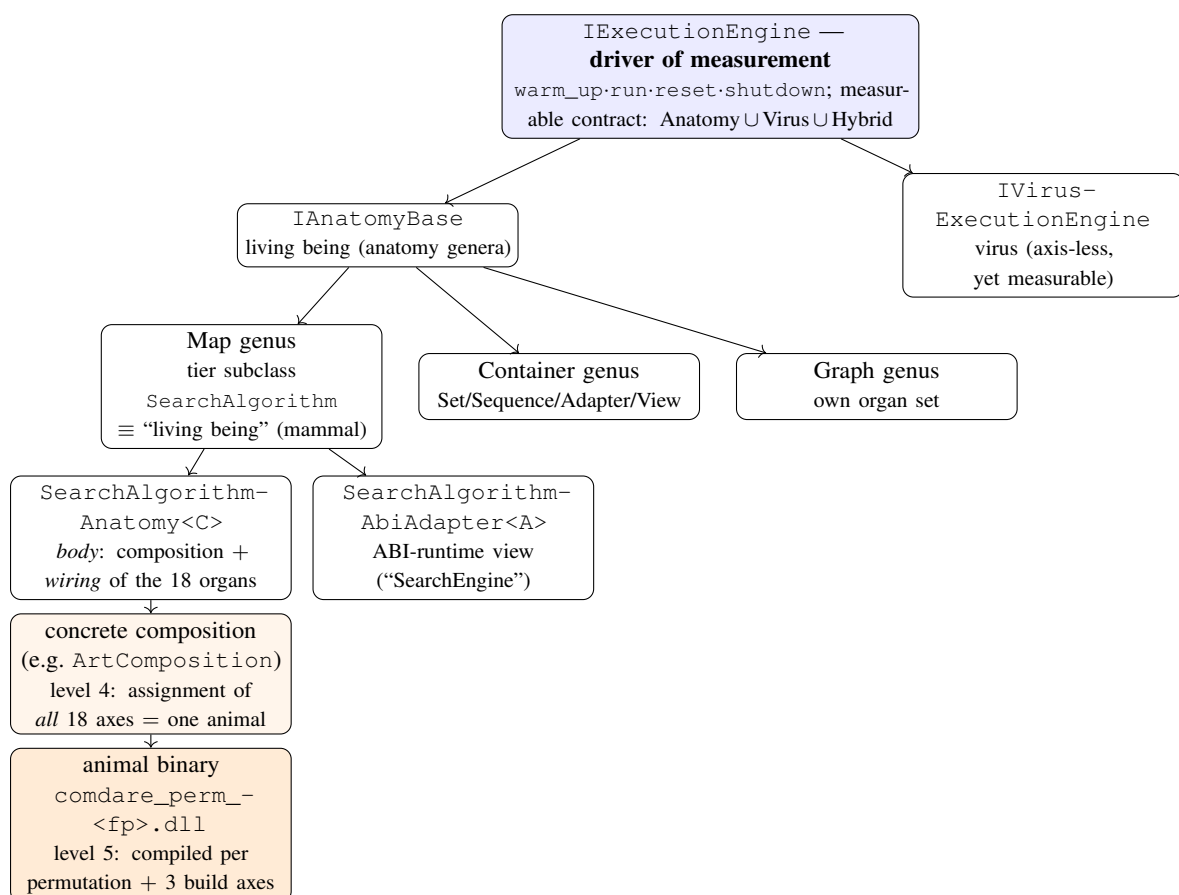
Figure 4.3: The one architecture as a single hierarchy without parallel trees. At the root stands IExecutionEngine as the driver of measurement — the universal measurable contract ( warm_up/run/reset/shutdown ) across all three engine kinds Anatomy , Virus and Hybrid ; beneath it branch the anatomy-bearing genera ( Map , Container , Graph ) and the axis-less viruses . SearchAlgorithm is the focal living being (mammal); its anatomy is its body — the fixed composition and wiring of the 18 organs —, and “ SearchEngine ” only its ABI-runtime view. The mammal branch is drawn out down to the individual: a concrete axis composition (level 4) is compiled per permutation into a standalone animal binary (level 5). Container (keyless storage) and Graph carry their own organ sets.
