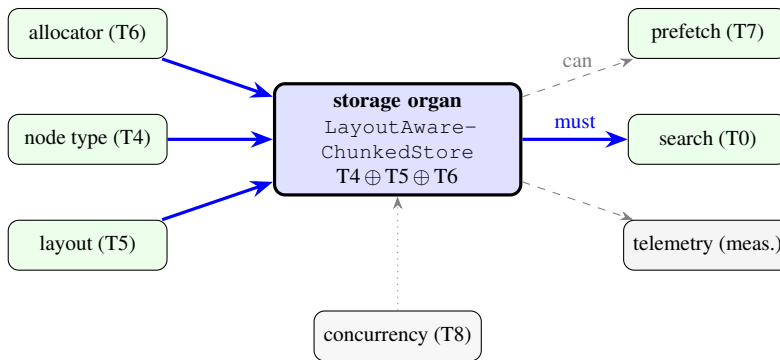
Figure 3.6: Inter-organ usage graph (“which axis uses which”): there is exactly one canonical hub — the storage organ LayoutAwareChunkedStore , which composes node type (T4), layout (T5) and allocator (T6). Mandatorily (solid) the store consumes these three axes, and the search (T0) runs over it. All remaining couplings are optional (dashed): prefetch (T7) and the telemetry (measurement instrumentation, Section 3.4.1) read the store only via requires -gated observer hooks — an axis can use foreign interfaces, but need not. The coupling of concurrency (T8) to the store is not (yet) wired in the code (dotted).
