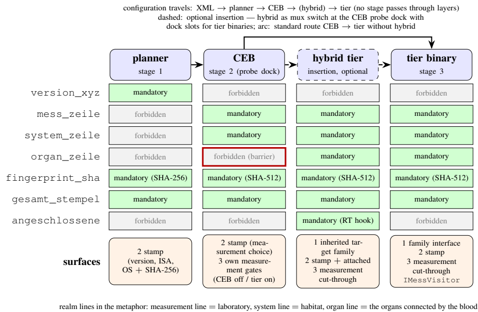
Figure 3.4: Carrier stages and interface surfaces: the three-valued admission matrix of the seven stamp interfaces over the four carrier stages planner, CacheEngineBuilder (CEB), hybrid tier binary (optional insertion), and tier binary (28 cells; green = mandatory, grey = forbidden; the cell organ line/CEB is the static barrier “the CEB carries no organ axes”) and beneath it the interface surfaces per stage — surface 1 family interface (runtime), surface 2 stamp (compile time, ABI-stable), surface 3 measurement cut-through. The configuration travels from the XML via planner and CEB to the tier binary; the hybrid tier binary is a stage optionally inserted between the CEB probe dock and the tier binary (dashed: mux switch at the probe dock with dock slots for tier binaries; the column order of the matrix follows the processing topology with the hybrid at its insertion position, the arc is the standard route without hybrid); no stage passes through layers, each contains its layer compiled in.
