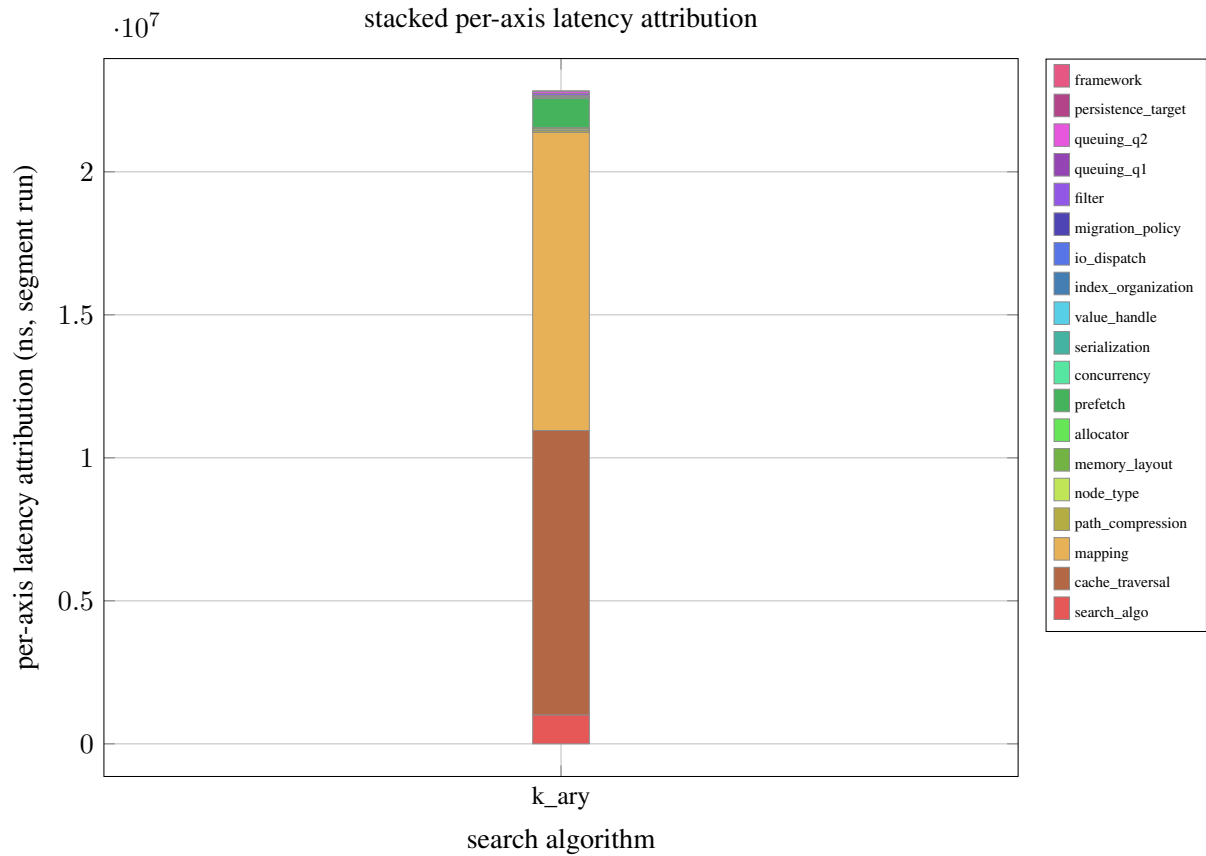
Figure A.7: stacked per-axis latency attribution
