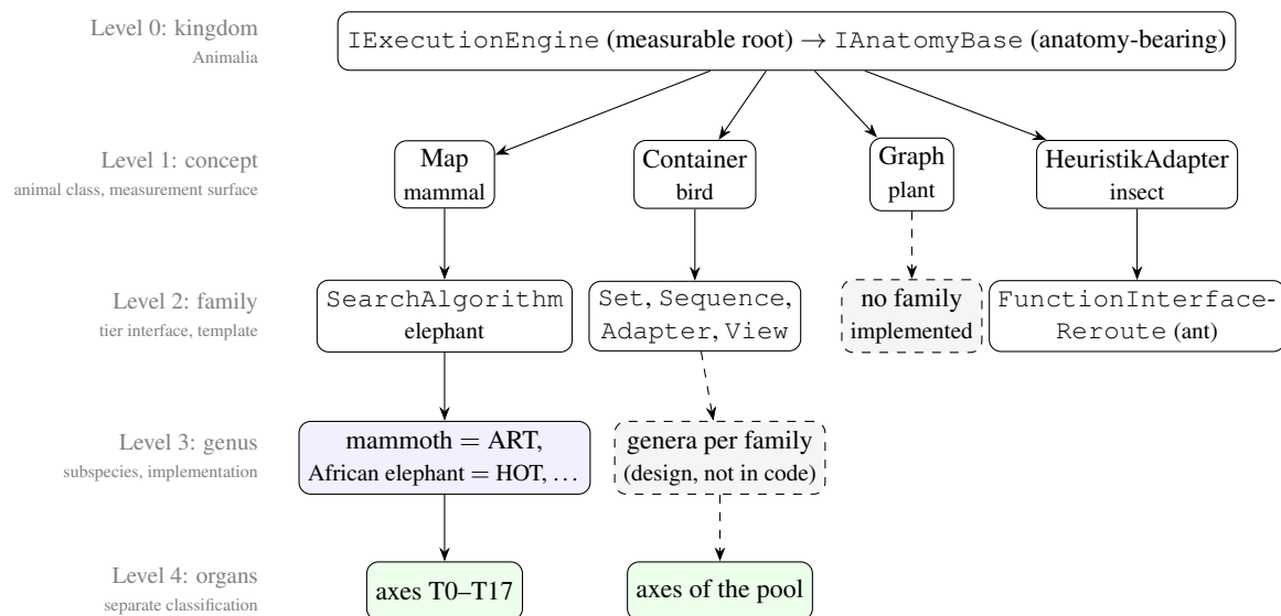
Figure 3.7: The three-level model: the three interface levels concept (level 1, animal class, measurement surface: probe dock) → family (level 2, tier interface, template outward) → genus (level 3, subspecies: implementation of the family interface, possibly with extended special interfaces); beneath them the organs/axes (level 4, a classification of their own), above them the kingdom (level 0). Four concepts: Map (mammal) possesses as its sole family SearchAlgorithm (elephant), whose genera are the concrete implementations (mammoth = ART, African elephant = HOT, Indian elephant = START); Container (bird) the families Set/Sequence/Adapter/View (woodpecker/stork/cockatoo/falcon), which are formed from the same axis pool; Graph (plant) is laid out as an interface, a family is not implemented; HeuristikAdapter (insect) possesses the reroute family FunctionInterfaceReroute (ant) of the hybrid tier. Today the code carries the genus only as an axis assignment; the genus implementation class is an acknowledged architecture error (fix after the defence). Tier binary (level 5a) and hybrid tier (level 5b) are the post-phase of the compilation (Figure 3.8).
