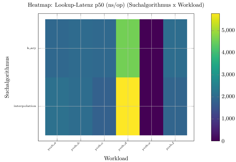
Figure 1: Heatmap: Lookup-Latenz p50 (ns/op) (Suchalgorithmus x Workload)
