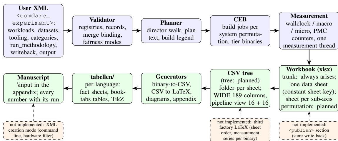
Figure 5.1: The automated evaluation chain from the user XML to the manuscript. Upper row: The XML declares what, where, and when; the validator checks it against the registries; the planner emits the deterministic plan; the CEB builds the tier binaries per system permutation; the measurement collects the three measurement levels and the counters with one measurement thread. Lower row: The workbook is the trunk (one data sheet under a constant sheet key; the fan-out into one sheet per sub-axis permutation is planned but not implemented), the CSV form its ordered tree of CSV files generated from it (one folder per sheet; not a single child document; implemented is a flat file), the generators render per language into the tabellen directory, the manuscript includes the files — every number carries its run. Dashed: parts not implemented (XML creation mode, <publish> section, third factory).
