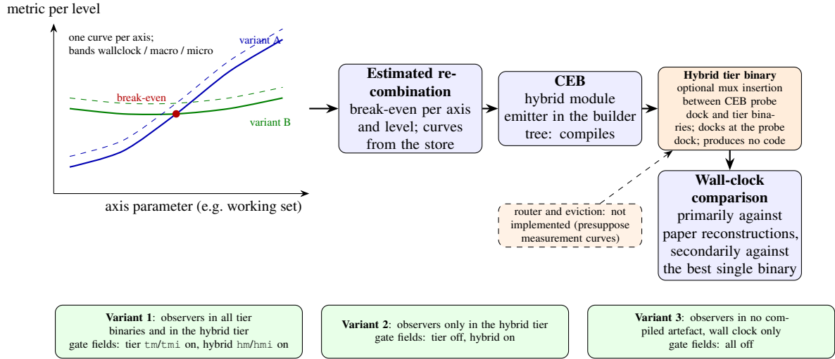
Figure 5.3: The measurement-curve type system in the heuristic counter-proof. Left: per axis one curve of the metric over the axis parameter, separated by measurement level (wallclock, macro, micro); the intersection of two variants is the break-even point from which the recombination is estimated. Middle and right: The CEB compiles the estimated recombination via the hybrid module emitter; the hybrid tier binary is the mux stage optionally inserted between the CEB probe dock and the tier binary, docks at the probe dock, carries dock slots for tier binaries, and itself produces no code; the comparison is made on the wall clock, primarily against the paper reconstructions, secondarily against the best single binary. Bottom: the three build variants of the measurement-error test plan, kept apart via the gate fields of the fingerprint. Dashed: router and eviction (not implemented).
