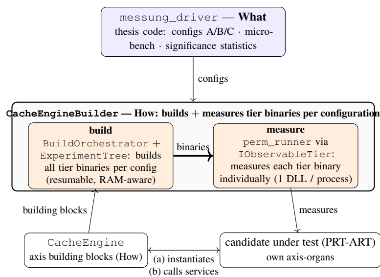
Figure 3.15: The M-model focused on the build and measurement phases. The outer messung_driver loop ( What , thesis code) feeds the configurations of the three measurement series A/B/C; the CacheEngineBuilder ( How , library) splits into the two genuinely interesting phases: build ( BuildOrchestrator/ExperimentTree builds a standalone tier binary per configuration, resumable and RAM-aware) and measure ( perm_runner drives and measures each tier binary individually through the observer interface IObservableTier ). The CacheEngine supplies the default axis building blocks, the candidate under test PRT-ART its own organs; their bidirectional relationship ((a) instantiates, (b) calls services) founds the multi-candidate capability. The ExecutionEngine remains the shared measurable root.
