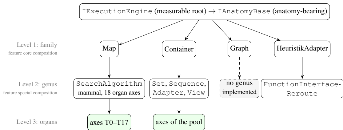
Figure 3.7: The three-level model: family (level 1, outer interface, feature core composition) → genus (level 2, fixed axis set, feature special composition) → organs/axes (level 3). Four families: Map possesses as its sole genus SearchAlgorithm , the “mammal” with the eighteen organ axes; Container the genera Set/Sequence/Adapter/View , which are formed from the same axis pool; Graph is laid out as an interface, a genus is not implemented; HeuristikAdapter possesses the reroute genus FunctionInterfaceReroute of the hybrid tier.
