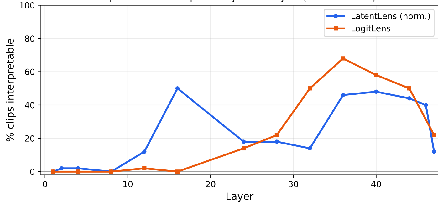
Speech token interpretability across layers (Gemma 4 12B)
