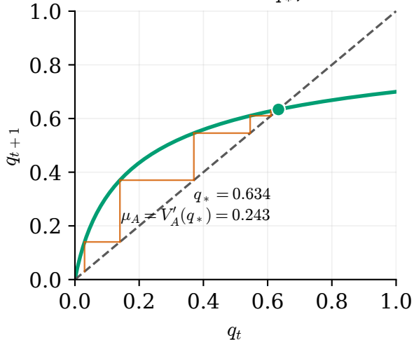
Iteration toward q_* , A = 2.5
