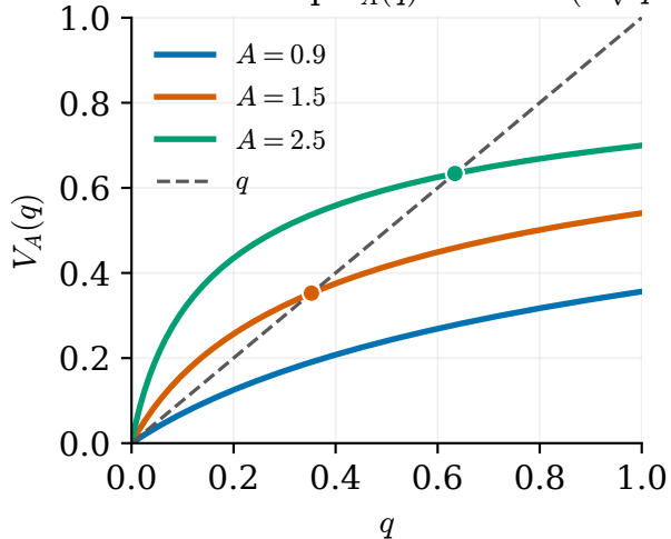
Mean-field map V_A(q) = \mathbb{E} \tanh^2(A\sqrt{q} G)
