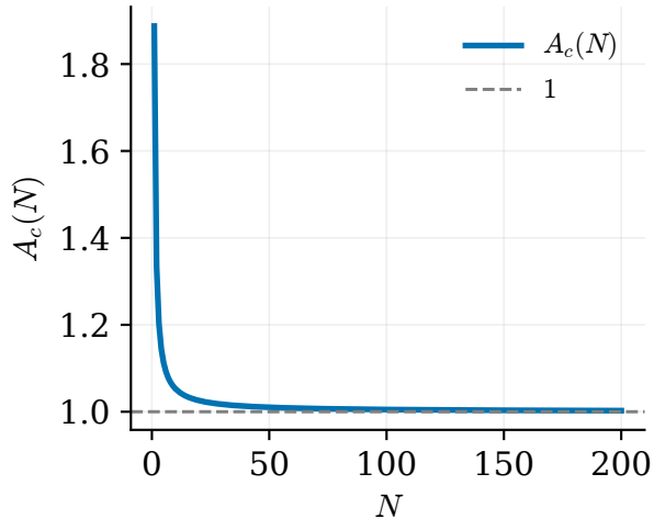
Fixed-width threshold A_c(N) \downarrow 1
