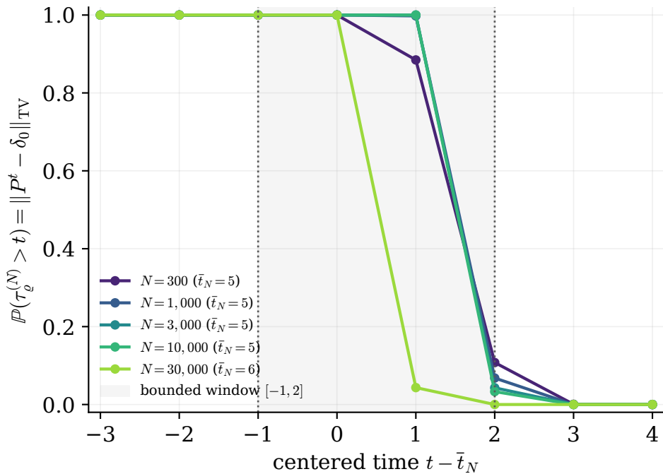
Subcritical dimension cutoff, A = 0.7 , \varrho = 0.5
