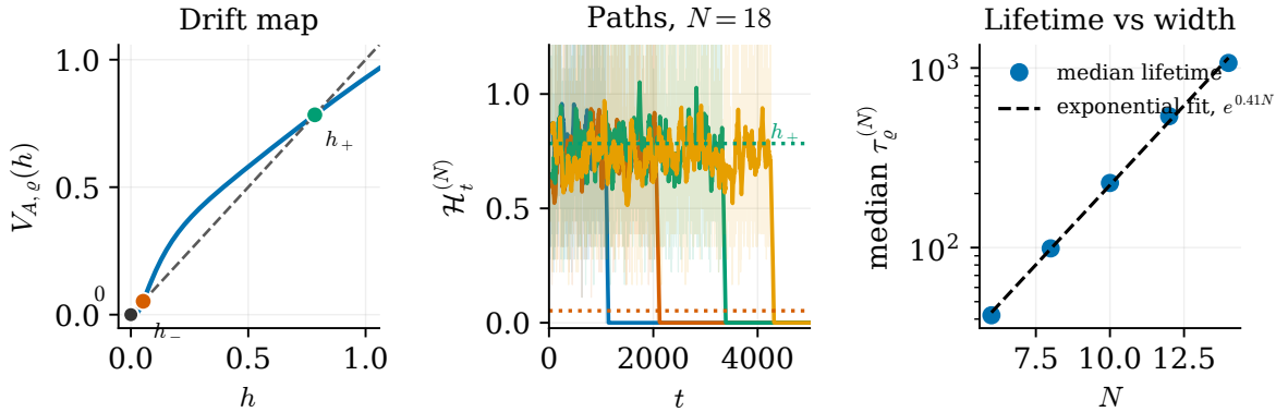
Figure 8.6: Metastability for A = 1.15 and \varrho = 0.5 . Left: the map V_{A, \varrho} with unstable endpoint h_- and stable endpoint h_+ . Middle: representative paths and moving averages with window 60. Right: median absorption times and an exponential fit. The observed growth is consistent with Theorem 5.2.
