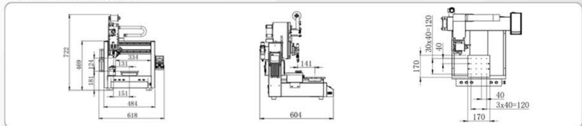
ET9483C Dimensions
