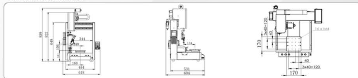
ET9484C Dimensions
