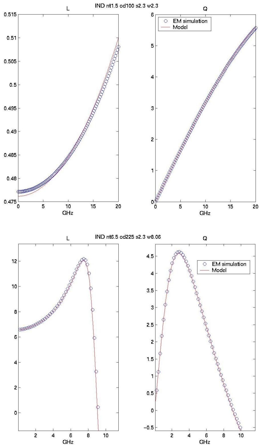
Figure 2-1 LQ plot of Spiral Inductor
