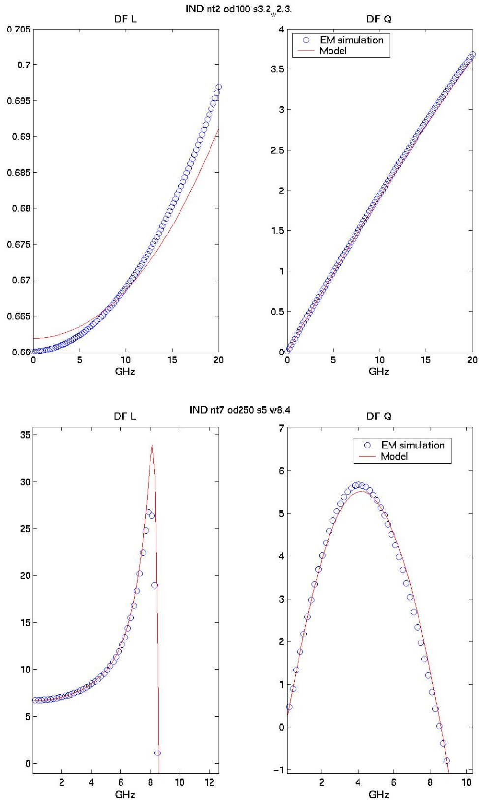
Figure 2-4 LQ plot of Symmetric Inductor with Center Tap
