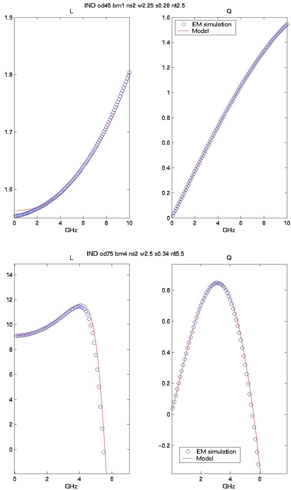
Figure 2-5 LQ plot of Stack Inductor
