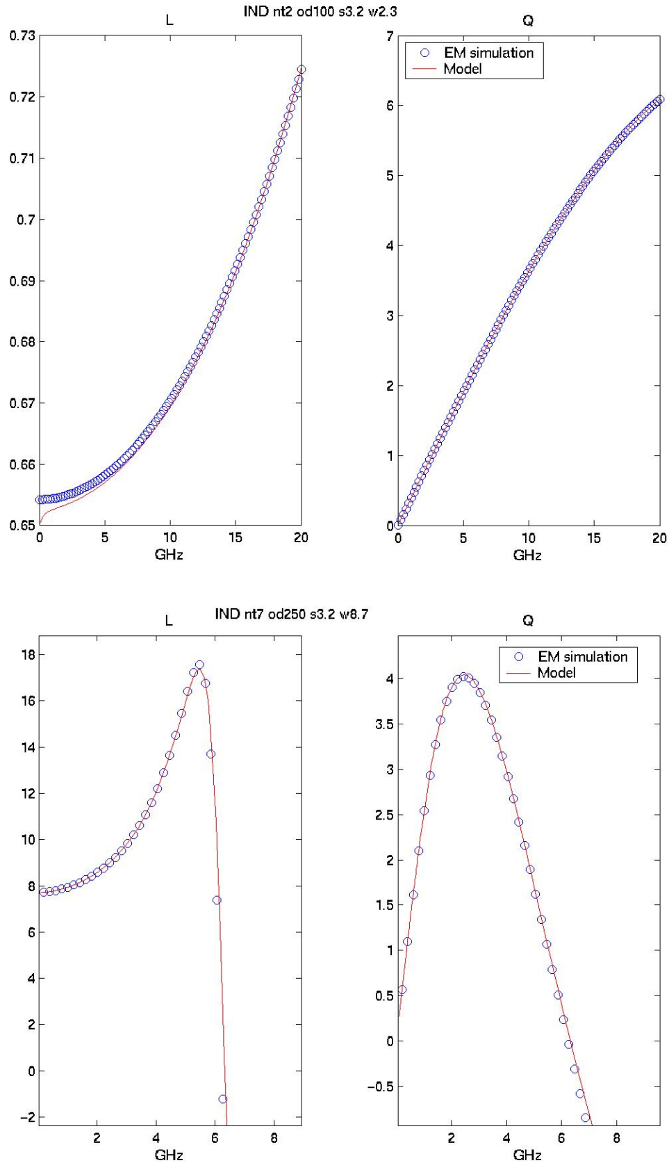
Figure 2-3 LQ plot of Symmetric Inductor
