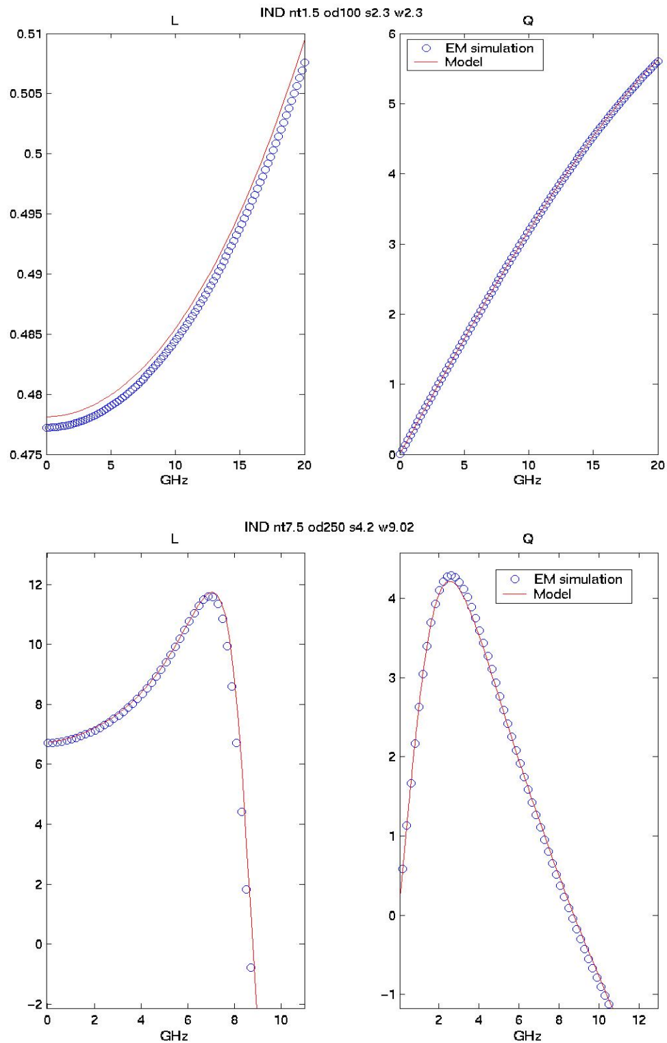
Figure 2-2 LQ plot of Spiral Inductor
