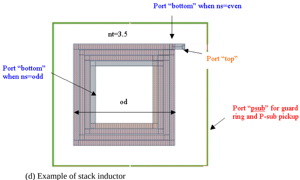
Figure 1-1 Sample layout of Inductor
