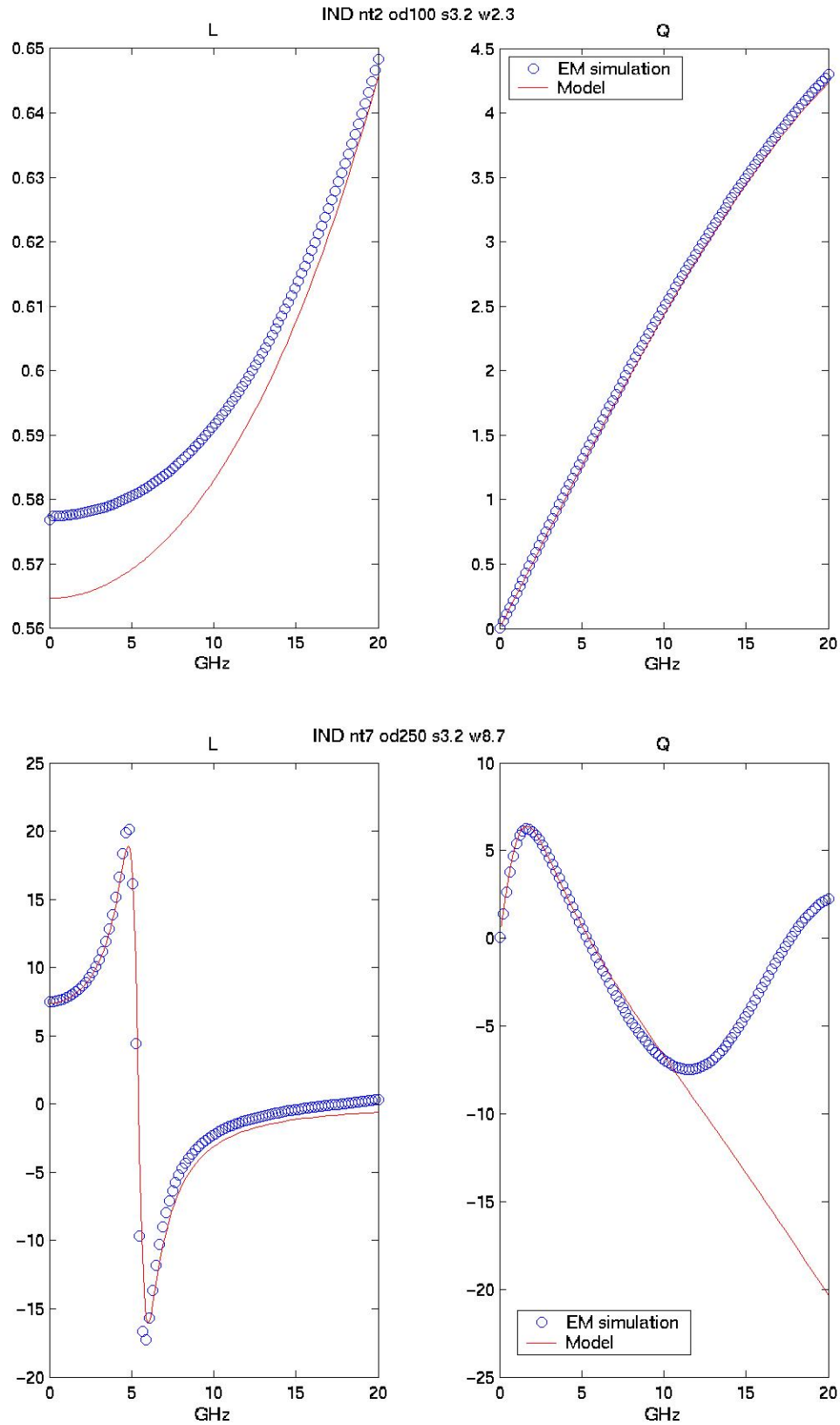
Figure 2-3 LQ plot of Symmetric Inductor
