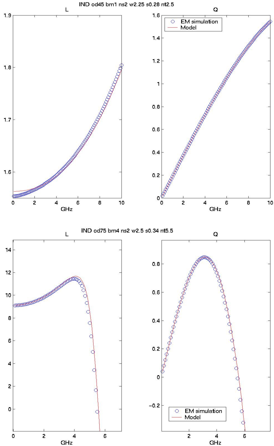
Figure 2-5 LQ plot of Stack Inductor
