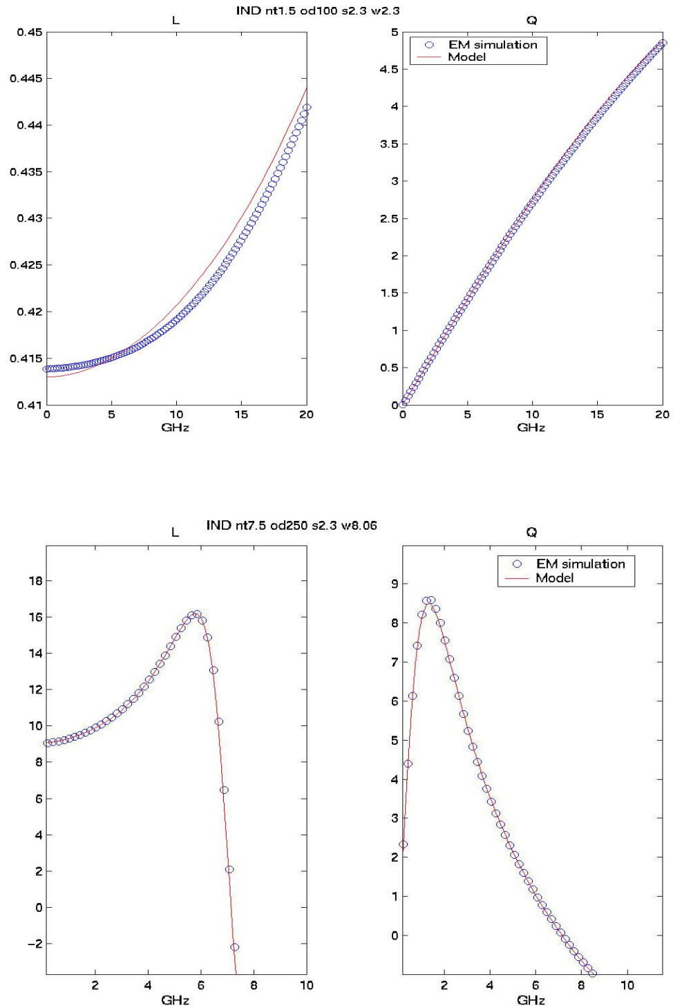
Figure 2-2 LQ plot of Spiral Inductor
