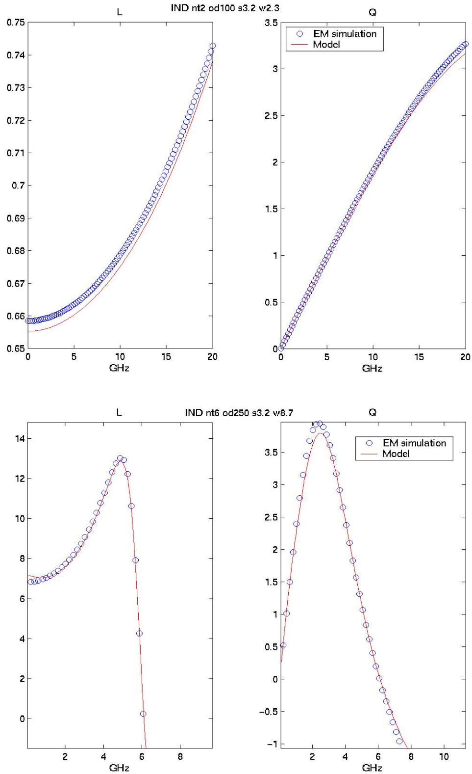
Figure 2-3 LQ plot of Symmetric Inductor
