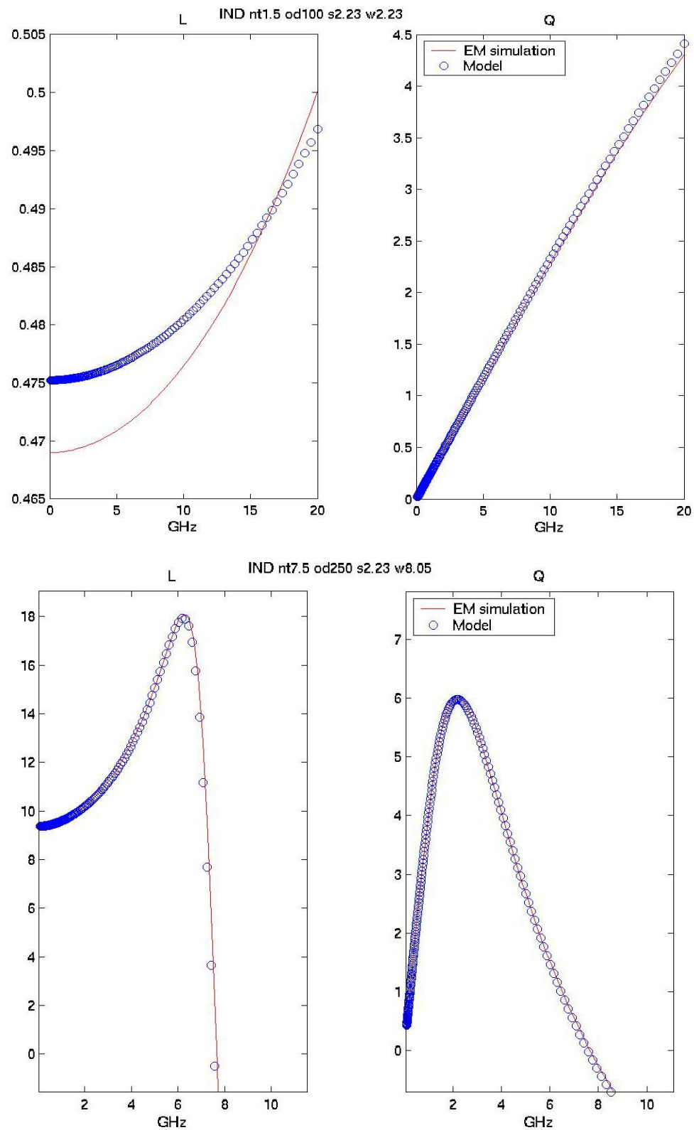
Figure 2-2 LQ plot of Spiral Inductor
