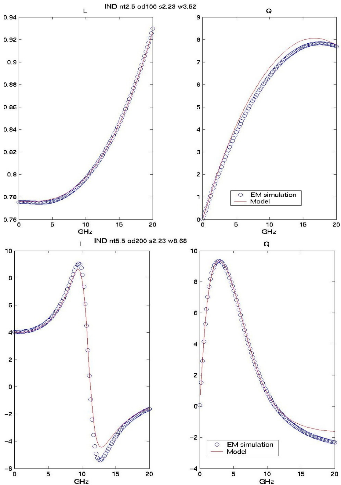
Figure 2-2 LQ plot of Spiral Inductor
