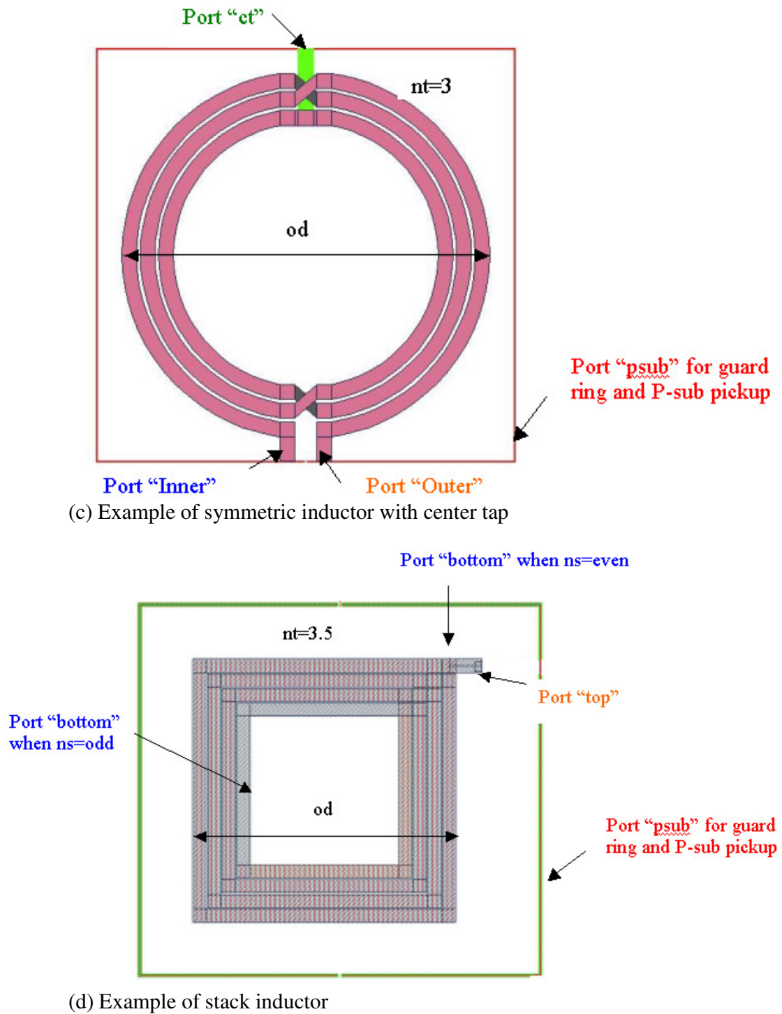
Figure 1-1 Sample layout of Inductor
