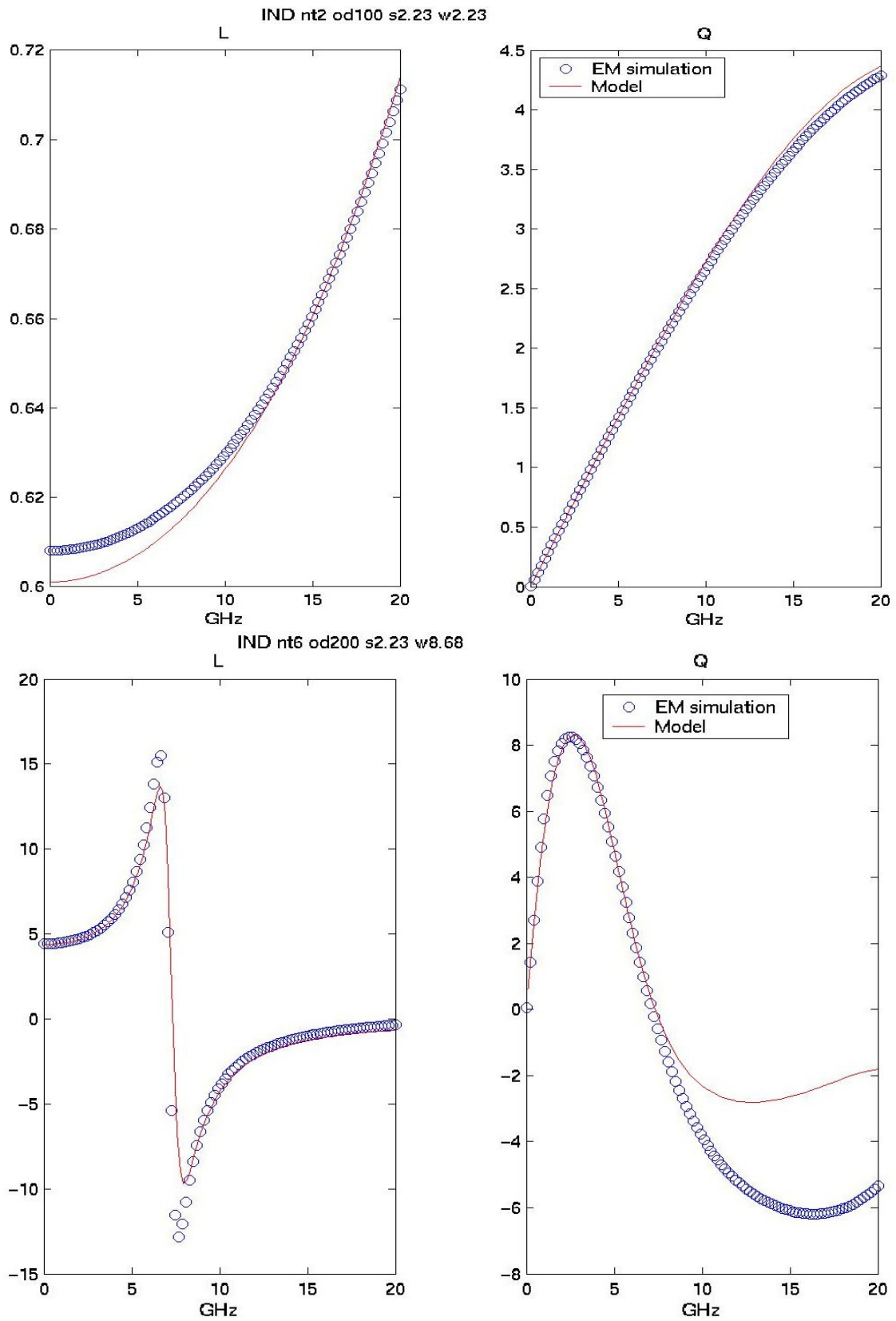
Figure 2-3 LQ plot of Symmetric Inductor
