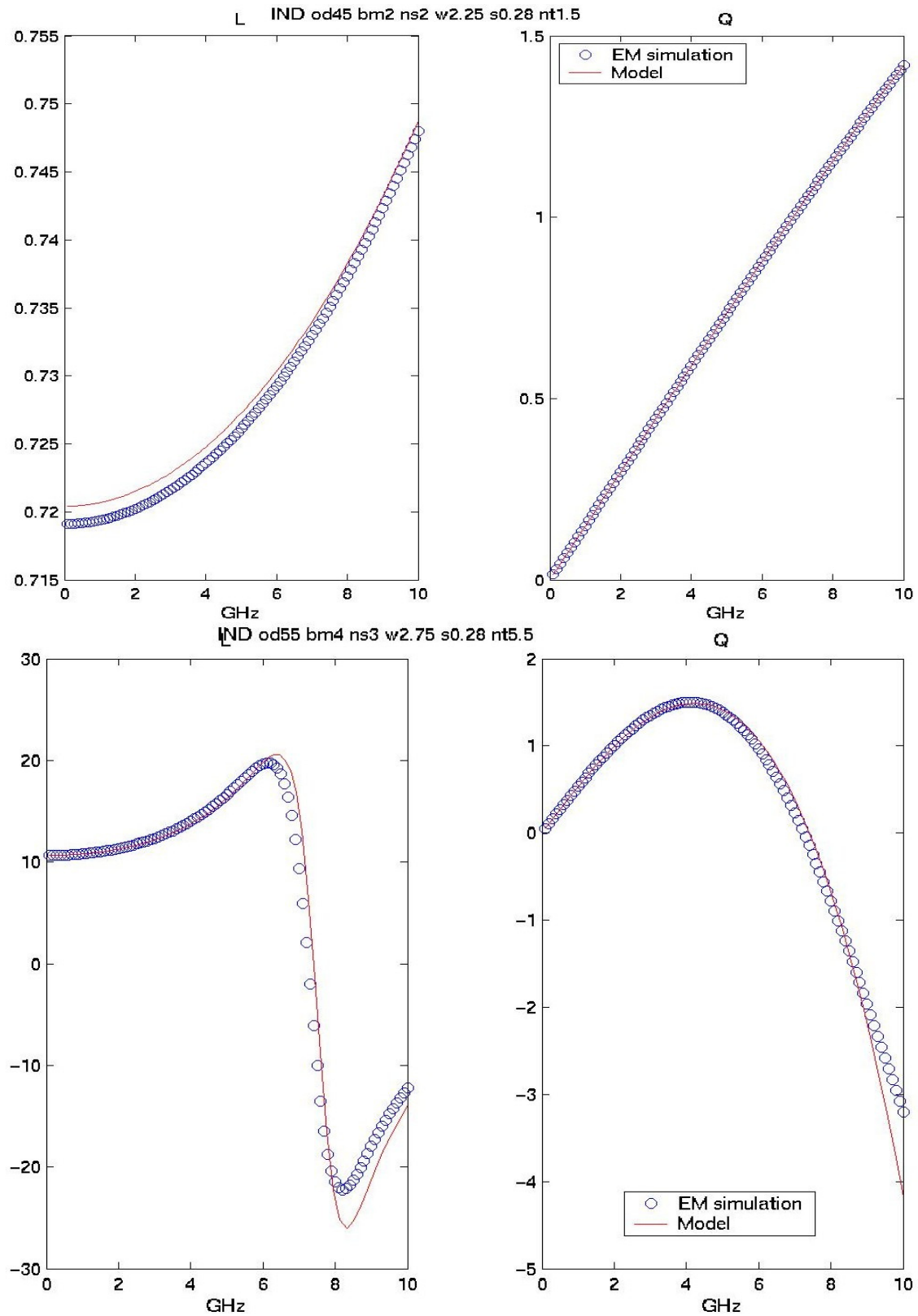
Figure 2-5 LQ plot of Stack Inductor
