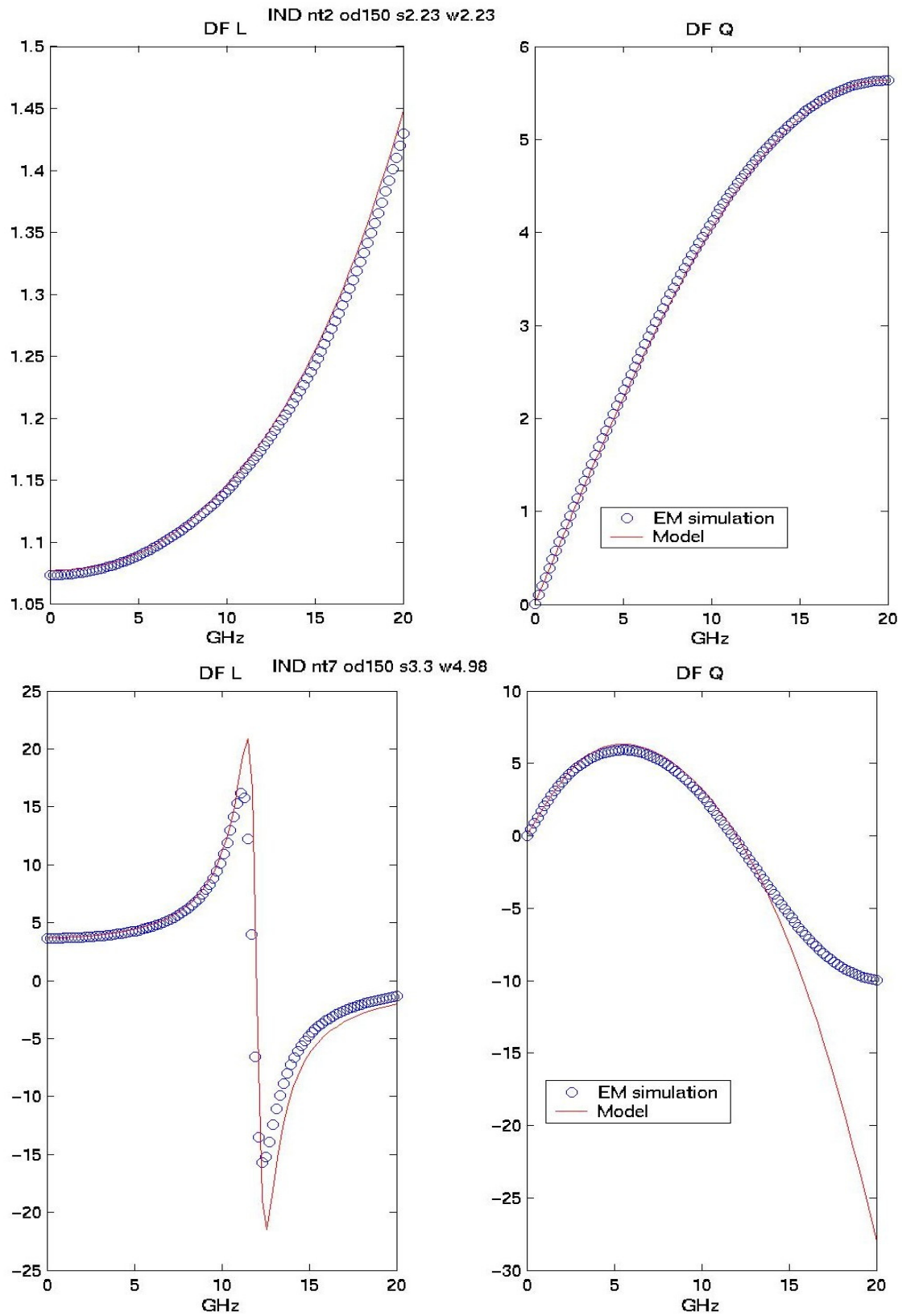
Figure 2-4 LQ plot of Symmetric Inductor with Center Tap
