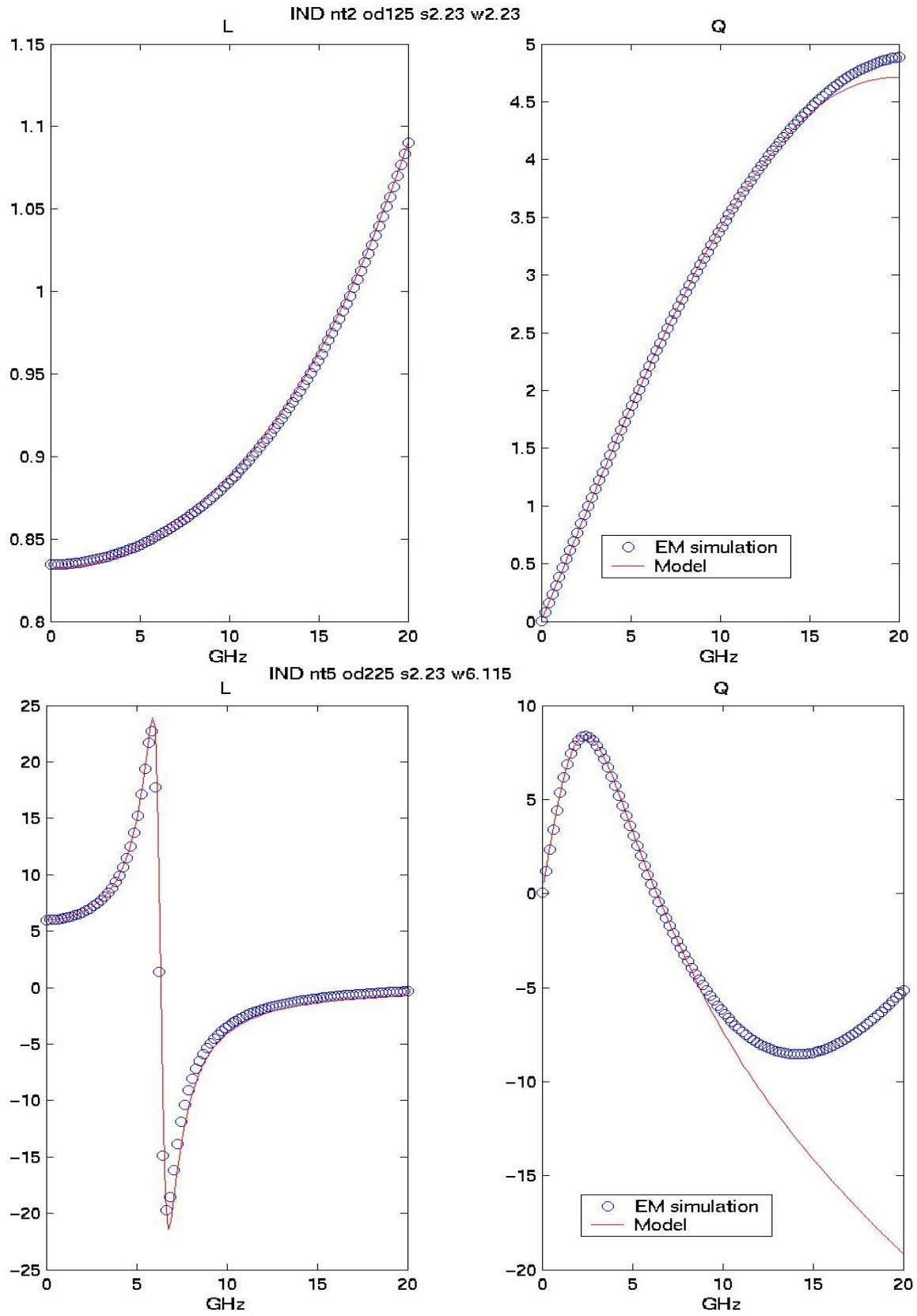
Figure 2-3 LQ plot of Symmetric Inductor
