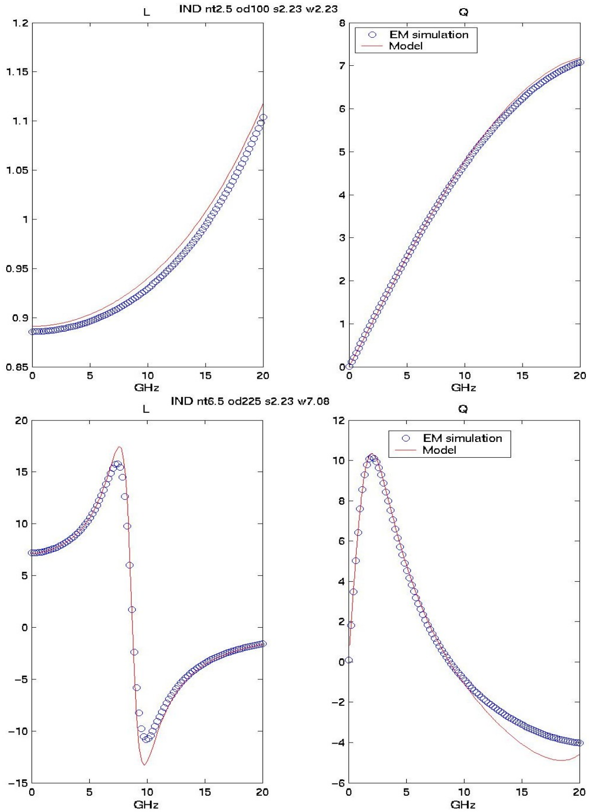
Figure 2-2 LQ plot of Spiral Inductor
