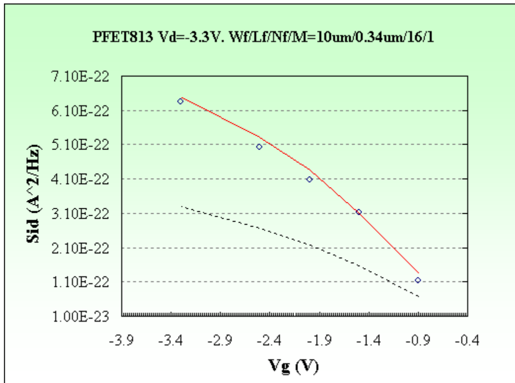
Figure 2-2c PFET813: Vd=-3.3V
