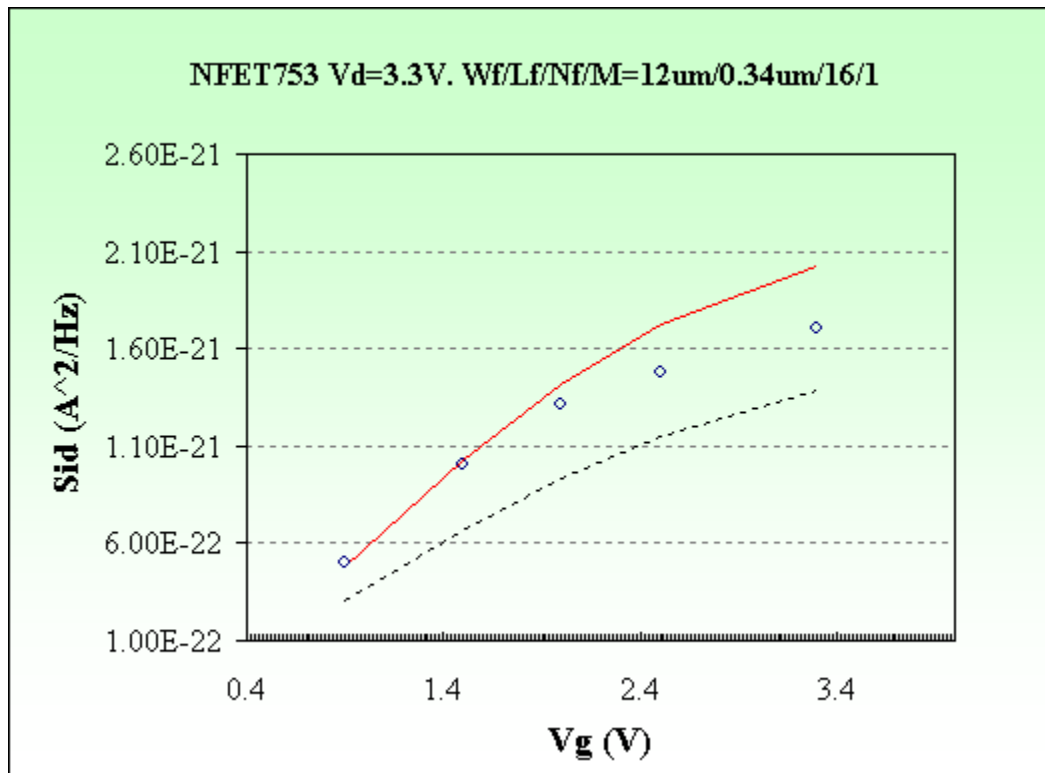
Figure 2-1c NFET753: Vd=3.3V
