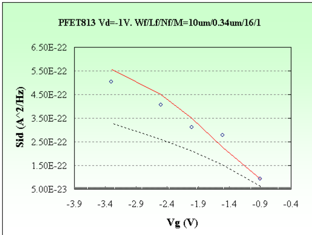
Figure 2-2a PFET813: Vd=-1V
