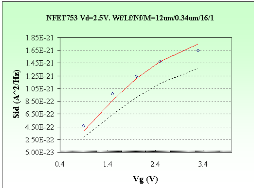
Figure 2-1b NFET753: Vd=2.5V
