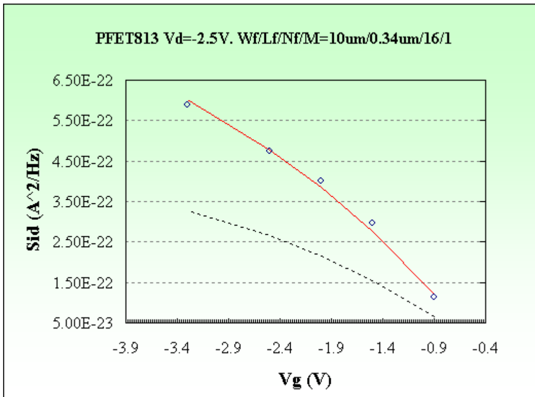
Figure 2-2b PFET813: Vd=-2.5V
