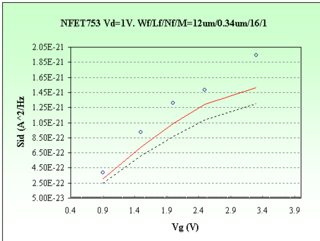
Figure 2-1a NFET753: Vd=1V
