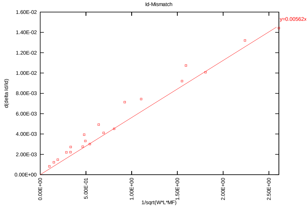
Figure 4-3 Idsat mis-matching simulation of 3.3V n-ch MOSFET
