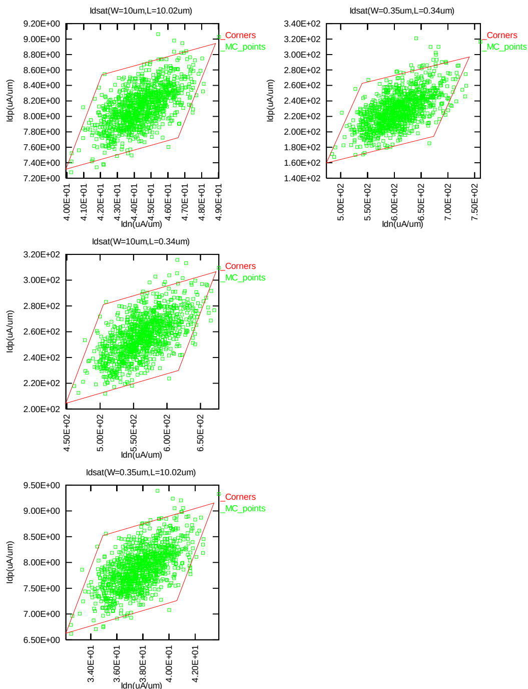
Figure 2-3 Monte Carlo graph of saturation current
