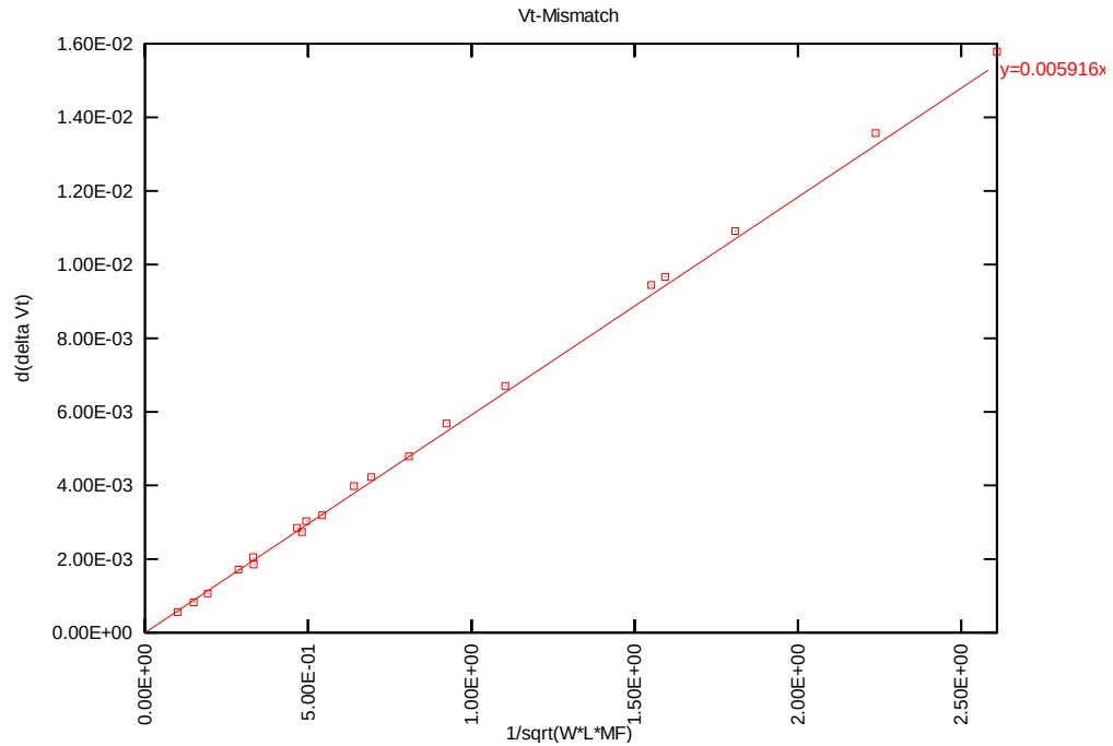
Figure 4-2 VTLIN mis-matching simulation of 3.3V p-ch MOSFET
