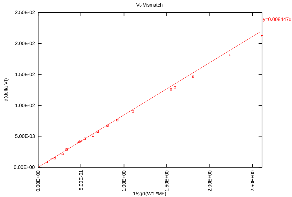
Figure 4-1 VTLIN mis-matching simulation of 3.3V n-ch MOSFET
