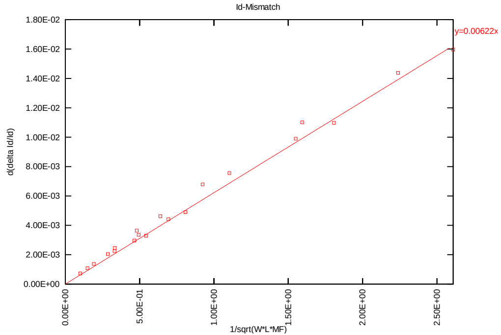
Figure 4-4 Idsat mis-matching simulation of 3.3V p-ch MOSFET
