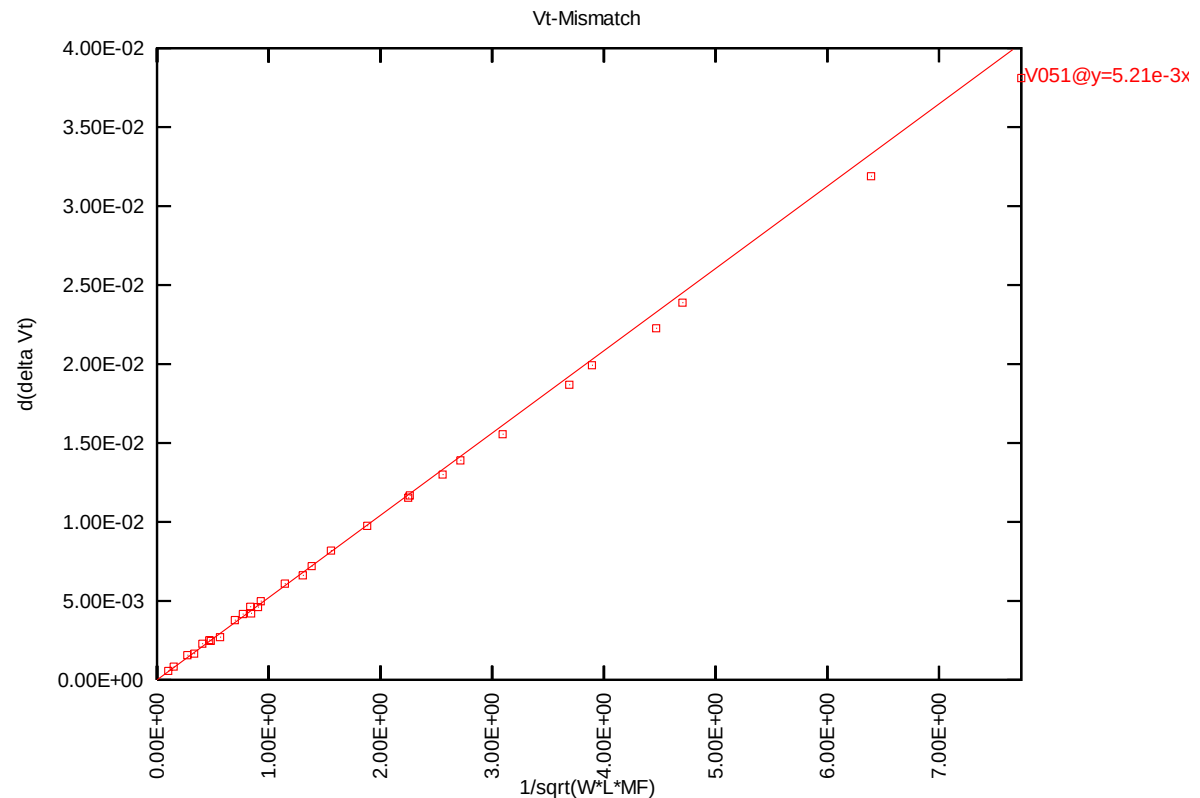
Figure 4-1 VTLIN mis-matching simulation of 1.2V n-ch MOSFET
