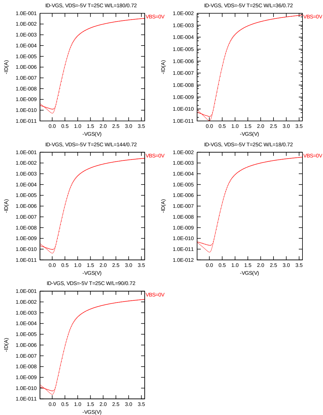
Figure 3-8 Log scaled I_D vs. V_{GS} at V_{DS} = -5.0 V for PMOS
