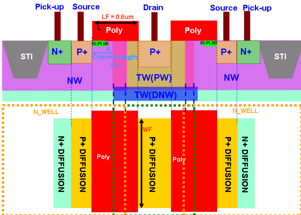
Figure 1-2 Top and Cross-sectional views of D5.0G3.3 p-ch MOSFETs unit
