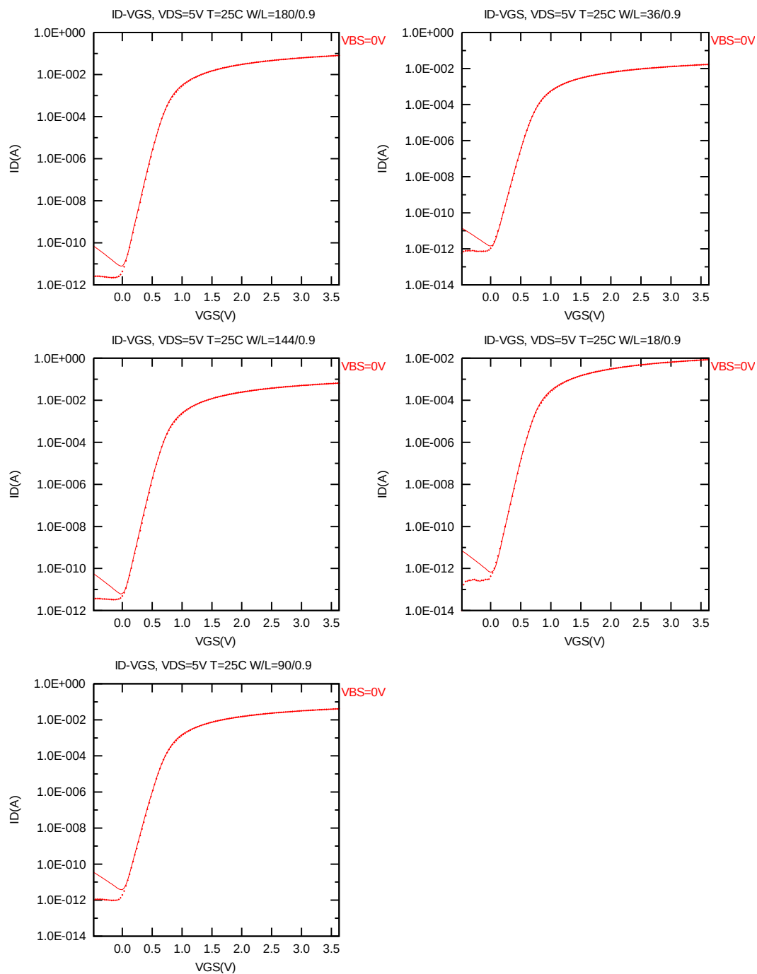
Figure 2-8 Log scaled I_D vs. V_{GS} at V_{DS} = 5.0 V for NMOS
