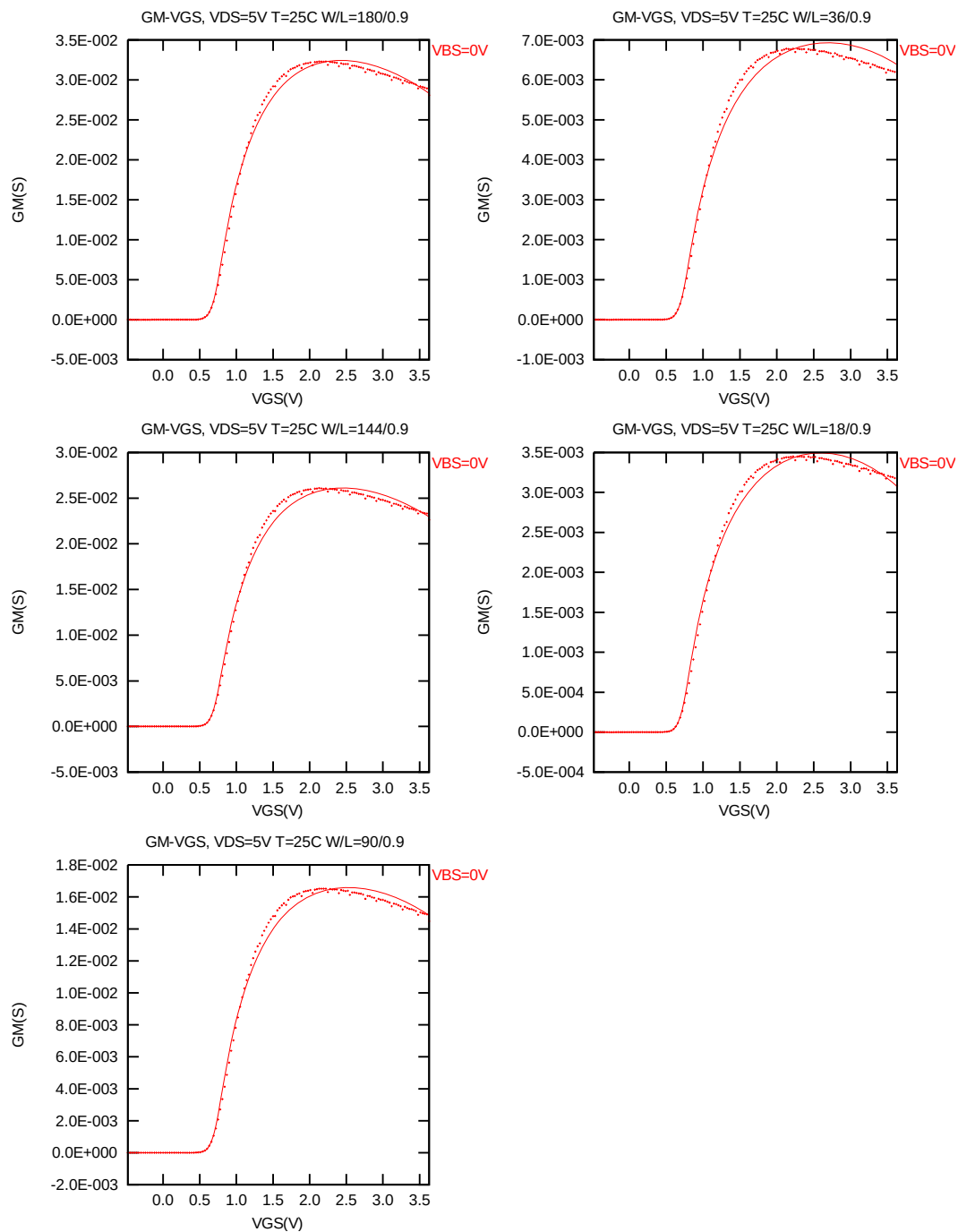
Figure 2-11 G_M vs. V_{GS} at V_{DS} = 5.0 V for NMOS
