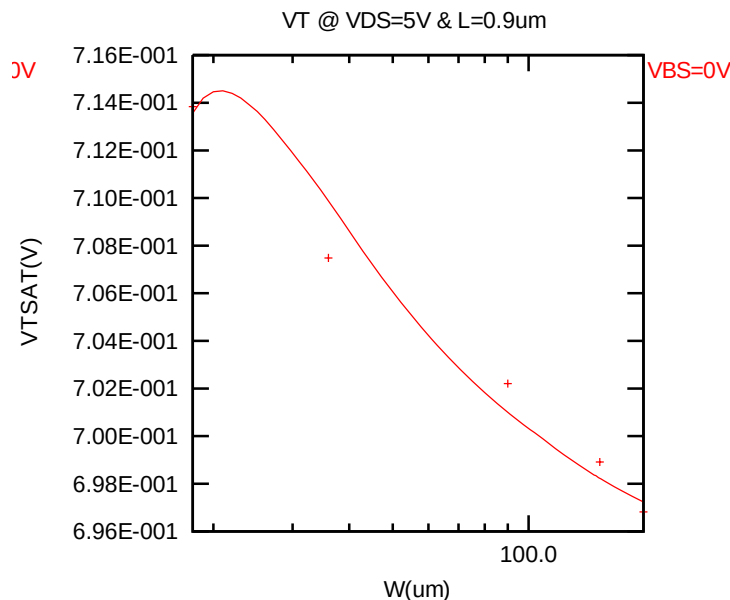
Figure 2-13 V_{TSAT} vs. channel width for high drain bias ( V_{DS} = 5.0 V) for NMOS
