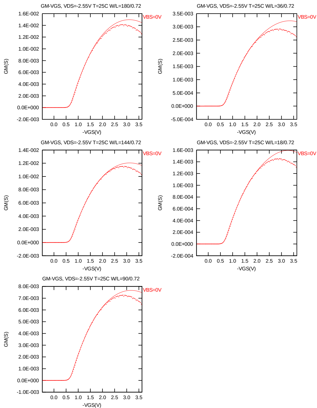
Figure 3-10 G_M vs. V_{GS} at V_{DS} = -2.55 V for PMOS
