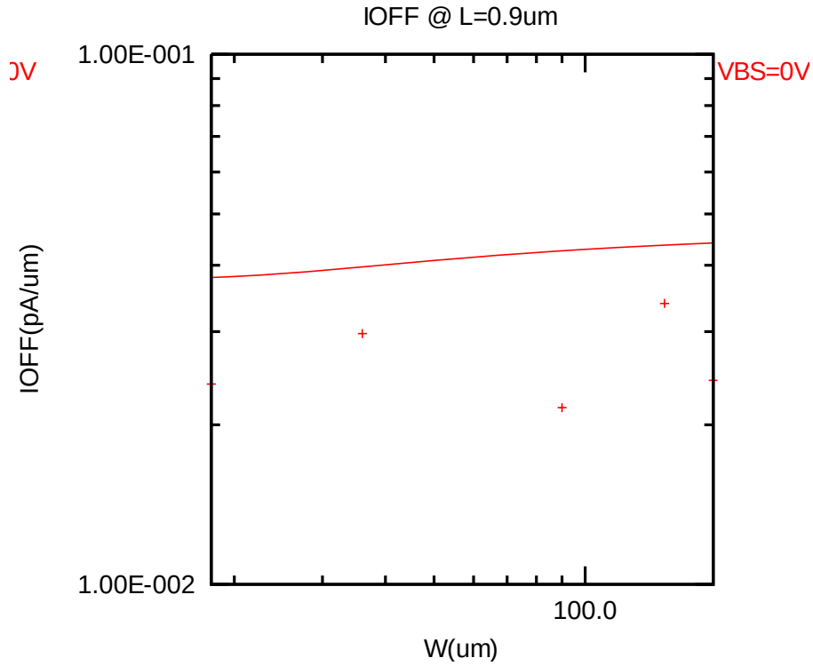
Figure 2-16 I_{OFF} vs. channel width for NMOS
