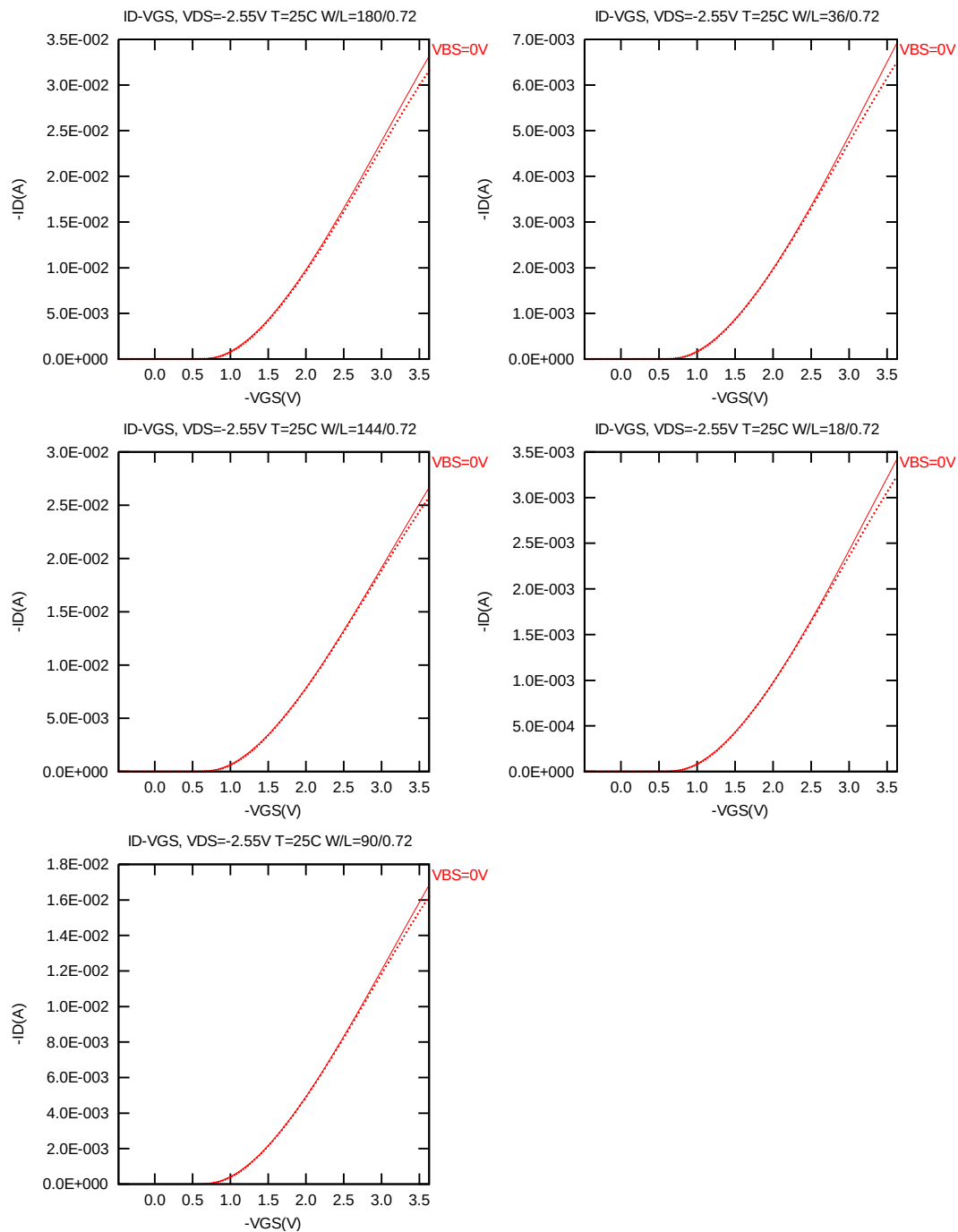
Figure 3-4 I_D vs. V_{GS} at V_{DS} = -2.55V for PMOS
