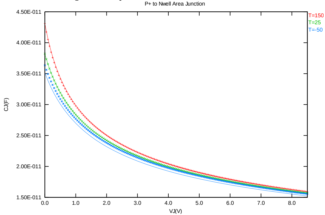
Figure 3-29 Bottom area junction capacitance at -50^\circ\text{C} , 25^\circ\text{C} and 150^\circ\text{C} for PMOS
