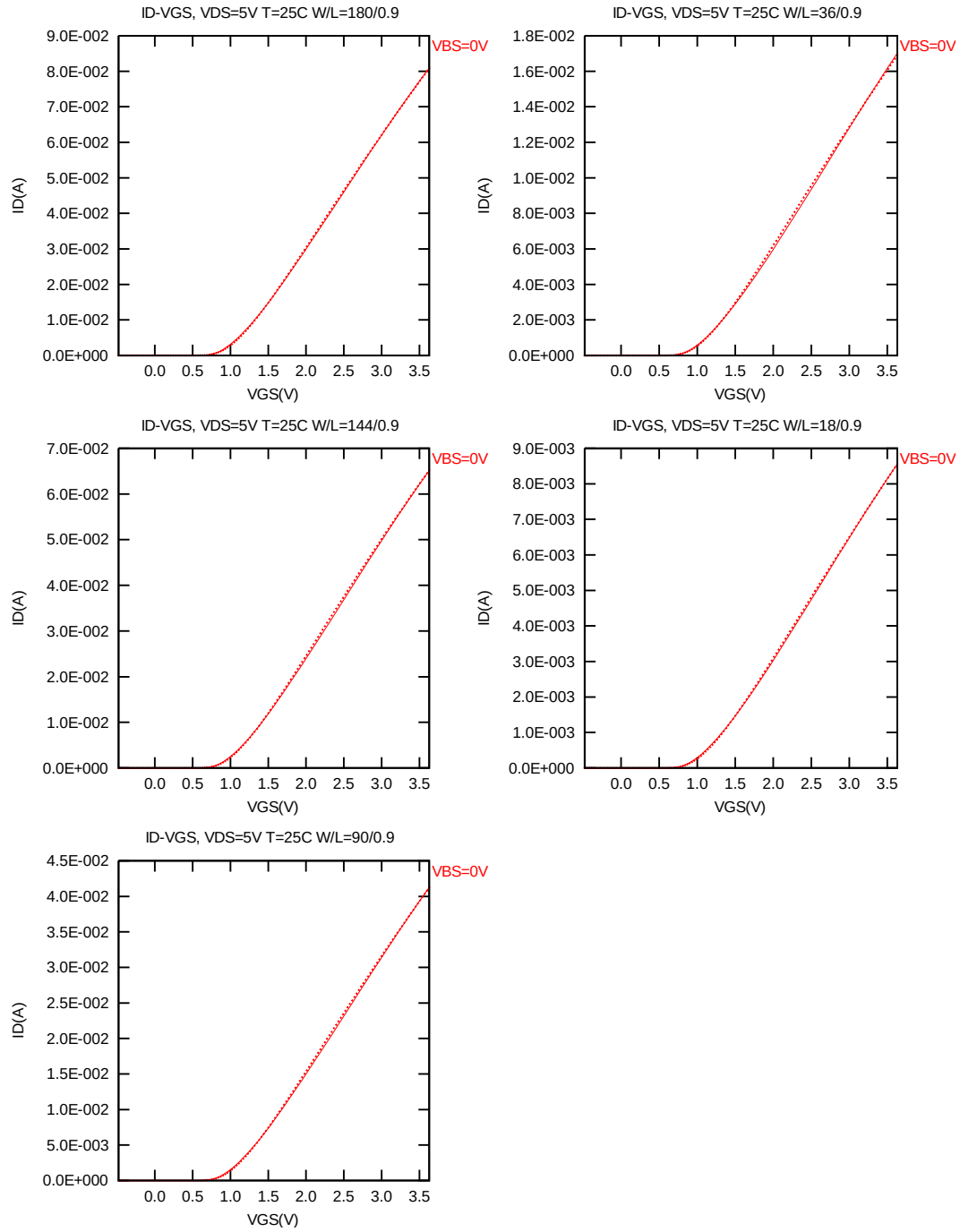
Figure 2-5 I_D vs. V_{GS} at V_{DS} = 5.0 V for NMOS
