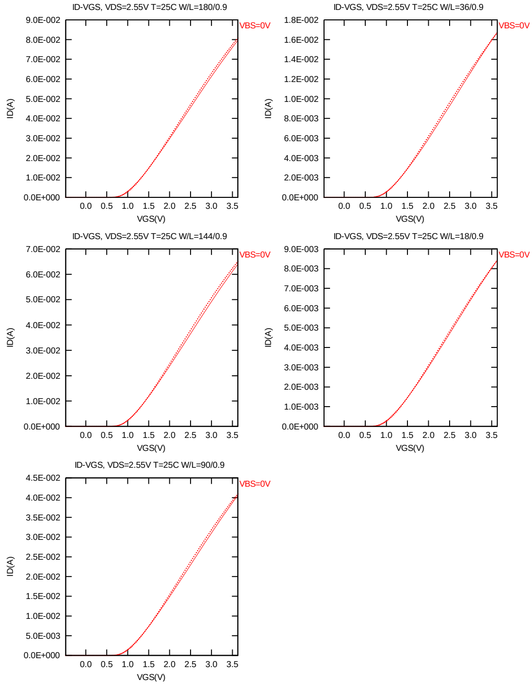
Figure 2-4 I_D vs. V_{GS} at V_{DS} = 2.55 V for NMOS
