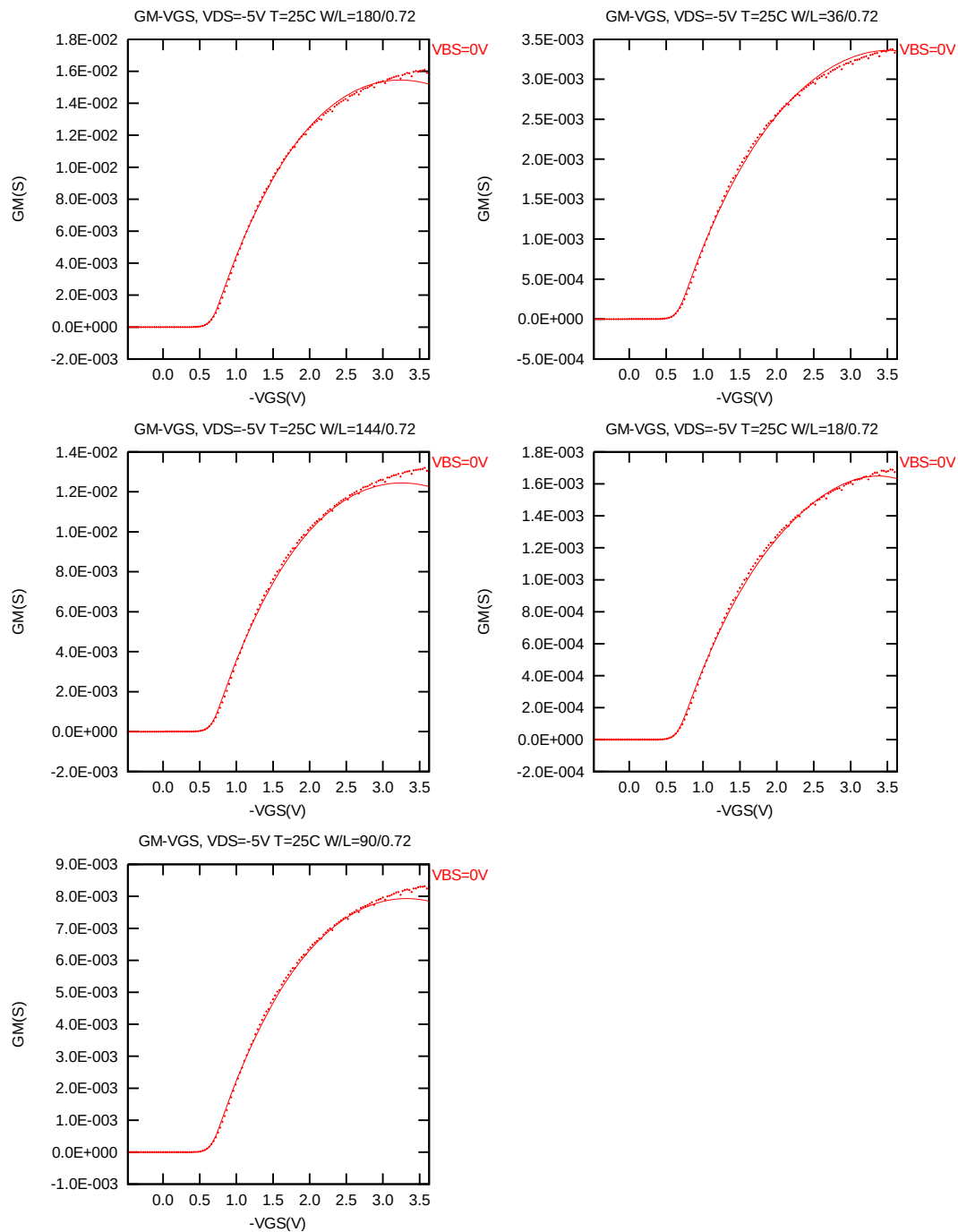
Figure 3-11 G_M vs. V_{GS} at V_{DS} = -5.0 V for PMOS
