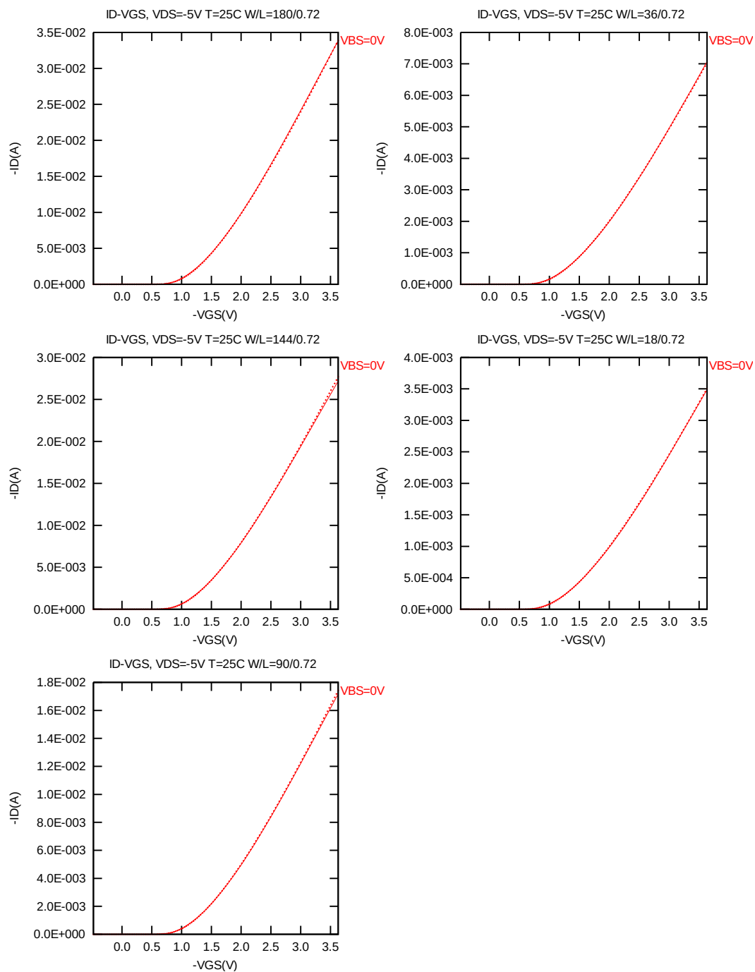
Figure 3-5 I_D vs. V_{GS} at V_{DS} = -5.0 V for PMOS
