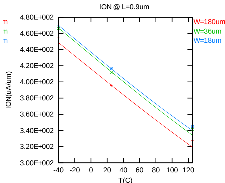
Figure 2-20 Saturation current vs. temperature for NMOS
