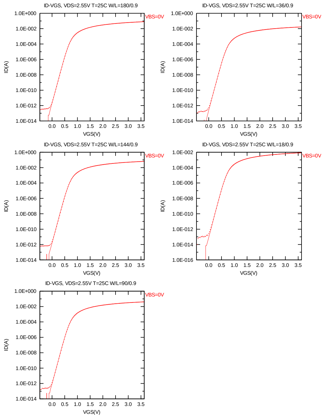
Figure 2-7 Log scaled I_D vs. V_{GS} at V_{DS} = 2.55V for NMOS
