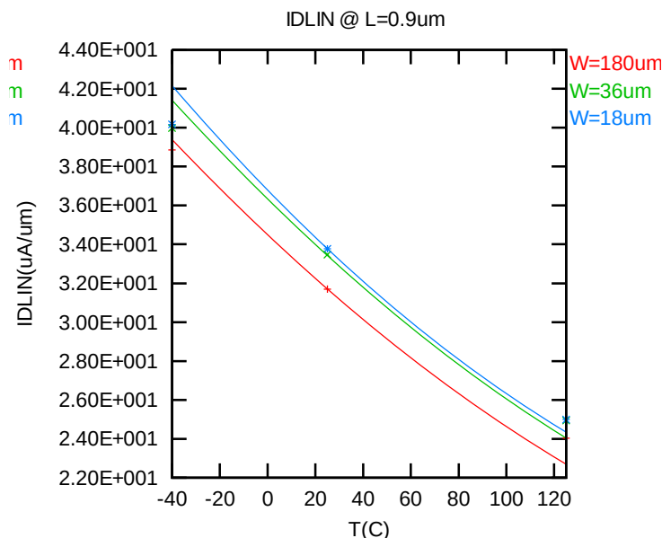
Figure 2-19 Linear current vs. temperature for NMOS
