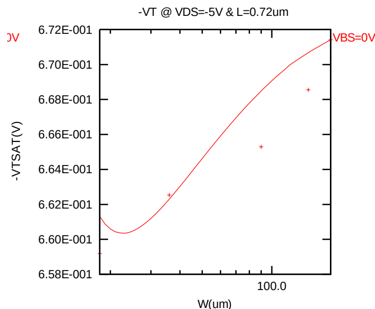
Figure 3-13 V_{TSAT} vs. channel width for high drain bias ( V_{DS} = -5.0 V) for PMOS
