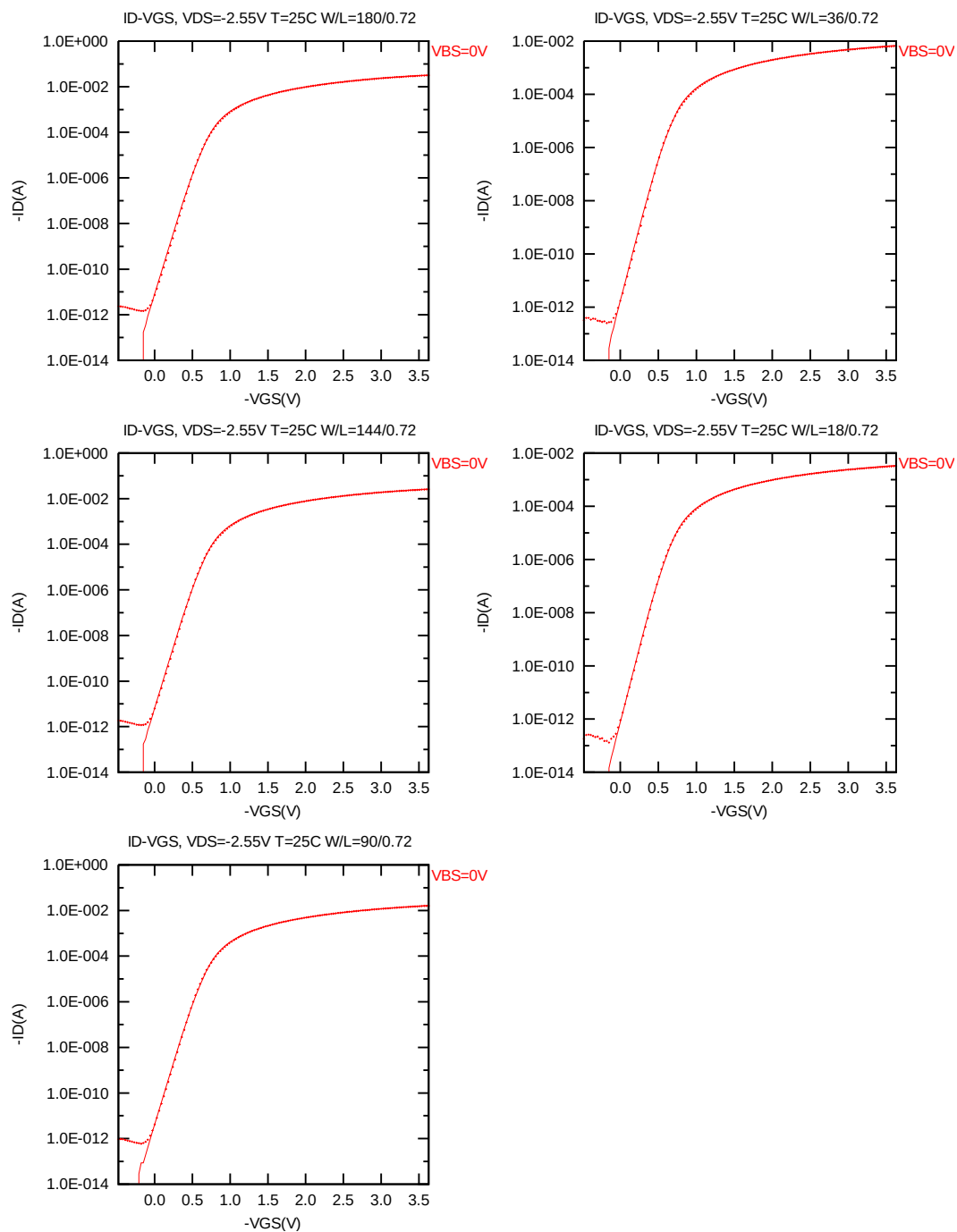
Figure 3-7 Log scaled I_D vs. V_{GS} at V_{DS} = -2.55 V for PMOS
