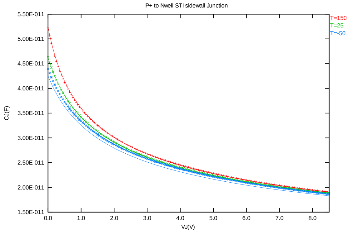
Figure 3-30 STI bounded sidewall junction capacitance at -50^\circ\text{C} , 25^\circ\text{C} and 150^\circ\text{C} for PMOS
