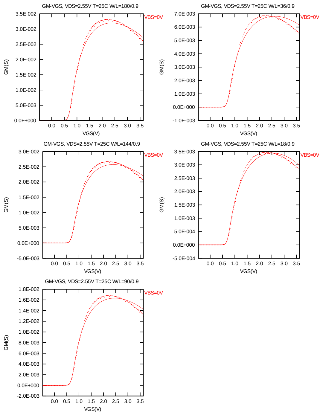
Figure 2-10 G_M vs. V_{GS} at V_{DS} = 2.55 V for NMOS
