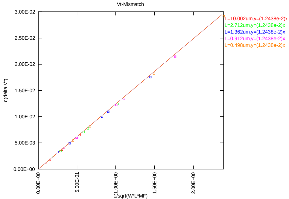
Figure 4-1 V_{TLIN} mis-matching simulation of 5 V n-ch MOSFET
