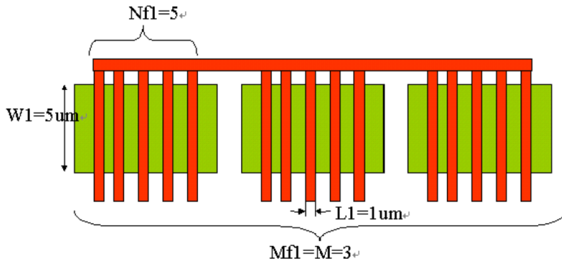
Figure 1-1 Layout Example of parallel devices.
