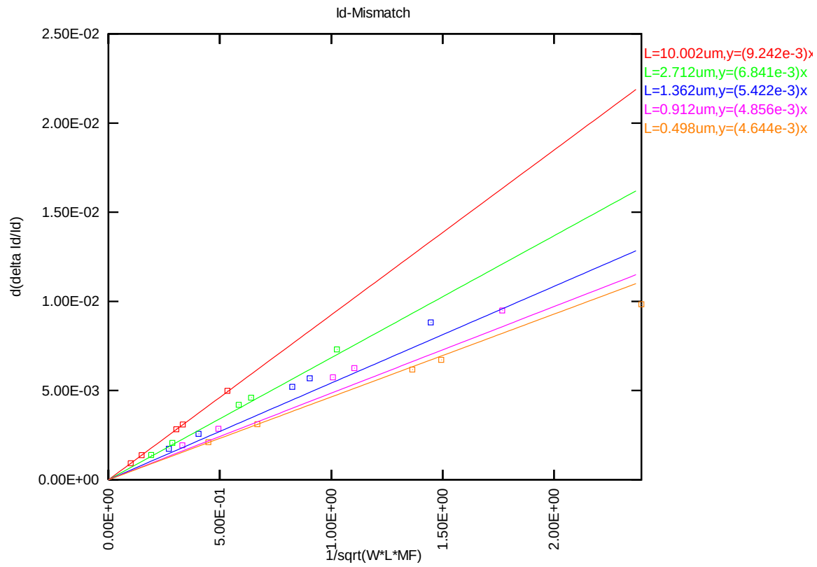
Figure 4-3 I_{DSAT} mis-matching simulation of 5 V n-ch MOSFET
