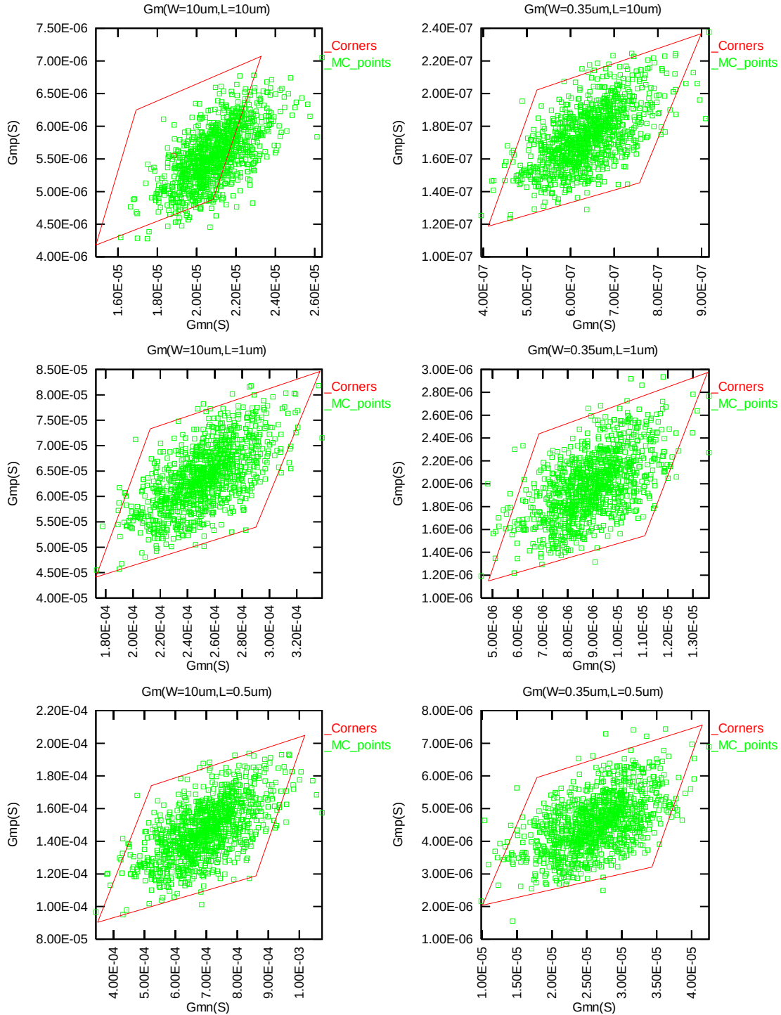
Figure 2-5 Monte Carlo plots of transfer conductance
