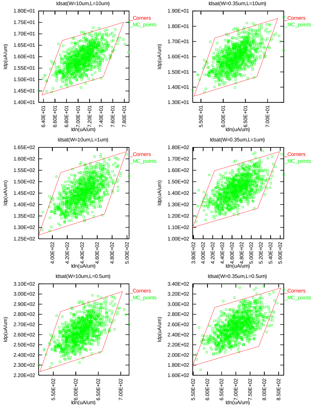
Figure 2-4 Monte Carlo plots of saturation current
