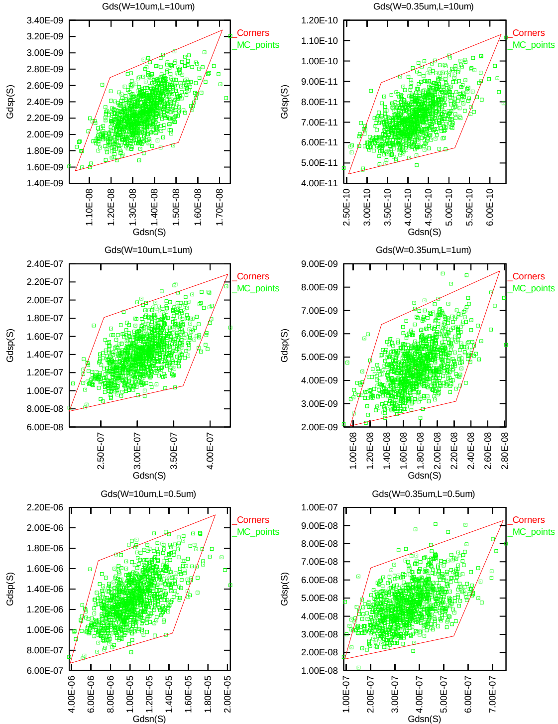
Figure 2-6 Monte Carlo plots of output conductance
