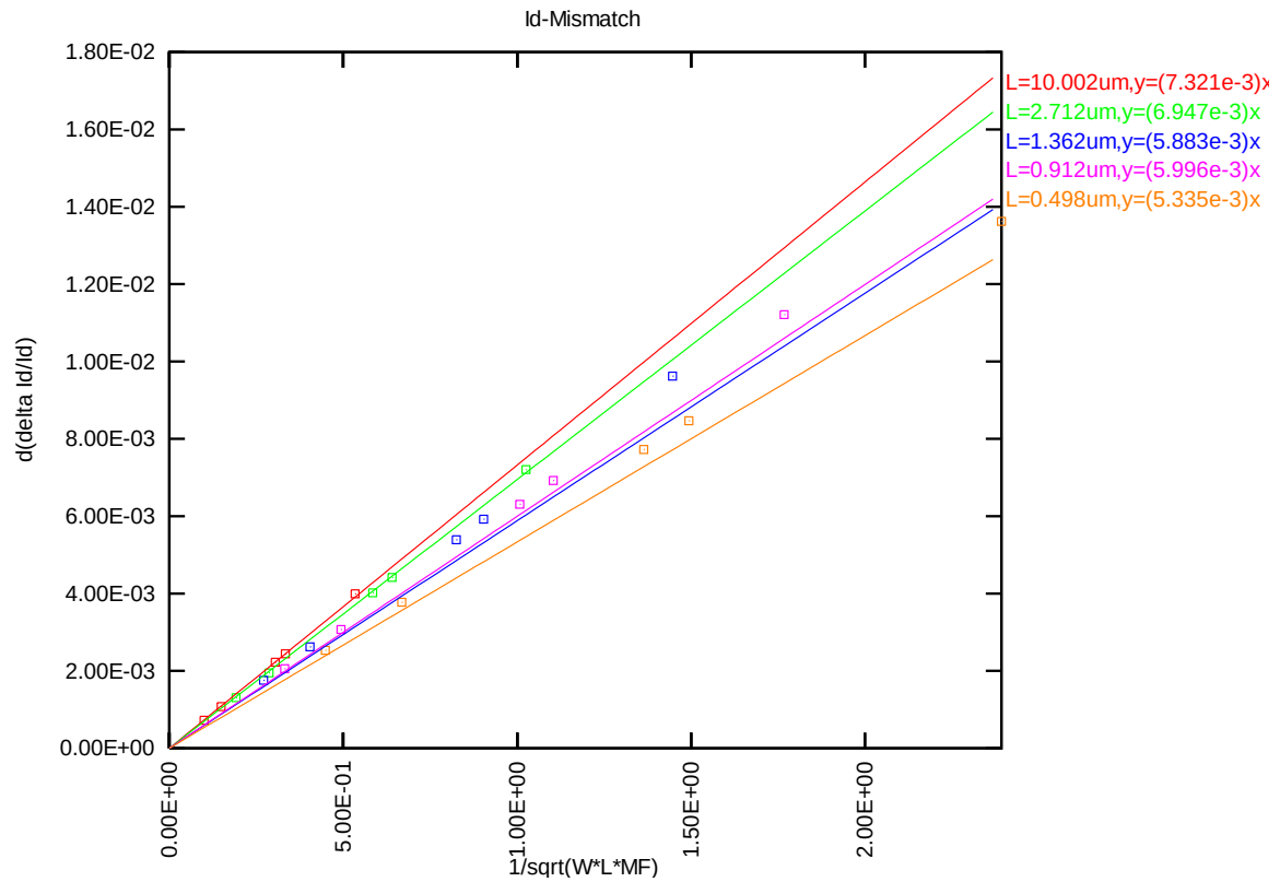
Figure 4-4 I_{\text{DSAT}} mis-matching simulation of 5 V p-ch MOSFET
