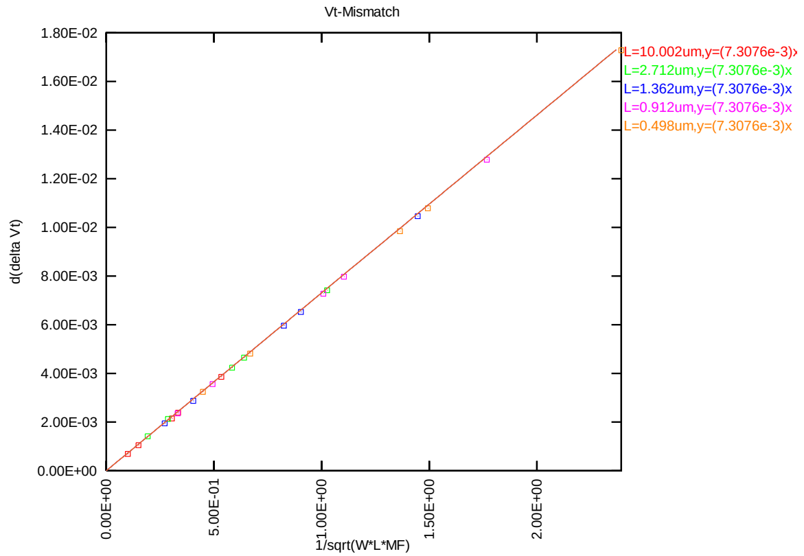
Figure 4-2 V_{TLIN} mis-matching simulation of 5 V p-ch MOSFET
