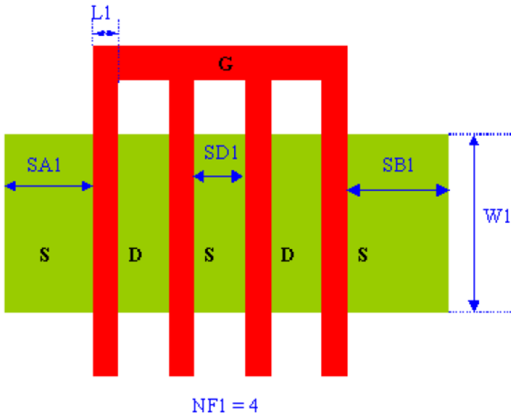
Figure 1-2 Layout Example for LOD effect
