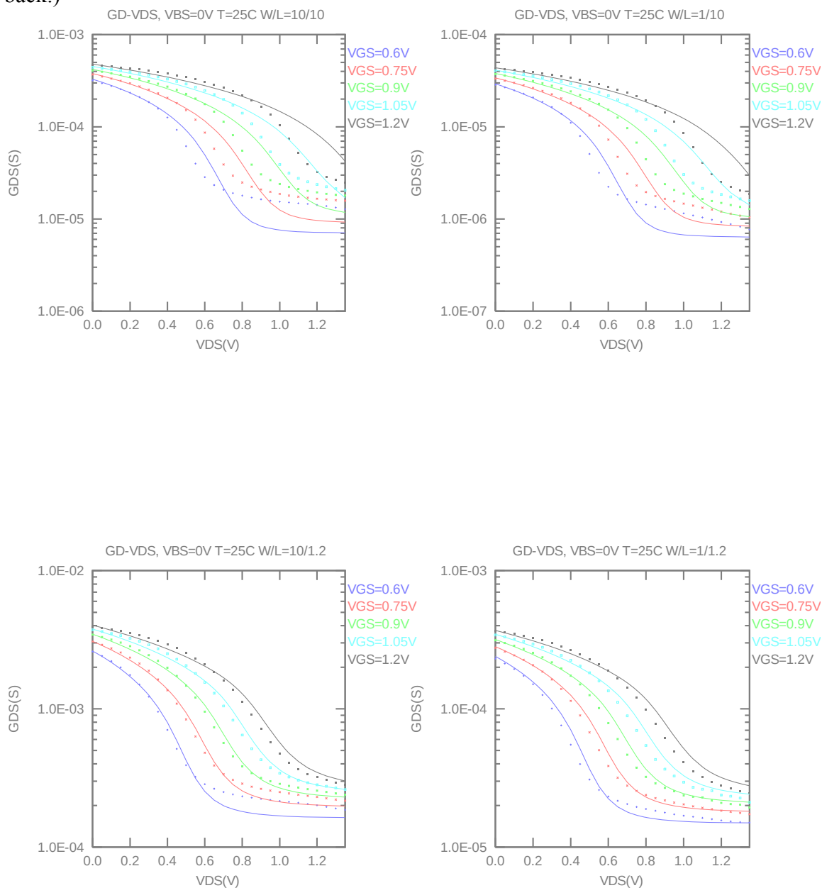
Figure 2-3 G_{DS} vs. V_{DS} at V_{BS} = 0 V for NMOS
