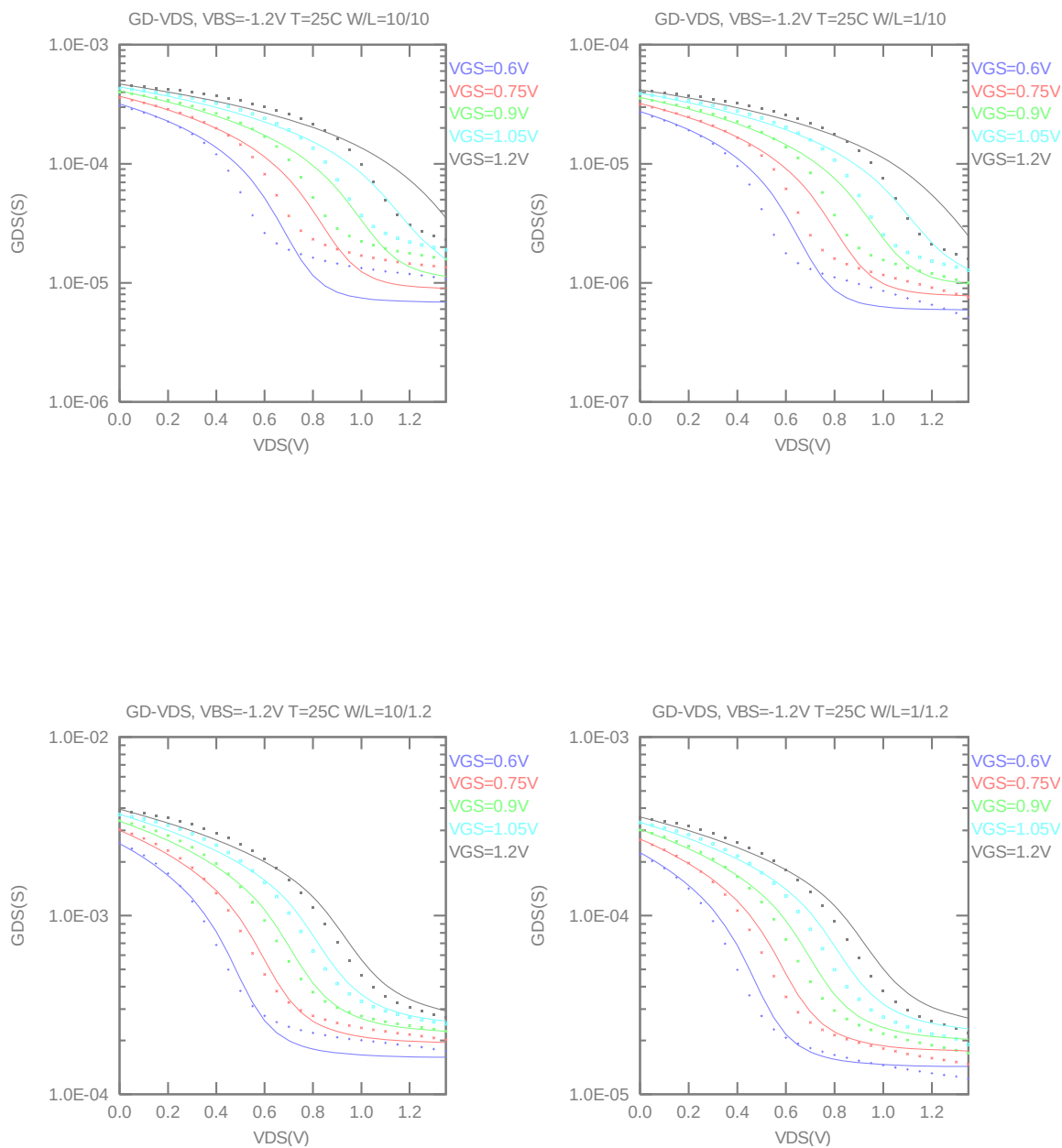
Figure 2-4 G_{DS} vs. V_{DS} at V_{BS} = -1.2V for NMOS
