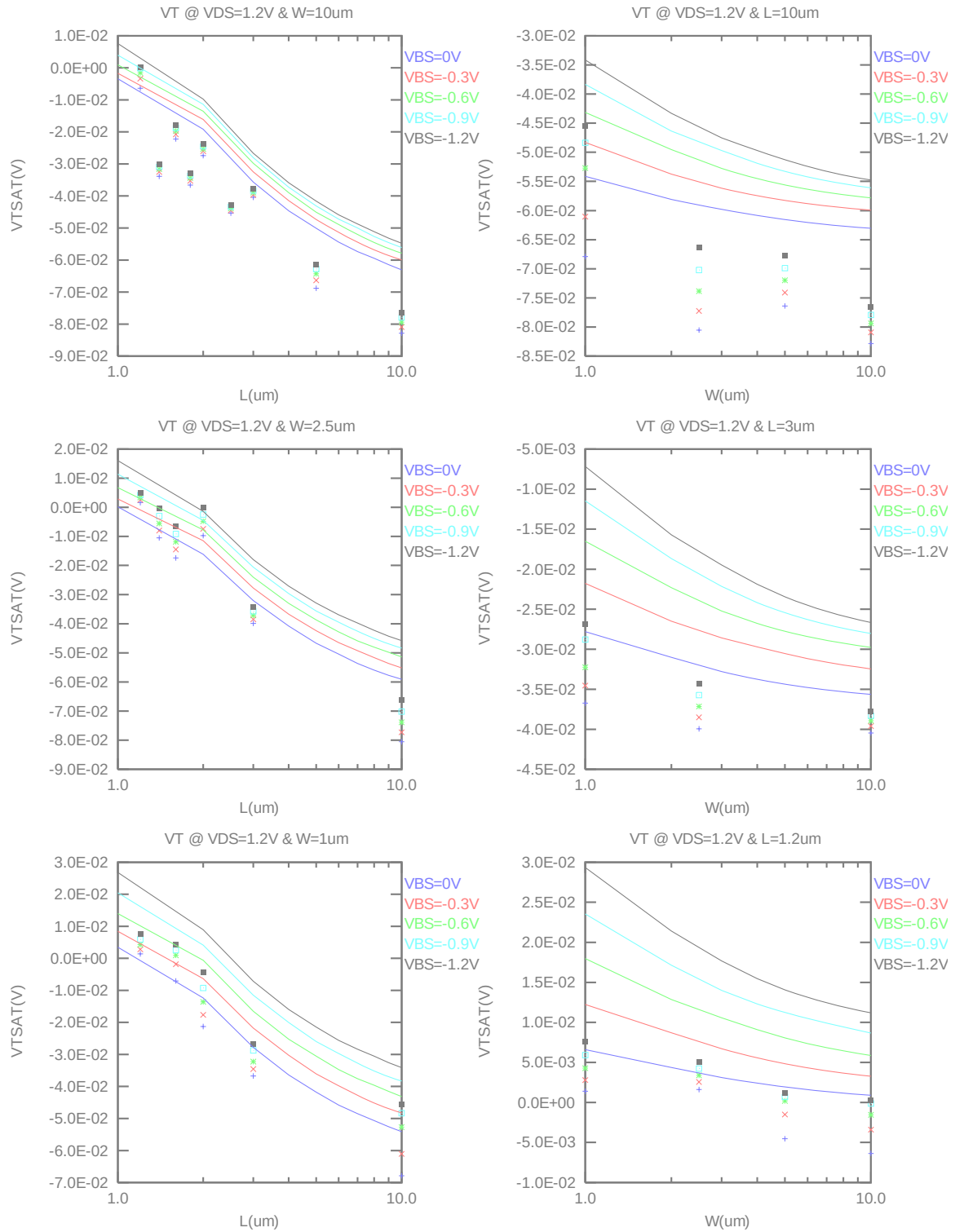
Figure 2-12 V_T vs. channel length & channel width for higt drain bias ( V_{DS} = 1.2V ) for NMOS
