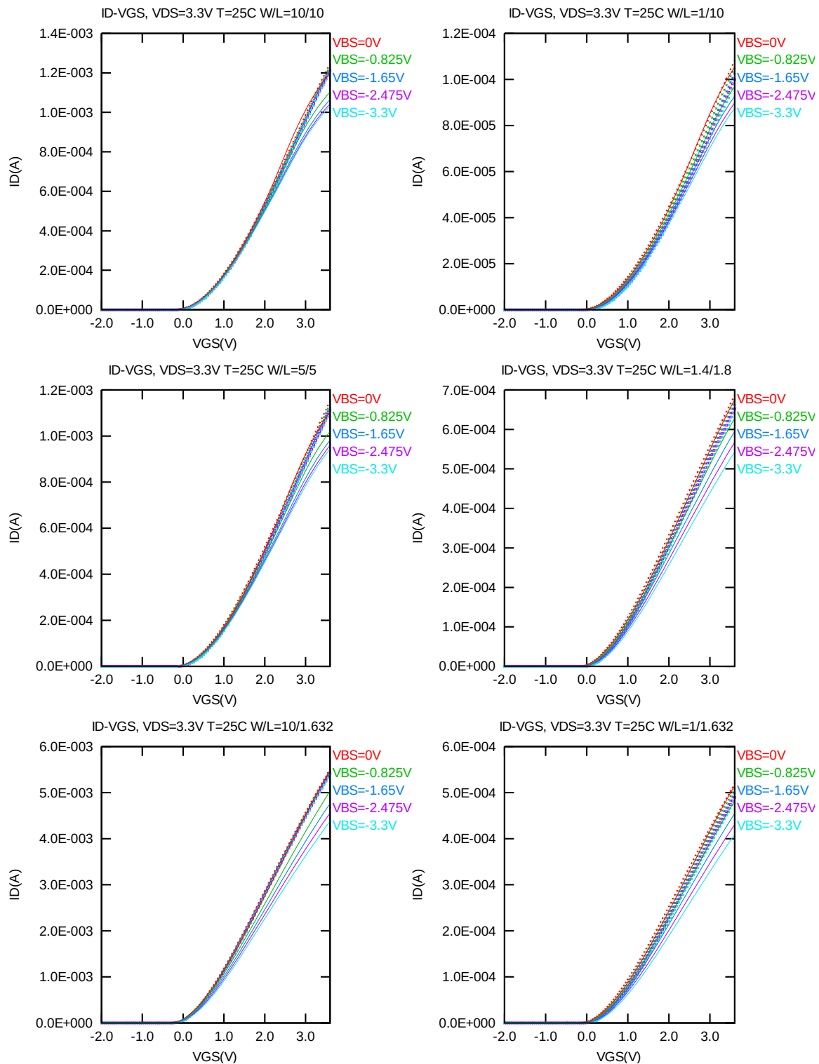
Figure 2-6 I_D vs. V_{GS} at V_{DS}=3.3V for NMOS
