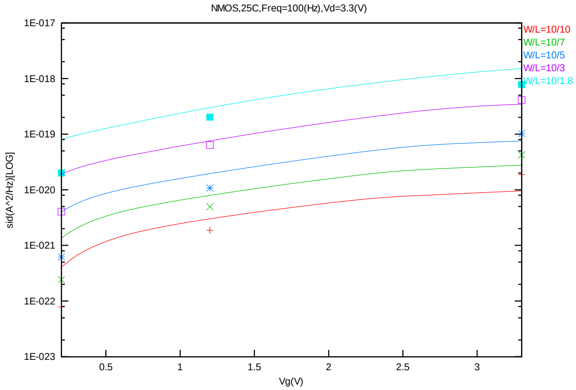
Figure 4-29 Noise vs. V_g for NMOS @ V_d=3.3 V
