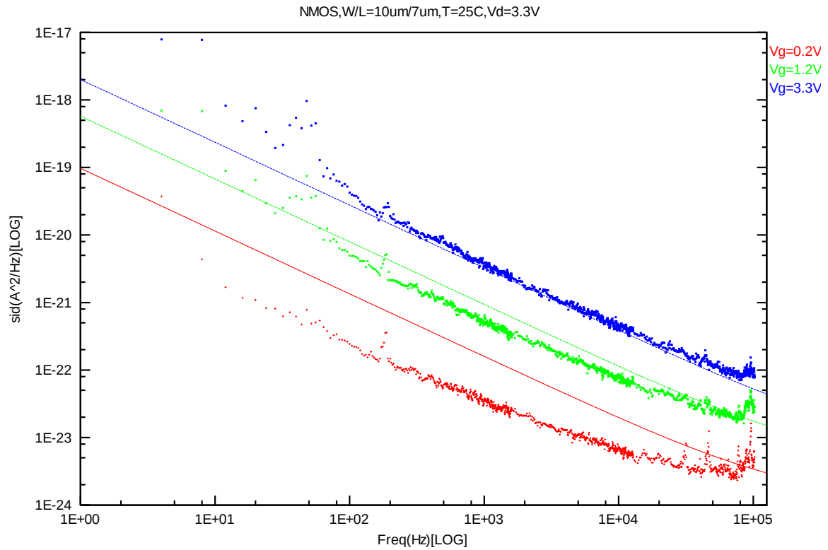
Figure 4-7 NMOS W/L=10um/7um @ Vd=3.3 V
