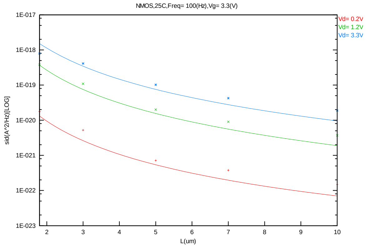
Figure 4-26 Noise vs. Length for NMOS @ Vg=3.3 V
