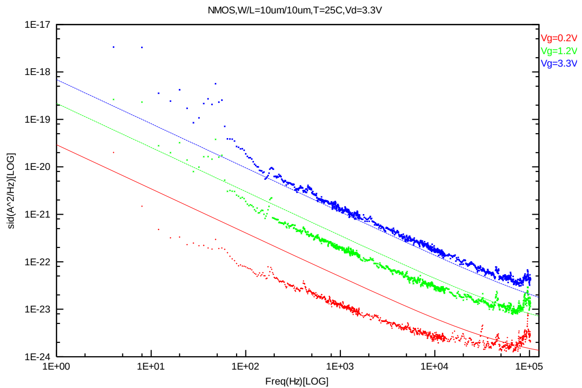
Figure 4-3 NMOS W/L=10um/10um @ Vd=3.3 V
