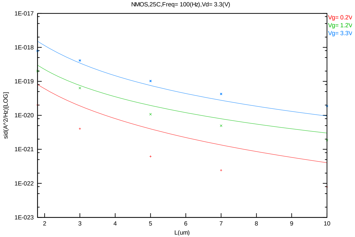
Figure 4-23 Noise vs. Length for NMOS @ Vd=3.3 V
