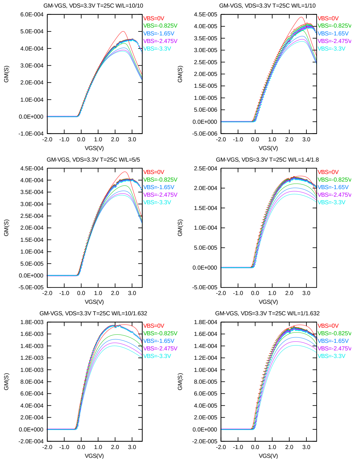
Figure 2-10 G_M vs. V_{GS} at V_{DS}=3.3V for NMOS
