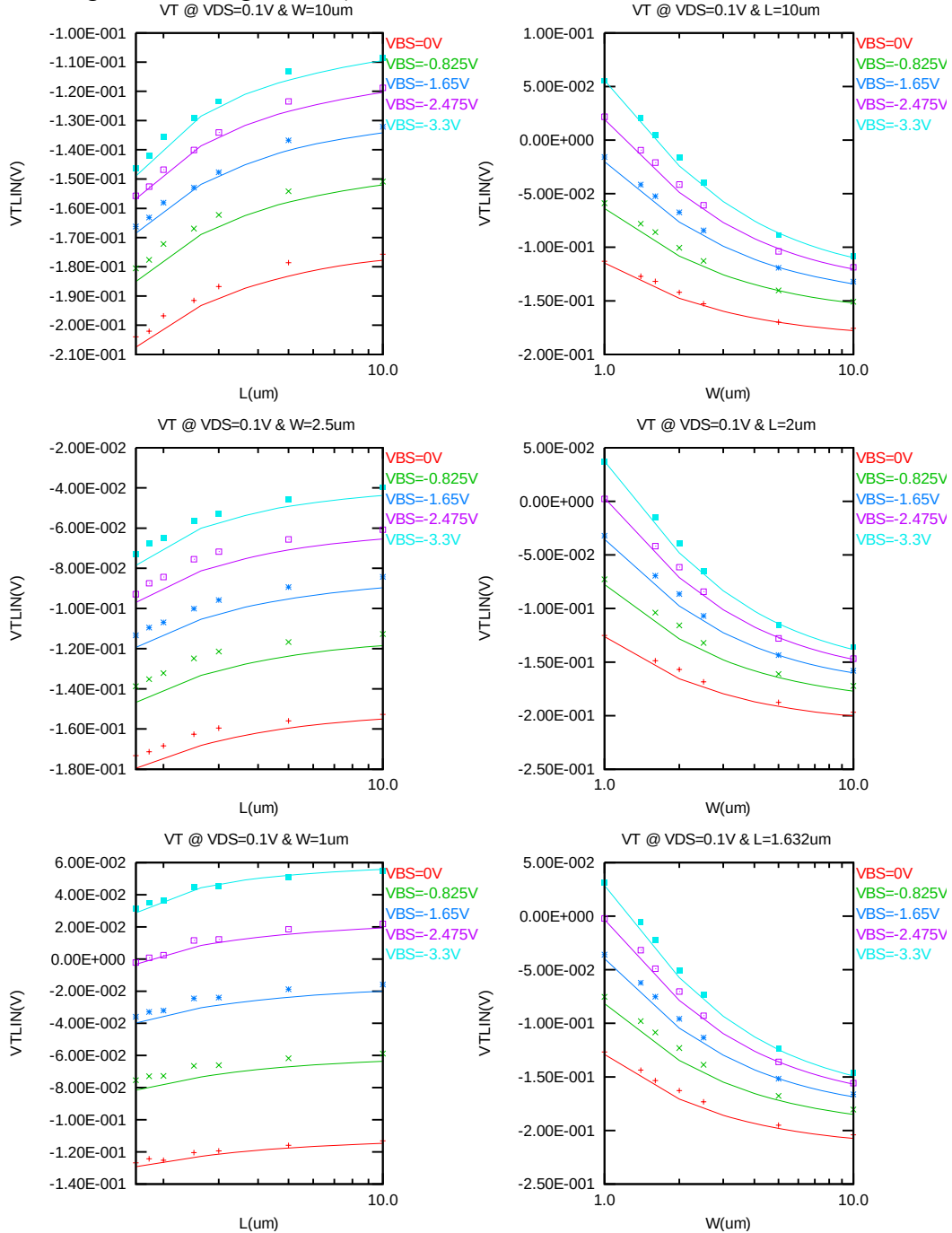
Figure 2-11 V_{TLIN} vs. channel length & channel width for low drain bias ( V_{DS} = 0.1\text{V} ) for NMOS
