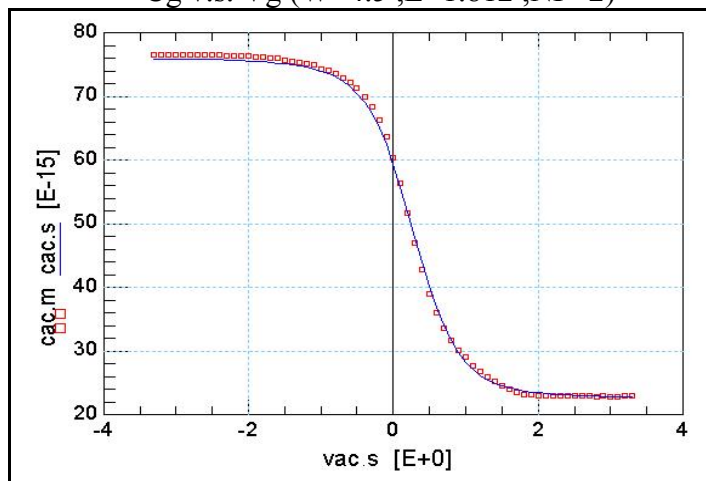
Cg v.s. Vg (W=4.5 ,L=1.812 ,NF=2)
