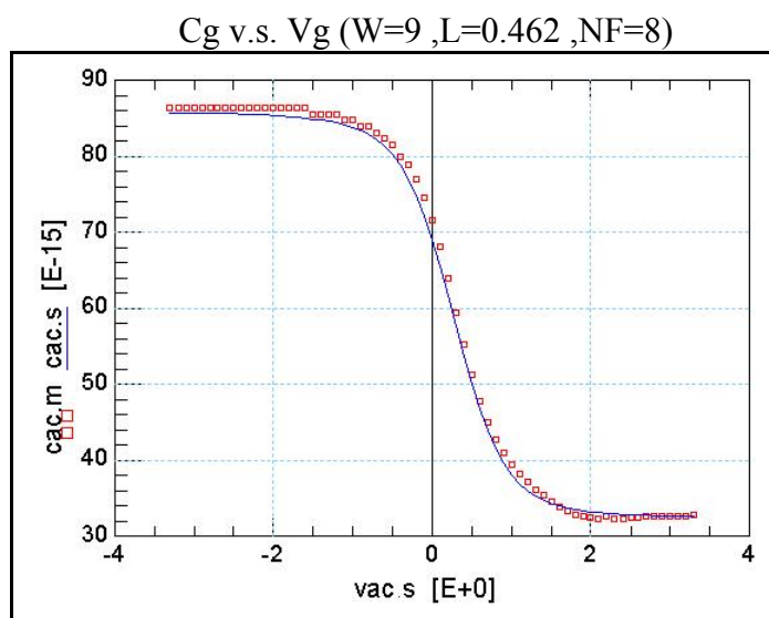
Figure 2-1 Cg vs. Vg at 25 °C
