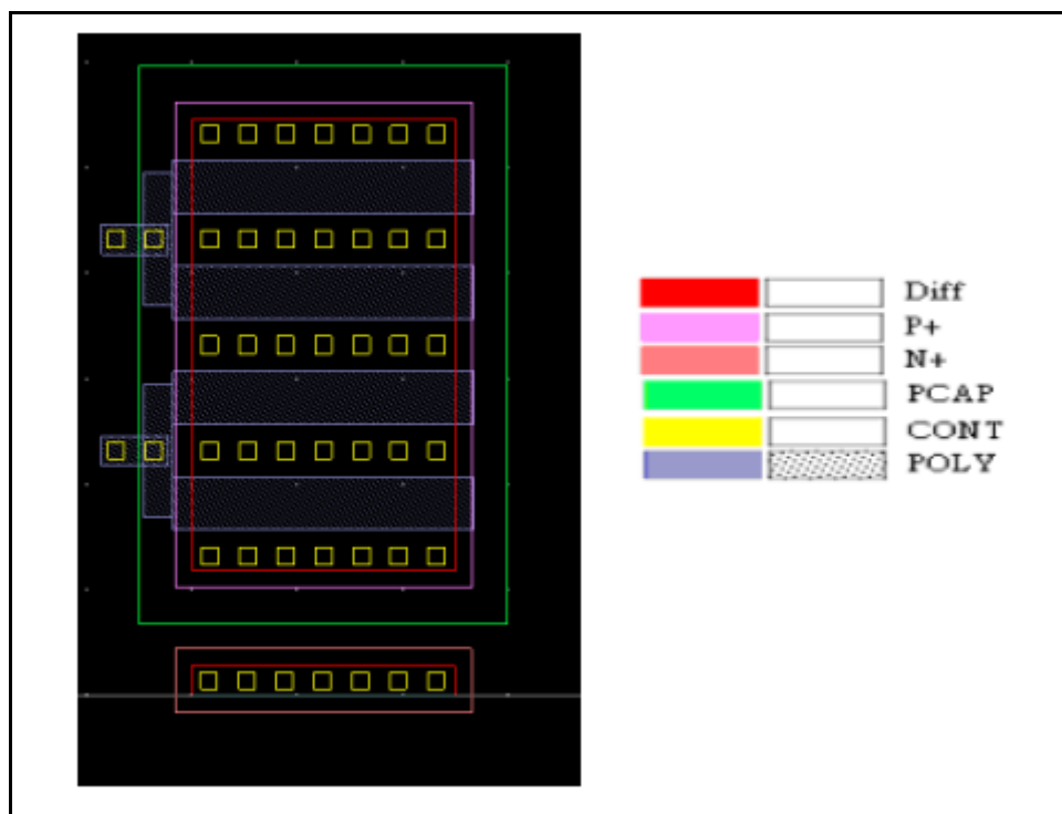
Figure 1-1 PCAP layout
