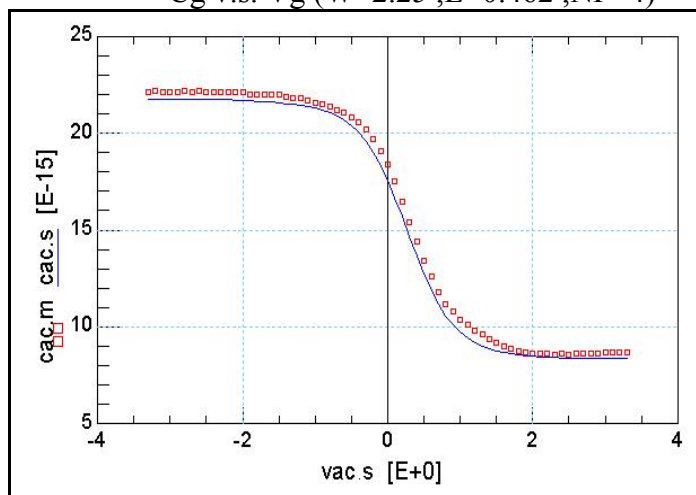
Cg v.s. Vg (W=2.25 ,L=0.462 ,NF=4)
