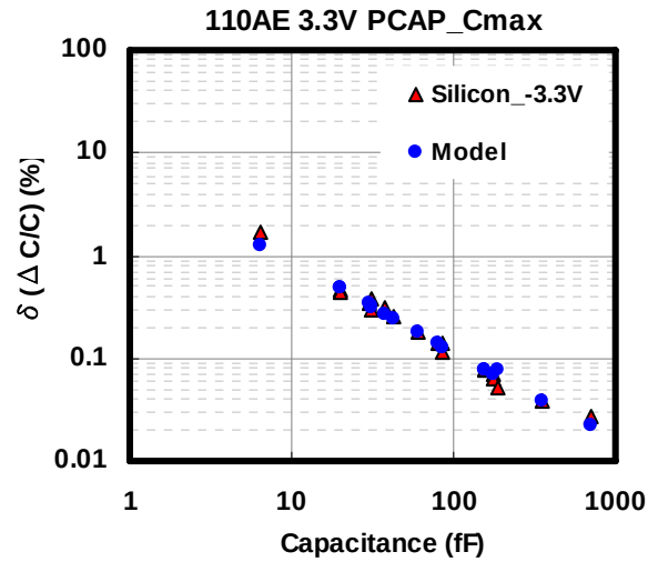
Figure 2-2 Mismatching simulation of PCAP's capacitance
