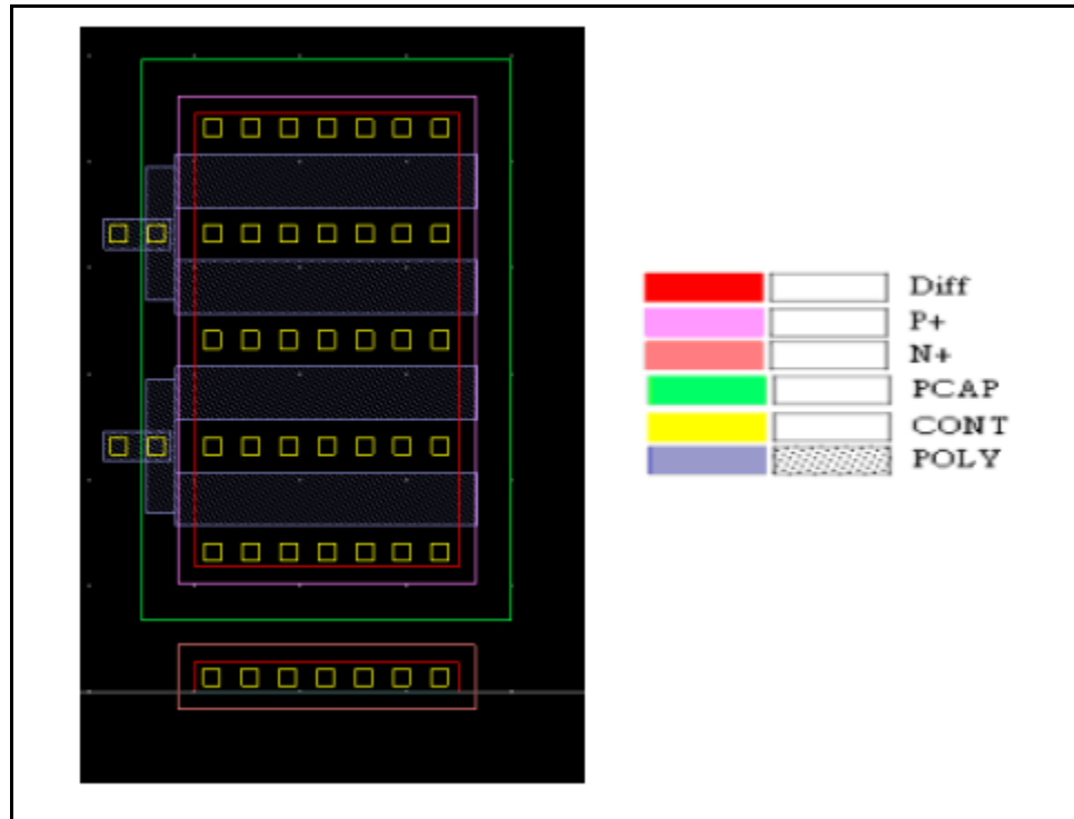
Figure 1-1 PCAP layout
