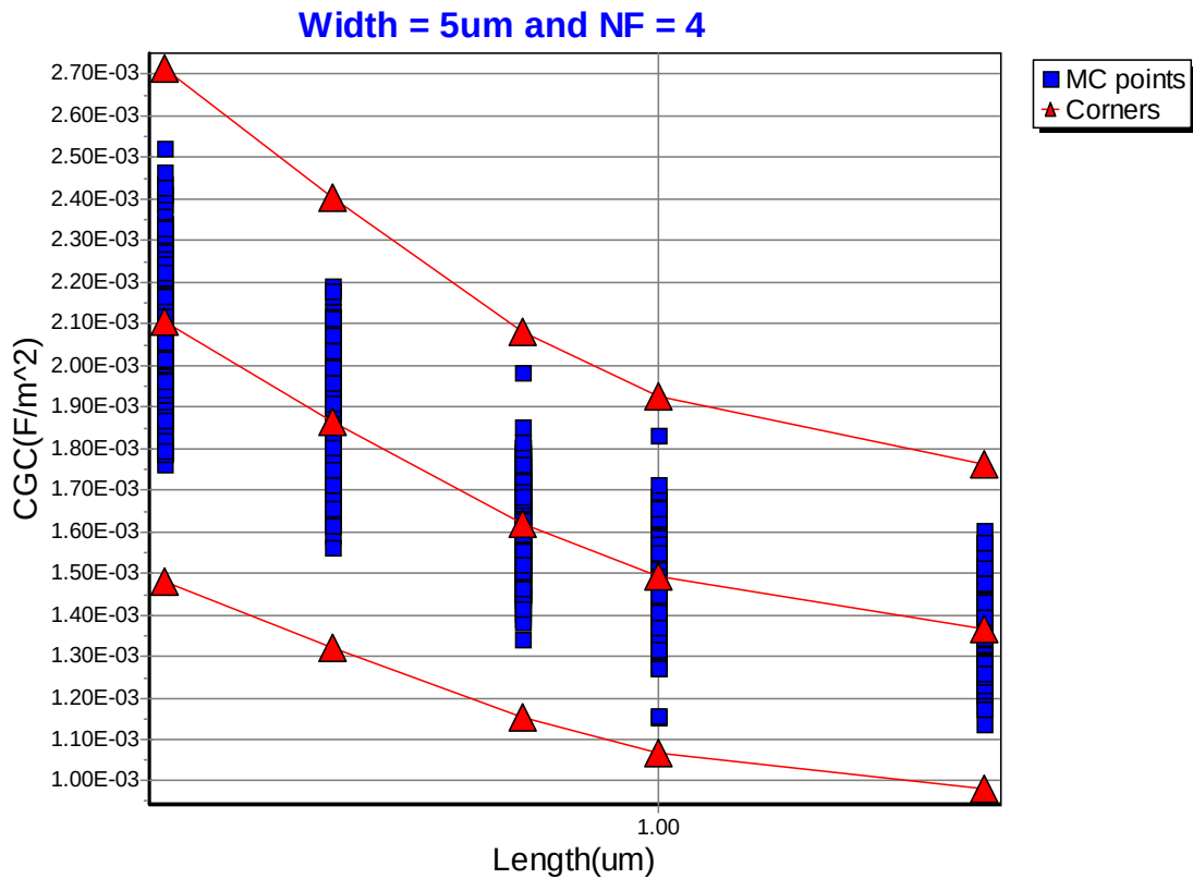
Figure 2-1 Monte Carlo plot of PCAP's capacitance
