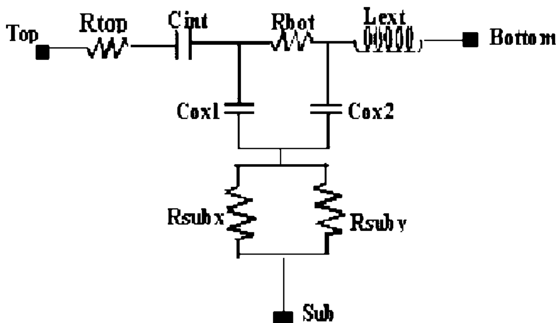
Figure 2-1 Equivalent circuit for mimcaps_1f_psub_rfkf
