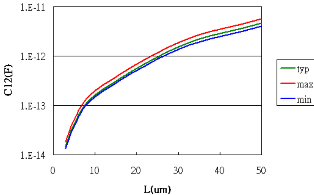
Figure 2-5 Model-predicted main capacitance for 3-corner cases at T=25 °C, frequency=5GHz, W/L ratio is 1, width range is 3um~50um, metal option is 1P8M(mo=26).
