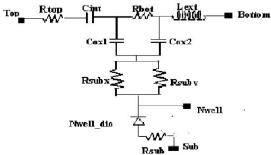
Figure 2-2 Equivalent circuit for mimcaps_2f_nwell_rfkf
