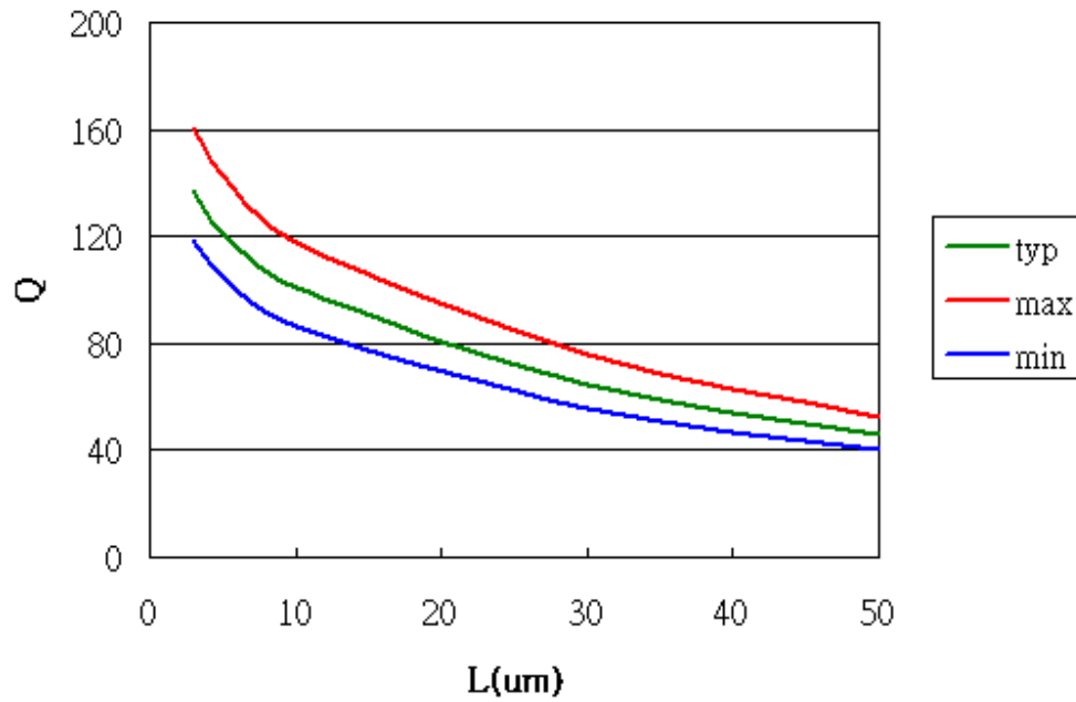
Figure 2-4 Model-predicted Q factor for 3-corner cases at T=25 °C, frequency=5GHz, W/L ratio=1, width range is 3um~50um, metal option is 1P8M(mo=26)
