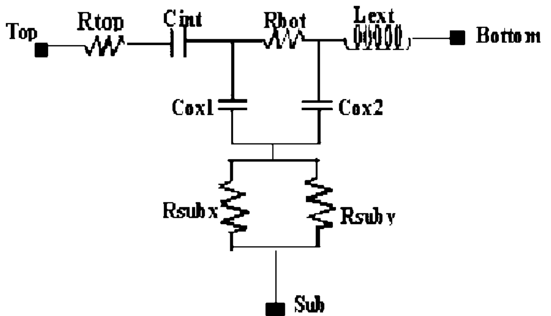
Figure 2-1 Equivalent circuit for mimcaps_2f_psub_rfkf
