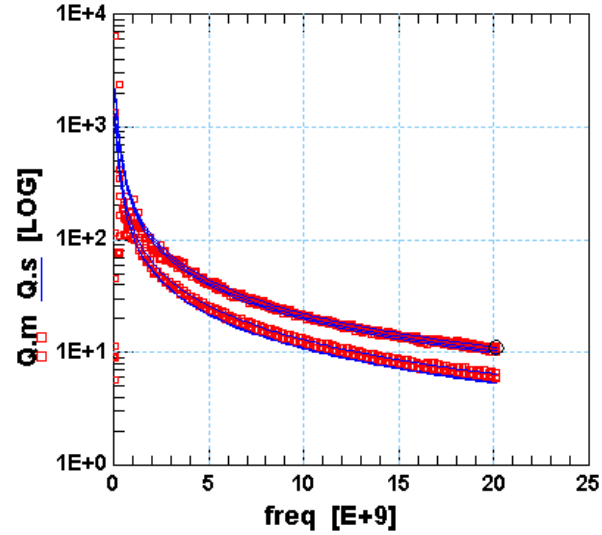
Figure 2-7 VAR_301:Q vs. Freq at V_g = -3.3, -2.2, -1.1, 0, 1.1, 2.2, 3.3 V, V_{nw} = 0 V
