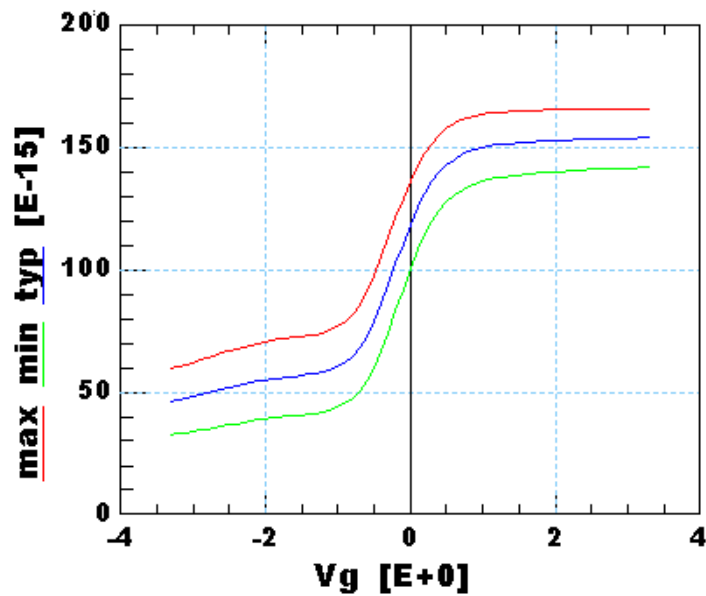
Figure 2-25 VAR_305:Cg vs. Vgb at Freq=5.9GHz
