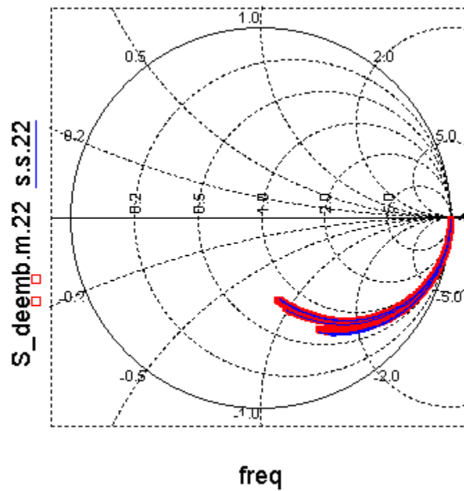
Figure 2-21 VAR_304:S22 at V_g = -3.3V to 3.3V , V_{nw} = 0V , Freq=100MHz to 20.1GHz
