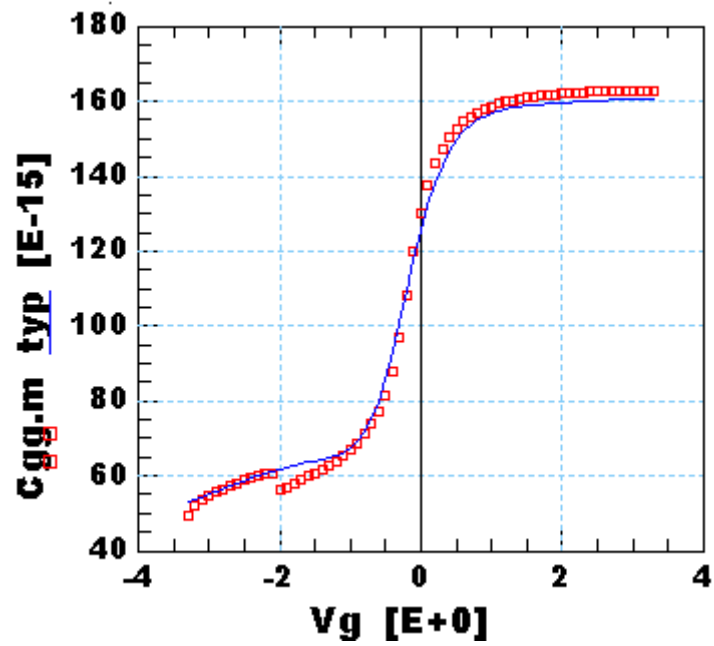
Figure 2-16 VAR_304:Cg vs. Vgb at Freq=5.9GHz
