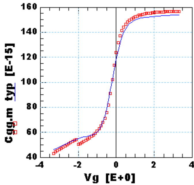
Figure 2-24 VAR_305:Cg vs. Vgb at Freq=5.9 GHz
