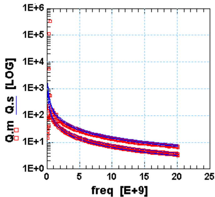
Figure 2-15 VAR_304:Q vs. Freq at Vg=-3.3, -2.2, -1.1, 0, 1.1, 2.2, 3.3 V, Vnw=0 V
