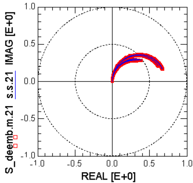
Figure 2-28 VAR_305:S21 at V_g = -3.3\text{V} to 3.3\text{V} , V_{nw} = 0\text{V} , Freq=100MHz to 20.1GHz
