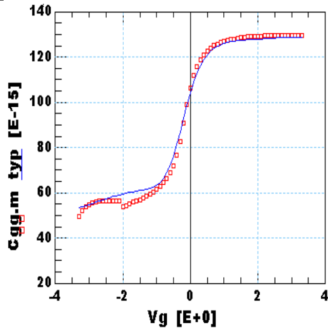
Figure 2-8 VAR_301: C_g vs. V_{gb} at Freq=5.9GHz
