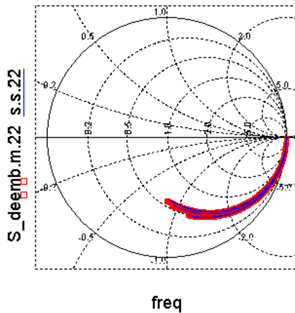
Figure 2-13 VAR_301:S22 at V_g = -3.3V to 3.3V , V_{nw} = 0V , Freq=100MHz to 20.2GHz
