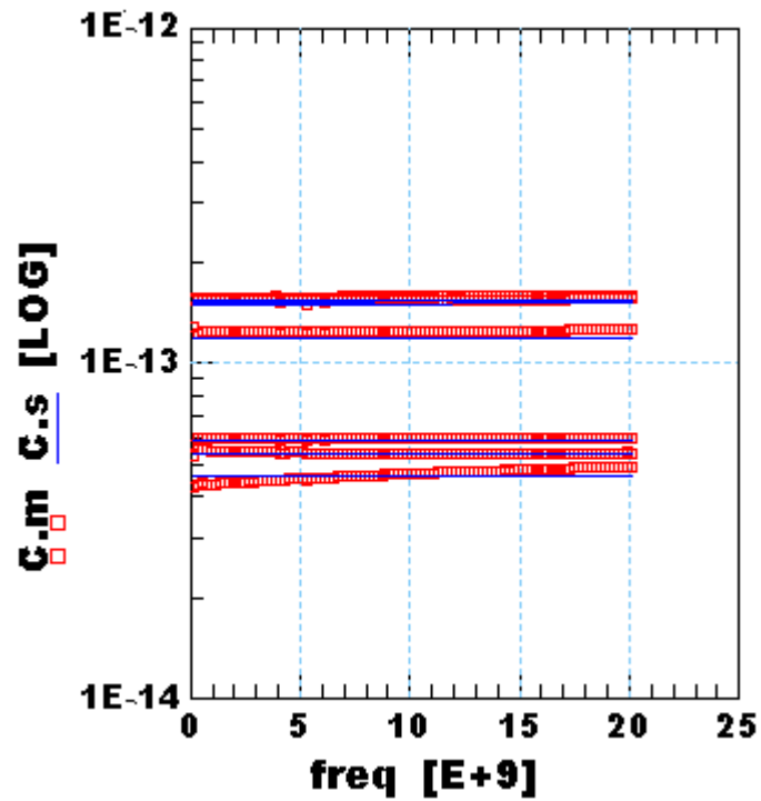
Figure 2-22 VAR_305:Cg vs. Freq at V_g = -3.3, -2.2, -1.1, 0, 1.1, 2.2, 3.3 V, V_{nw} = 0 V
