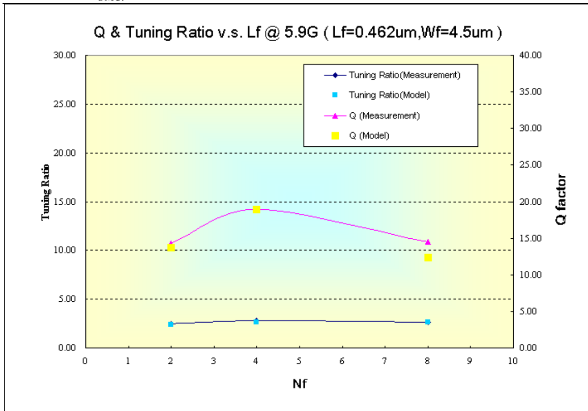
Figure 2-5 Q & Tuning Ratio vs. Nf @ 5.9 GHz
