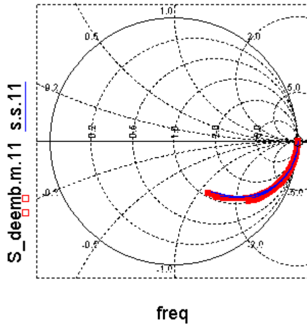
Figure 2-18 VAR_304:S11 at V_g = -3.3V to 3.3V , V_{nw} = 0V , Freq=100MHz to 20.1GHz
