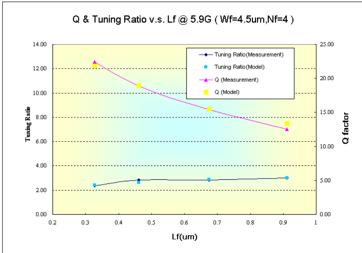
Figure 2-3 Q & Tuning Ratio vs. Lf @ 5.9 GHz
