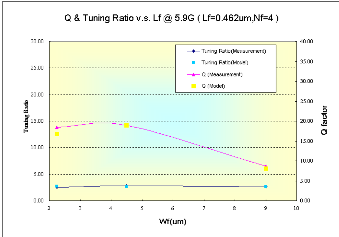
Figure 2-4 Q & Tuning Ratio vs. Wf @ 5.9 GHz
