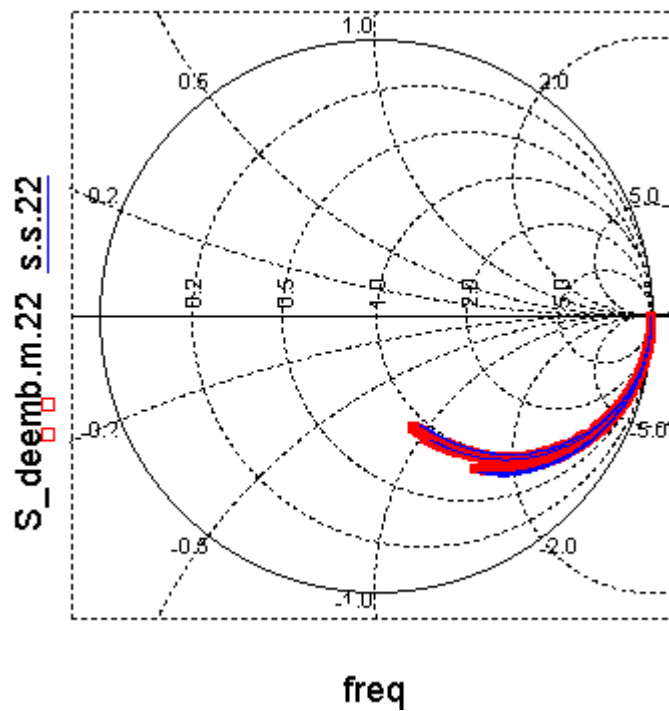
Figure 2-29 VAR_305:S22 at V_g = -3.3\text{V} to 3.3\text{V} , V_{nw} = 0\text{V} , Freq=100MHz to 20.1GHz
