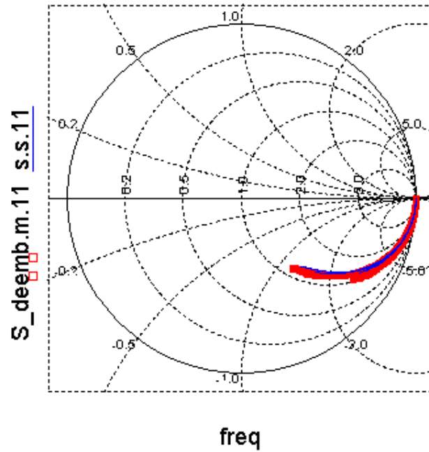
Figure 2-26 VAR_305:S11at V_g = -3.3V to 3.3V , V_{nw} = 0V , Freq=100MHz to 20.1GHz
