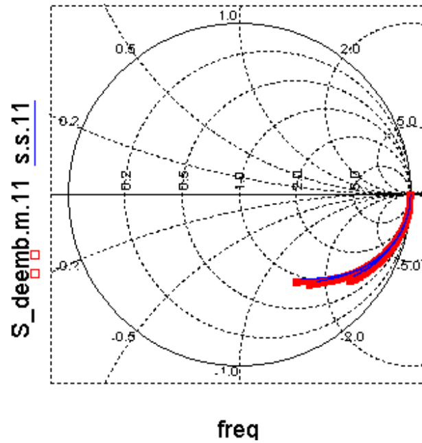
Figure 2-10 VAR_301:S11 at V_g = -3.3V to 3.3V , V_{nw} = 0V , Freq=100MHz to 20.1GHz
