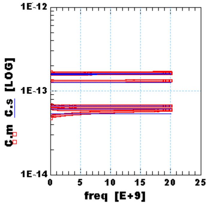
Figure 2-14 VAR_304:Cg vs. Freq at Vg=-3.3, -2.2, -1.1, 0, 1.1, 2.2, 3.3 V, Vnw=0 V
