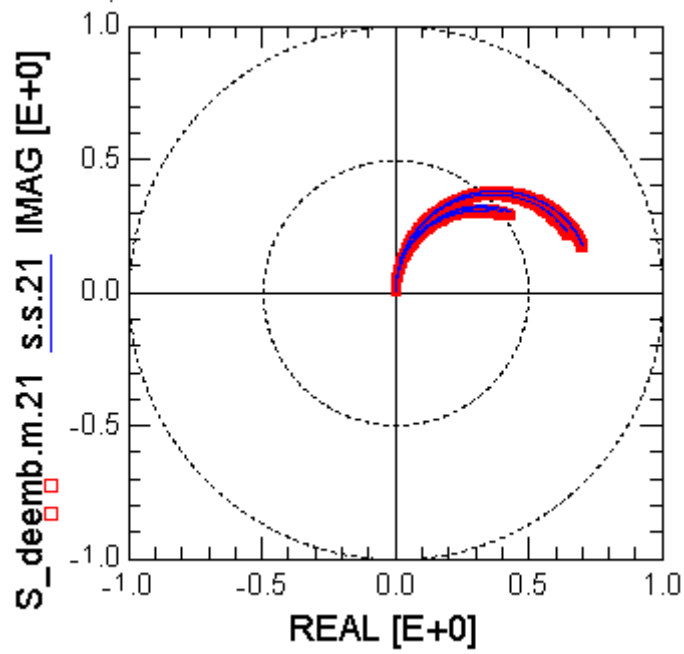
Figure 2-20 VAR_304:S21at V_g = -3.3V to 3.3V , V_{nw} = 0V , Freq=100MHz to 20.1GHz
