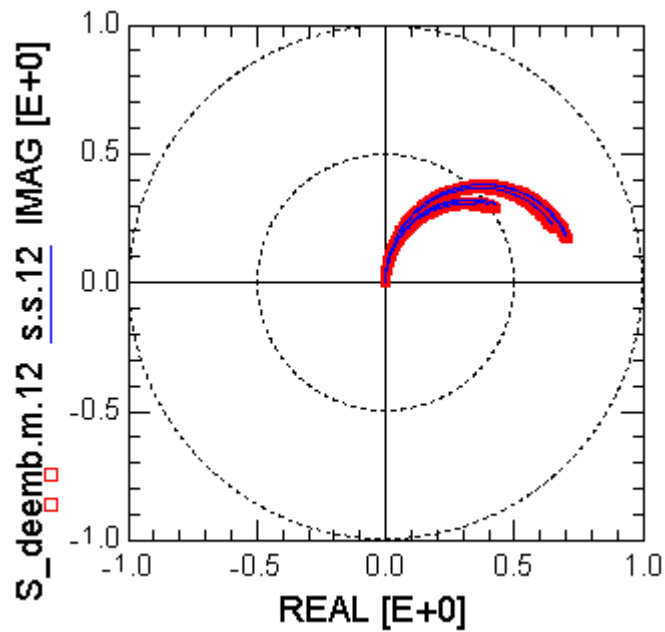
Figure 2-19 VAR_304:S12 at V_g = -3.3V to 3.3V , V_{nw} = 0V , Freq=100MHz to 20.1GHz
