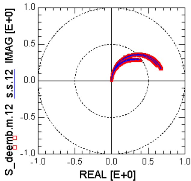
Figure 2-27 VAR_305:S12 at V_g = -3.3V to 3.3V , V_{nw} = 0V , Freq=100MHz to 20.1GHz
