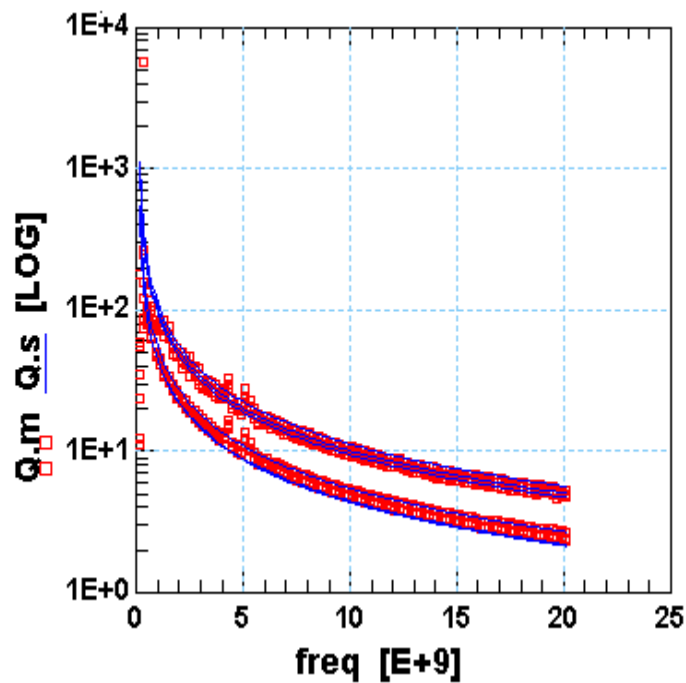
Figure 2-23 VAR_305:Q vs. Freq at V_g = -3.3, -2.2, -1.1, 0, 1.1, 2.2, 3.3 V, V_{nw} = 0 V
