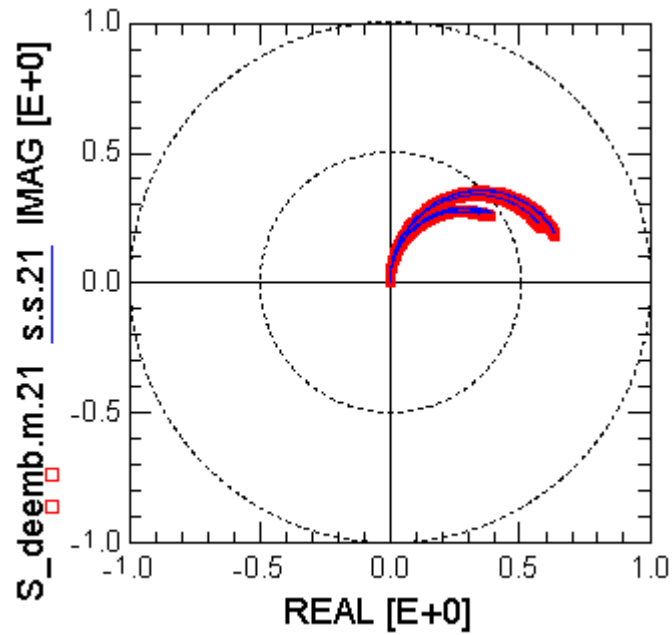
Figure 2-12 VAR_301:S21 at V_g = -3.3V to 3.3V , V_{nw} = 0V , Freq=100MHz to 20.1GHz
