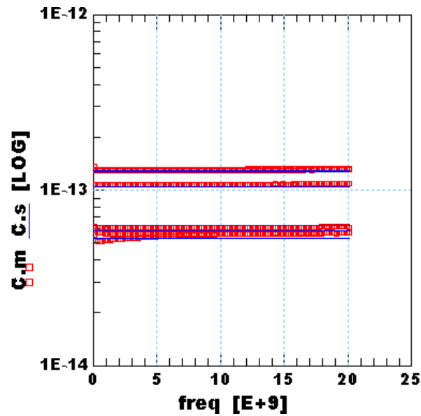
Figure 2-6 VAR_301:Cg vs. Freq at V_g = -3.3, -2.2, -1.1, 0, 1.1, 2.2, 3.3 V, V_{nw} = 0 V
