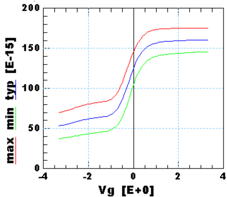
Figure 2-17 VAR_304:Cg vs. Vgb at Freq=5.9GHz
