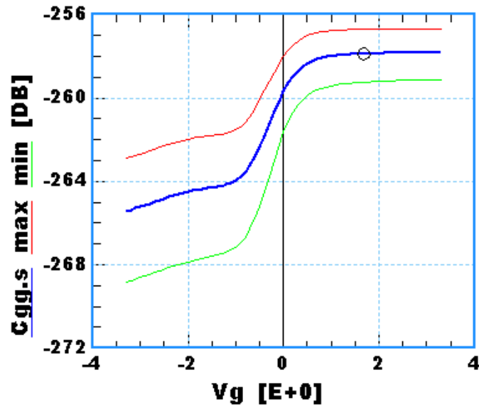
Figure 2-9 VAR_301: C_g vs. V_{gb} at Freq=5.9GHz for center model
