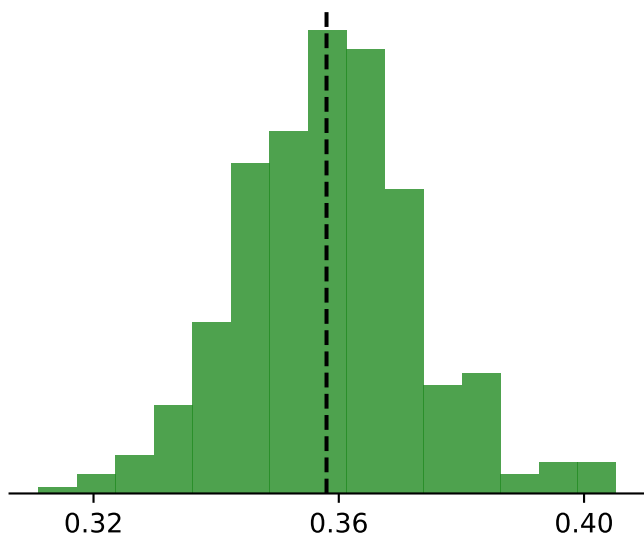
Odds-ratio state effects
