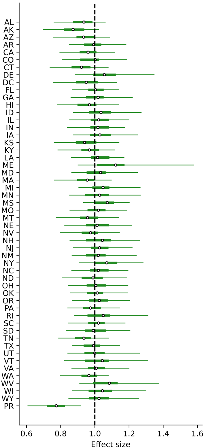
Odds-ratio state effects
