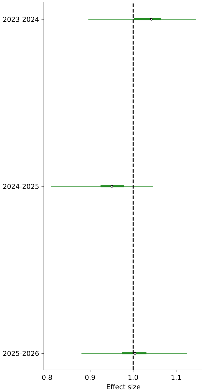
Odds-ratio season effects
