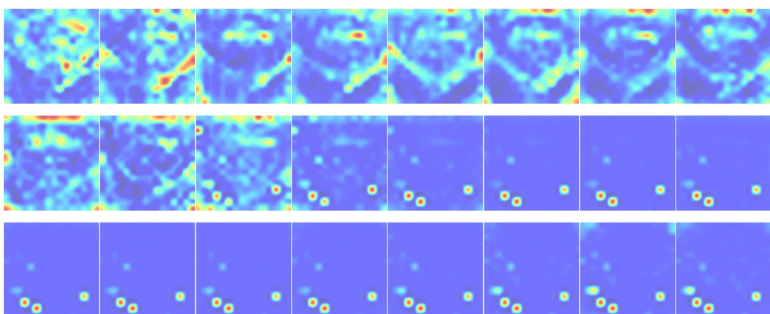
Original CLIP
