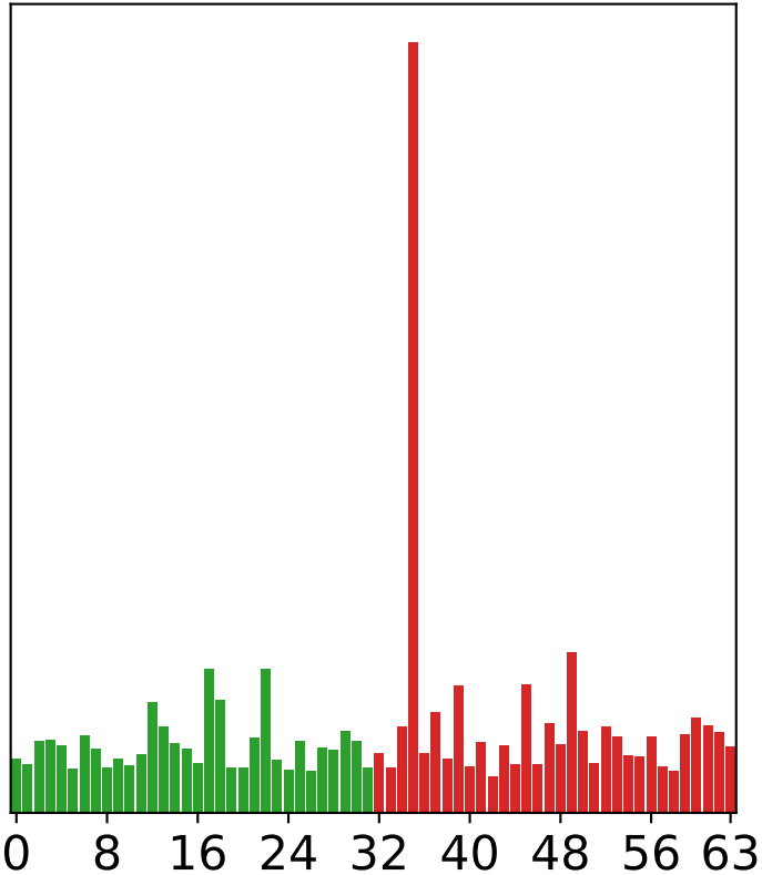
Attention Score on Prototypes
