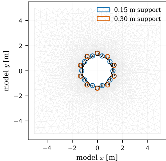
ERT support geometry
