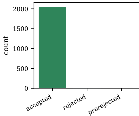
Trace decisions
