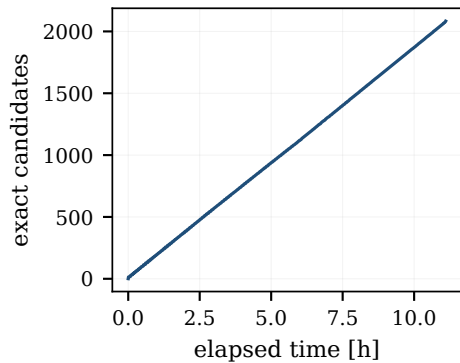
Candidate production
