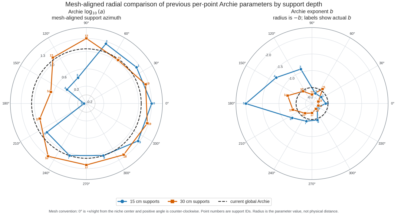
Figure 8: Mesh-aligned radial comparison of previous per-support Archie parameters against the current global Archie reference. The polar angle follows the support-table convention: 0^\circ is positive mesh x from the niche center and angles increase counter-clockwise.
