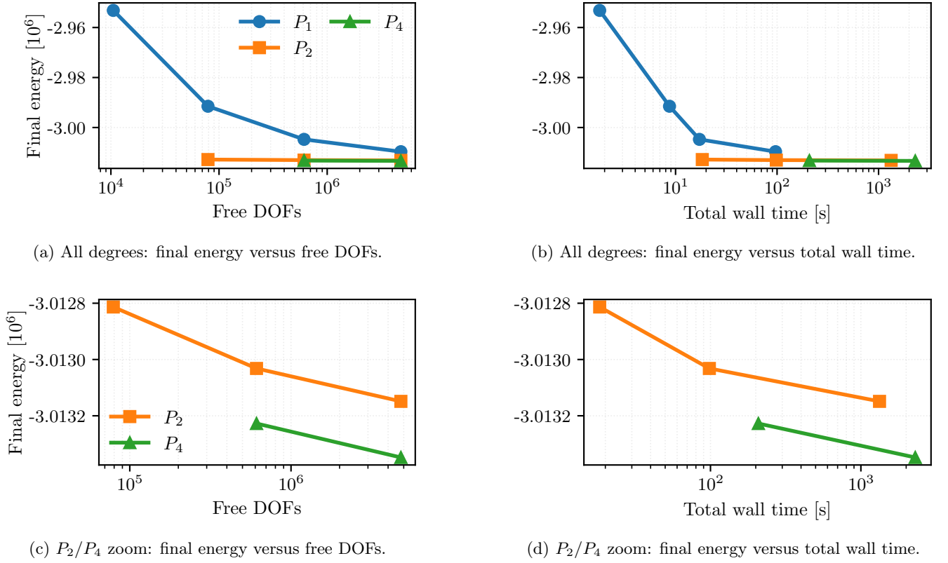
Figure 26: Bottom-clamped 3D plasticity degree-versus-resolution study at \lambda_{sr} = 1.55 . The top panels show the full P_1/P_2/P_4 comparison, while the bottom panels zoom to P_2/P_4 so the near-overlap hidden by the coarse P_1 points becomes visible. The left column plots final values of (33) against free DOFs; the right column plots the same converged energies against end-to-end wall time. All timings use the same 32-rank configuration.
