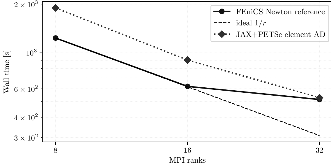
Figure 23: Hyperelasticity strong scaling for the 24-step load path defined by (16).
