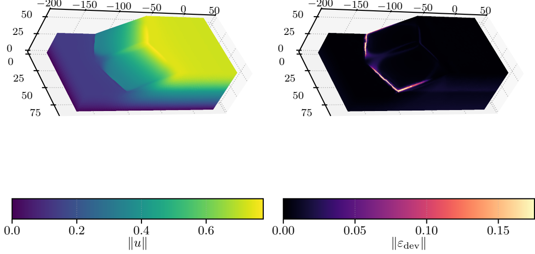
Figure 14: Bottom-clamped 3D plasticity representative endpoint at \lambda_{\text{sr}} = 1.55 : displacement magnitude and surface deviatoric strain for the P_4(L_2) configuration, both derived from the scalar surrogate in (33).
