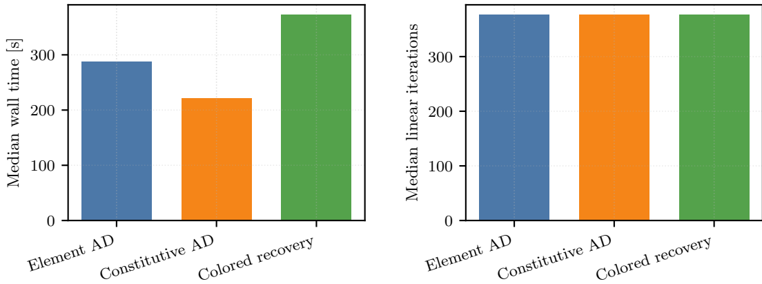
Figure 25: Fixed 3D plasticity derivative-route comparison on P_4(L_1) , \lambda_{\text{sr}} = 1.5 , and 8 MPI ranks.
