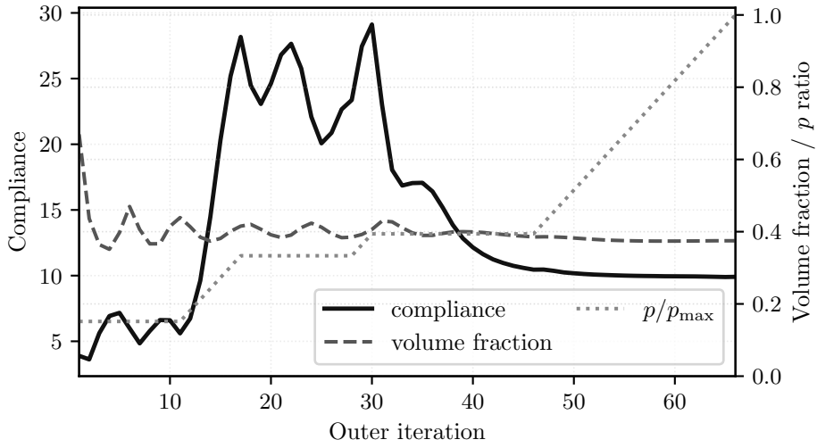
Figure 18: Objective-history view for the frozen reduced topology objective (37), with compliance on the left axis and volume fraction plus the continuation schedule in p on the right axis.
