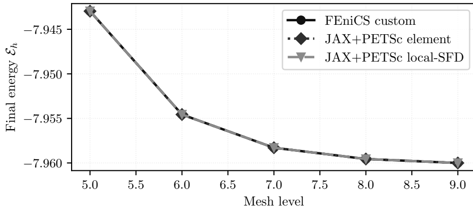
Figure 7: Final discrete energies from equation (6) across the selected mesh hierarchy. The element-AD and local-SFD JAX+PETSc paths are essentially energy-consistent with the FEniCS reference.
