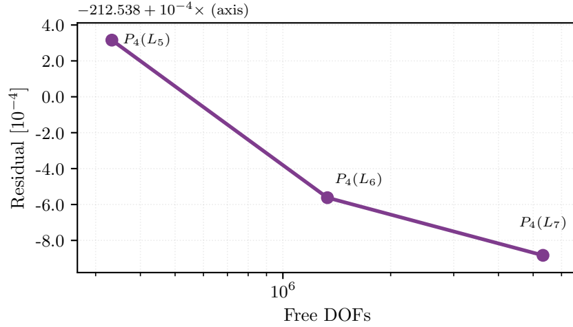
Figure 13: Resolution trend for the Plasticity2D family. The plotted terminal energies are evaluations of equation (19) on the completed P_4(L_5) endpoint case and on the larger 20-iteration capped P_4(L_6) and P_4(L_7) diagnostics, which are not used as endpoint-convergence evidence.
