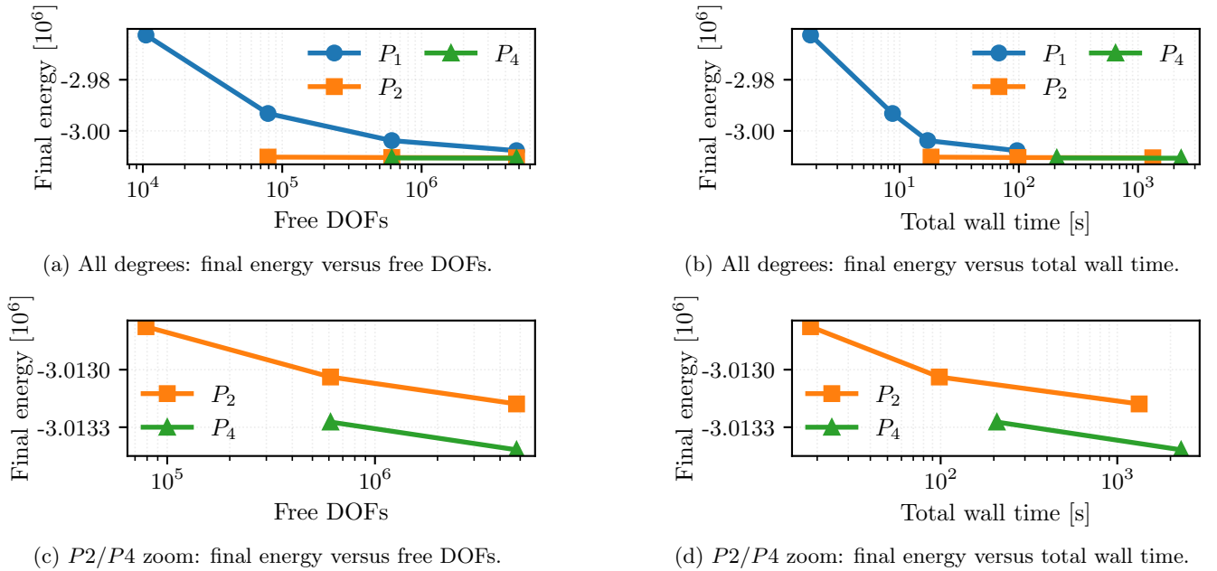
Figure 26: Corrected glued-bottom Plasticity3D degree-versus-resolution study at \lambda_{sr} = 1.55 . The top row shows the full P_1/P_2/P_4 comparison, while the bottom row zooms to P_2/P_4 so the near-overlap hidden by the coarse P_1 points becomes visible. The left column plots final values of equation (21) against free DOFs; the right column plots the same converged energies against end-to-end wall time. All timings use the same 32-rank configuration.
