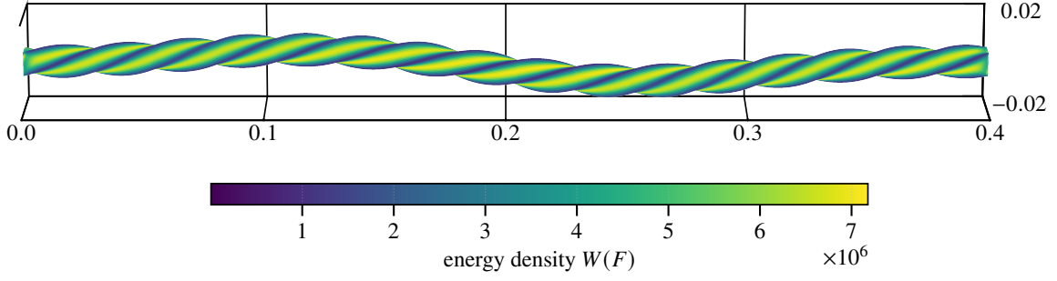
Figure 10: Representative finite-strain hyperelastic state, colored by the energy density in equation (11).
