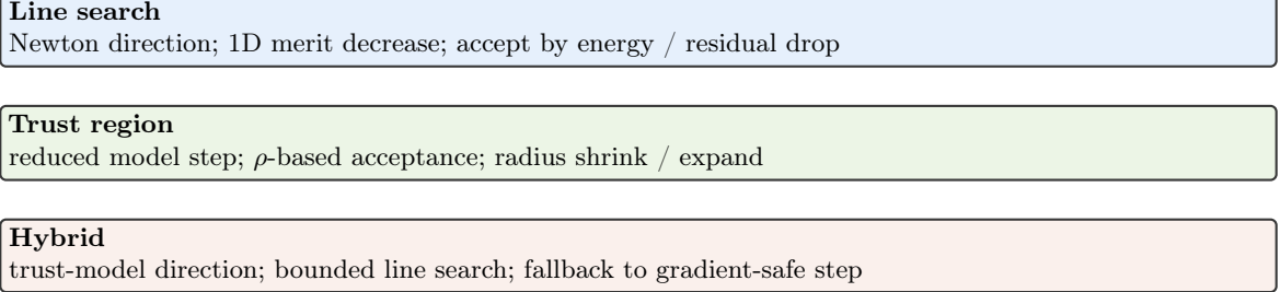
Figure 4: Globalization choices used across the benchmark suite, from pure line search to trust-region and hybrid strategies.
