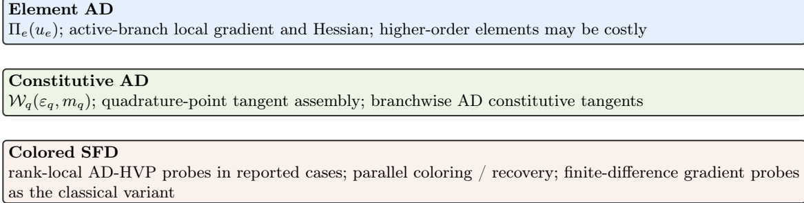
Figure 3: Second-order derivative modes exposed in the JAX+PETSc realization. The methodological choice is that the scalar energy or energy-density expression remains the defining mathematical object even when the tangent route changes from element AD to constitutive AD or colored sparse recovery.
