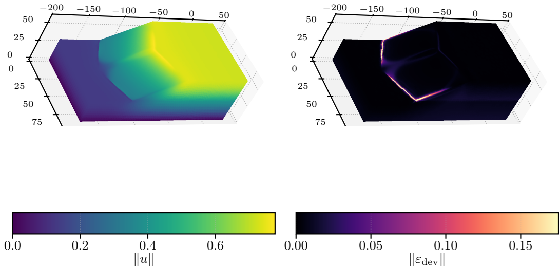
Figure 14: Bottom-clamped Plasticity3D representative endpoint at \lambda_{sr} = 1.55 : displacement magnitude and surface deviatoric strain for the P_4(L_2) run, both derived from the scalar surrogate in equation (22).
