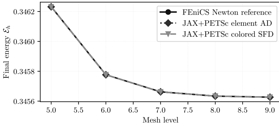
Figure 9: Final discrete energies associated with the stationary problem equation (11) across mesh levels. The element-AD and colored sparse-recovery JAX+PETSc routes agree with the FEniCS reference within about 1 \times 10^{-6} in final energy.
