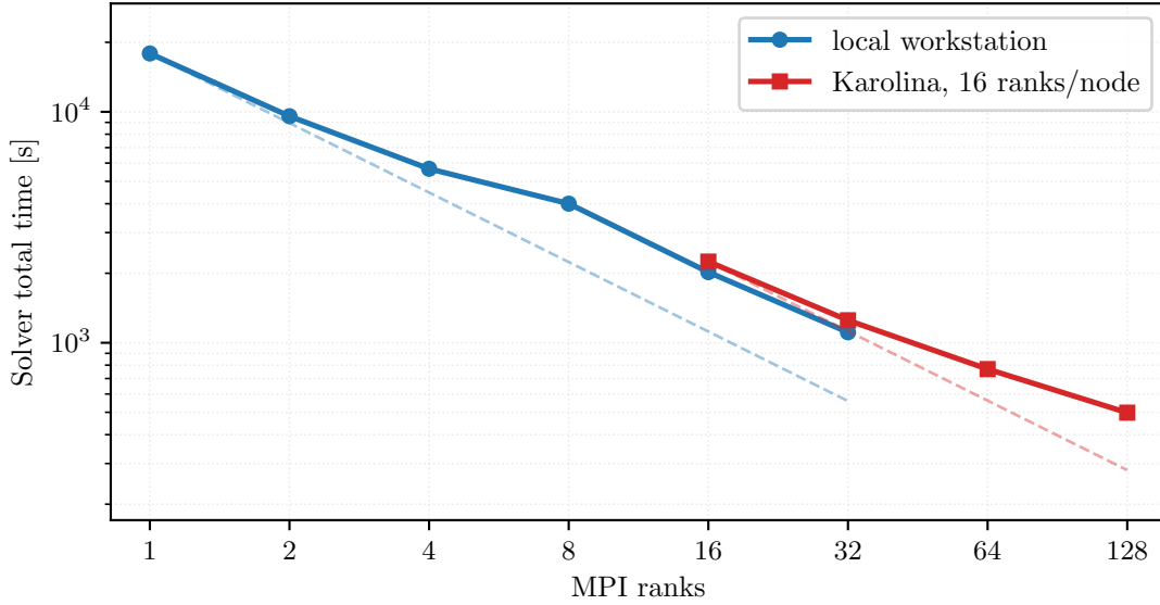
Figure 28: Workstation and Karolina converged scaling for the glued-bottom Plasticity3D P_4(L_2) case at \lambda_{sr} = 1.55 . Dashed references are ideal 1/r lines anchored separately to the first point of each platform.
