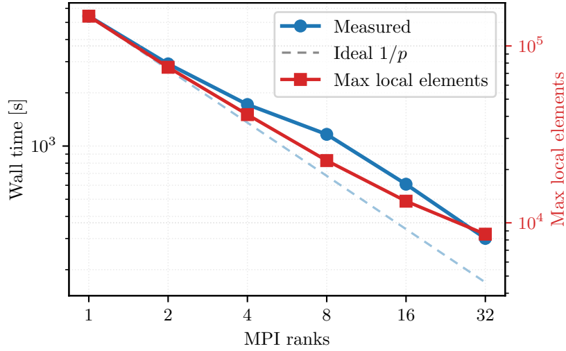
Figure 27: Historical strong scaling for the selected Plasticity3D stack: constitutive-AD local assembly with same-mesh PMG on P_4(L_2) at \lambda_{sr} = 1.0 . This is a separate timing study from the glued-bottom \lambda_{sr} = 1.55 results shown in figures 14, 15 and 26.
