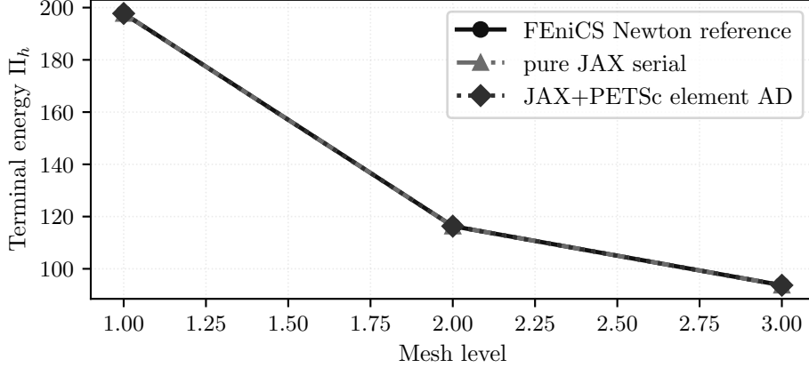
Figure 11: Final discrete energies along the stationary sequence equation (15) across the selected mesh hierarchy. The comparison records completion of the same 24-step schedule and comparable terminal energies; this figure does not assess trajectory-level agreement.
